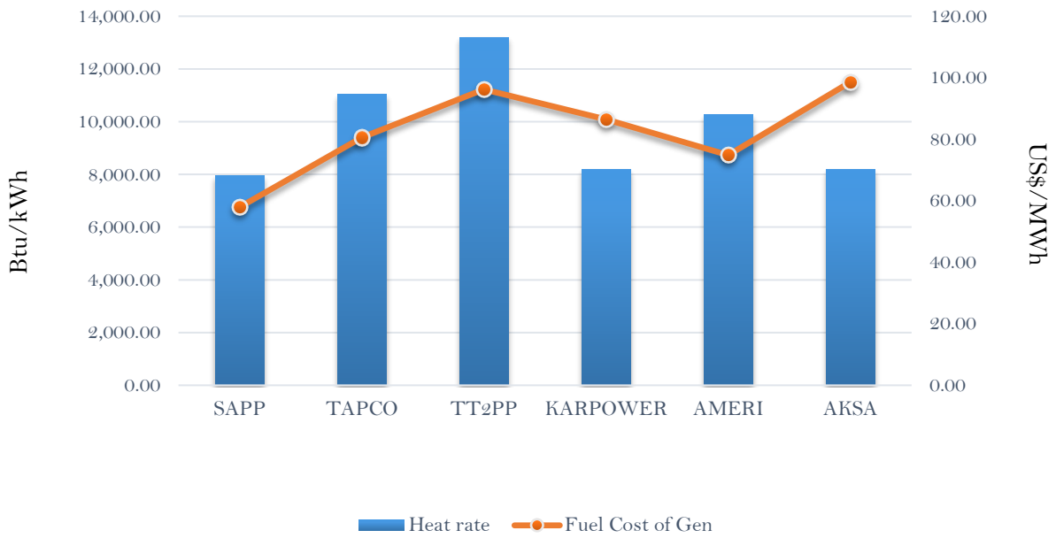
Efficiency and fuel cost of generation on the 6th February 2019
