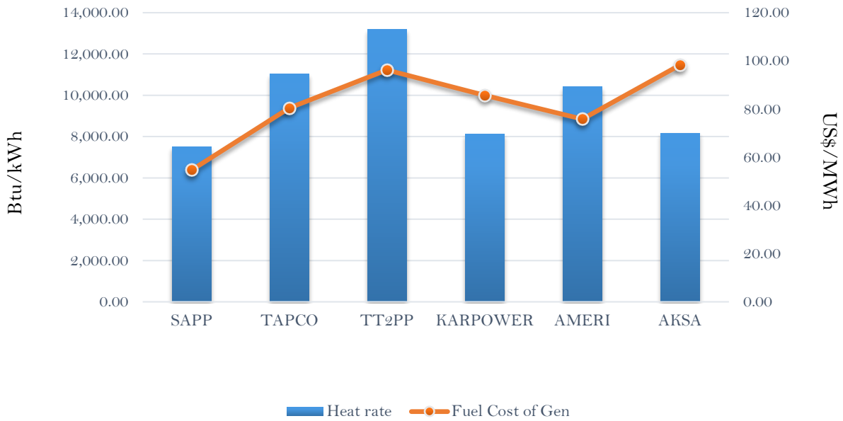
Efficiency and fuel cost of generation on the 2nd February 2019
