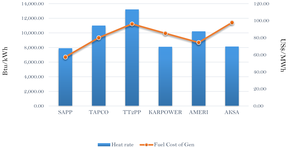
Efficiency and fuel cost of generation on the 4th February 2019
