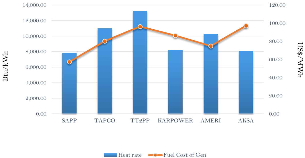
Efficiency and fuel cost of generation on the 2nd February 2019
