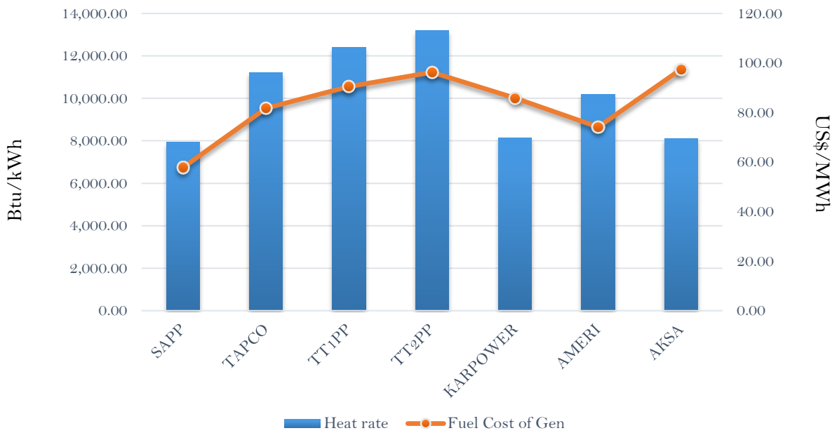
Efficiency and fuel cost of generation on the 11th February 2019
