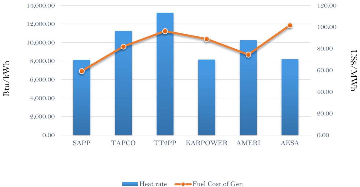
Efficiency and fuel cost of generation on the 13th February 2019
