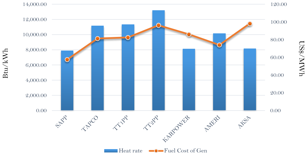
Efficiency and fuel cost of generation on the 11th February 2019
