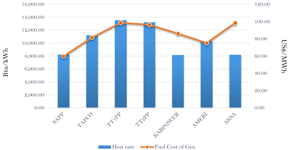
Efficiency and fuel cost of generation on the 9th February 2019
