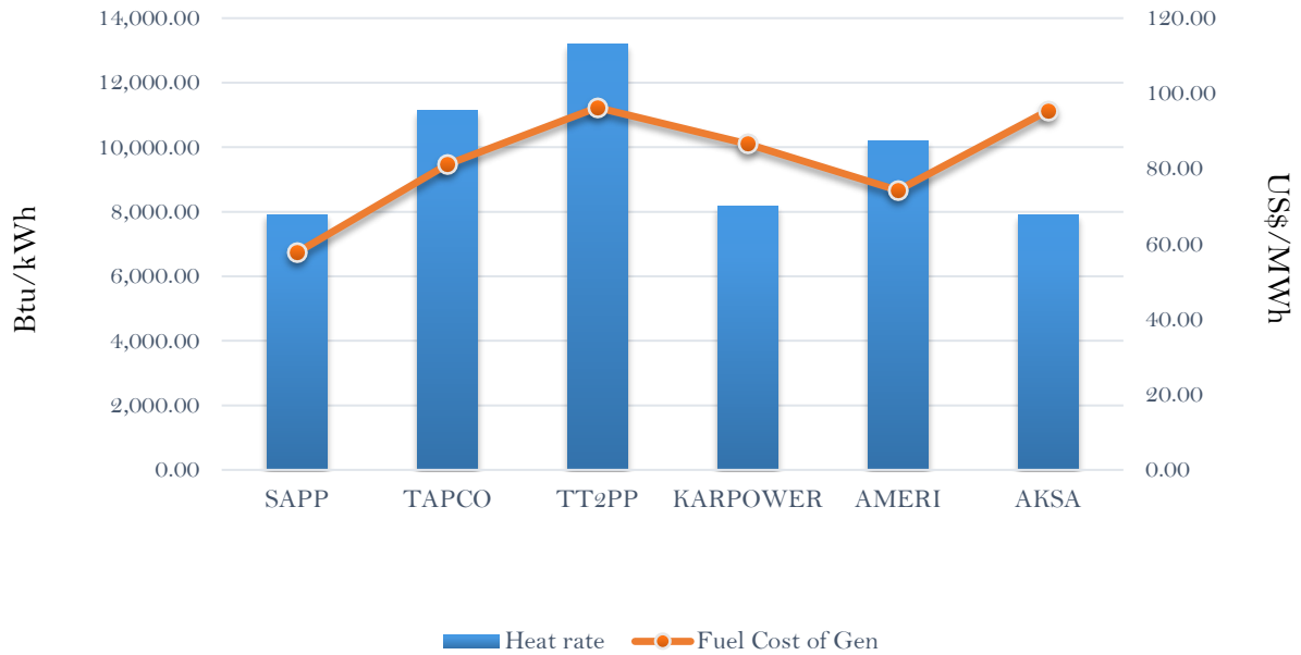
Efficiency and fuel cost of generation on the 9th February 2019
