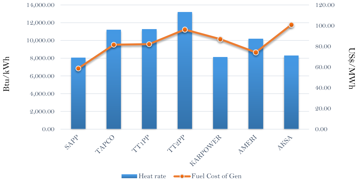
Efficiency and fuel cost of generation on the 13th February 2019
