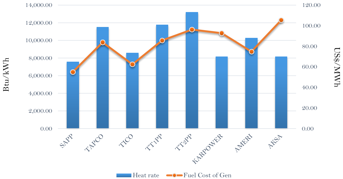
Efficiency and fuel cost of generation on the 20th February 2019
