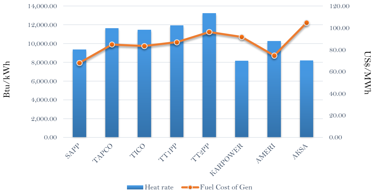
Efficiency and fuel cost of generation on the 18th February 2019
