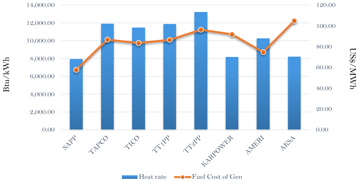
Efficiency and fuel cost of generation on the 20th February 2019
