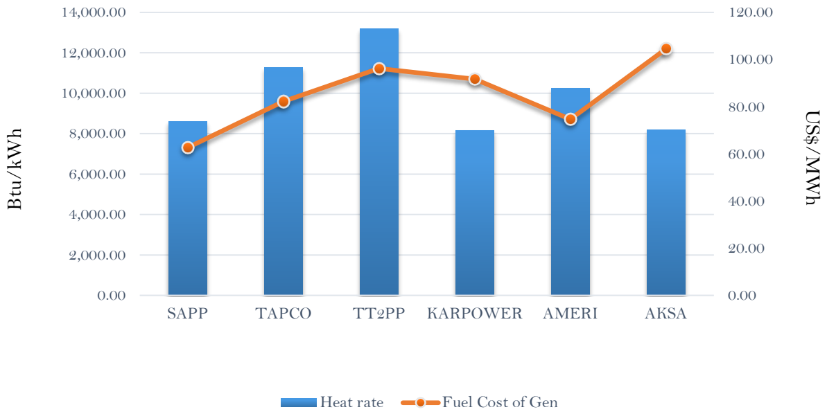
Efficiency and fuel cost of generation on the 16th February 2019
