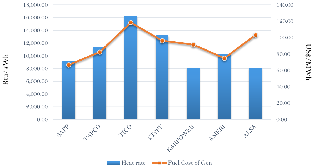
Efficiency and fuel cost of generation on the 16th February 2019
