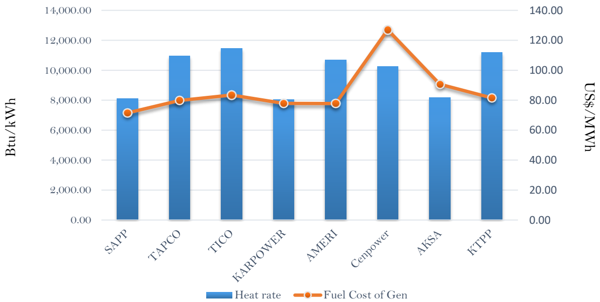
Efficiency and fuel cost of generation on the 4th January 2019
