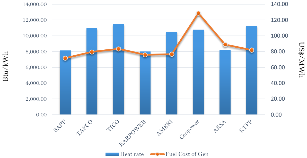
Efficiency and fuel cost of generation on the 3rd January 2019
