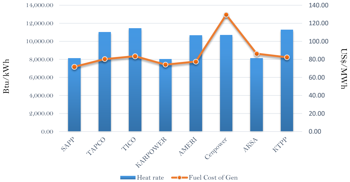
Efficiency and fuel cost of generation on the 2nd January 2019
