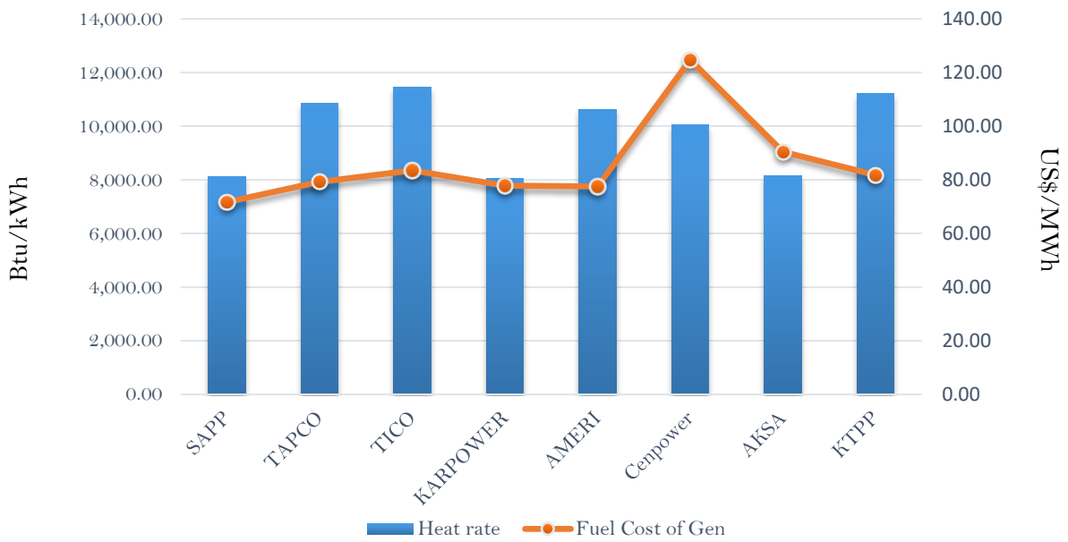
Efficiency and fuel cost of generation on the 6th January 2019
