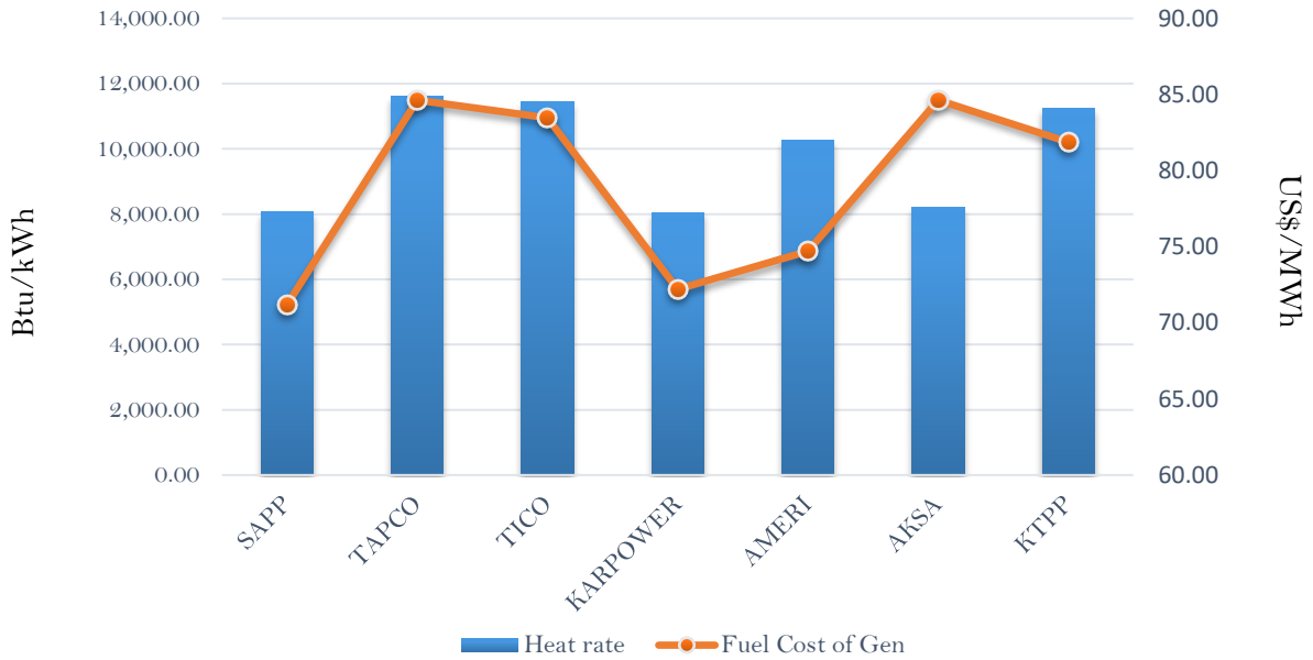
Efficiency and fuel cost of generation on the 2nd January 2019
