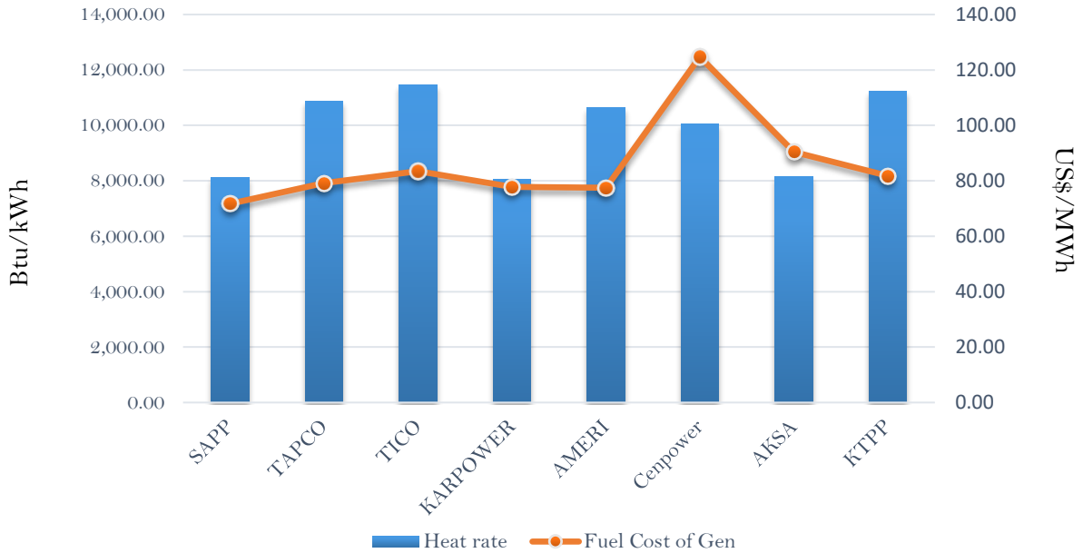
Efficiency and fuel cost of generation on the 5th January 2019
