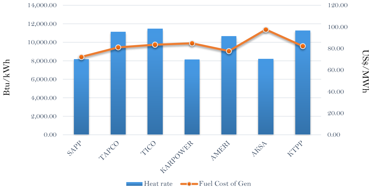
Efficiency and fuel cost of generation on the 11th January 2019
