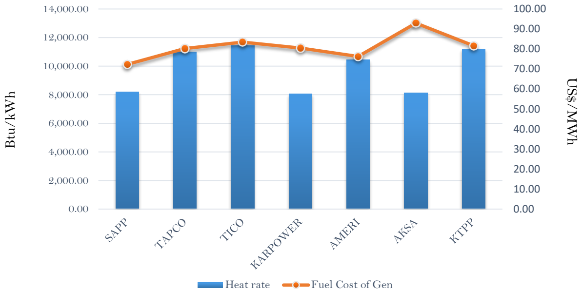
Efficiency and fuel cost of generation on the 8th January 2019
