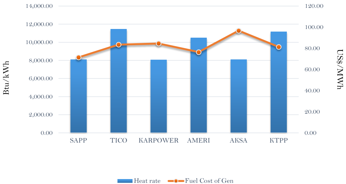
Efficiency and fuel cost of generation on the 9th January 2019
