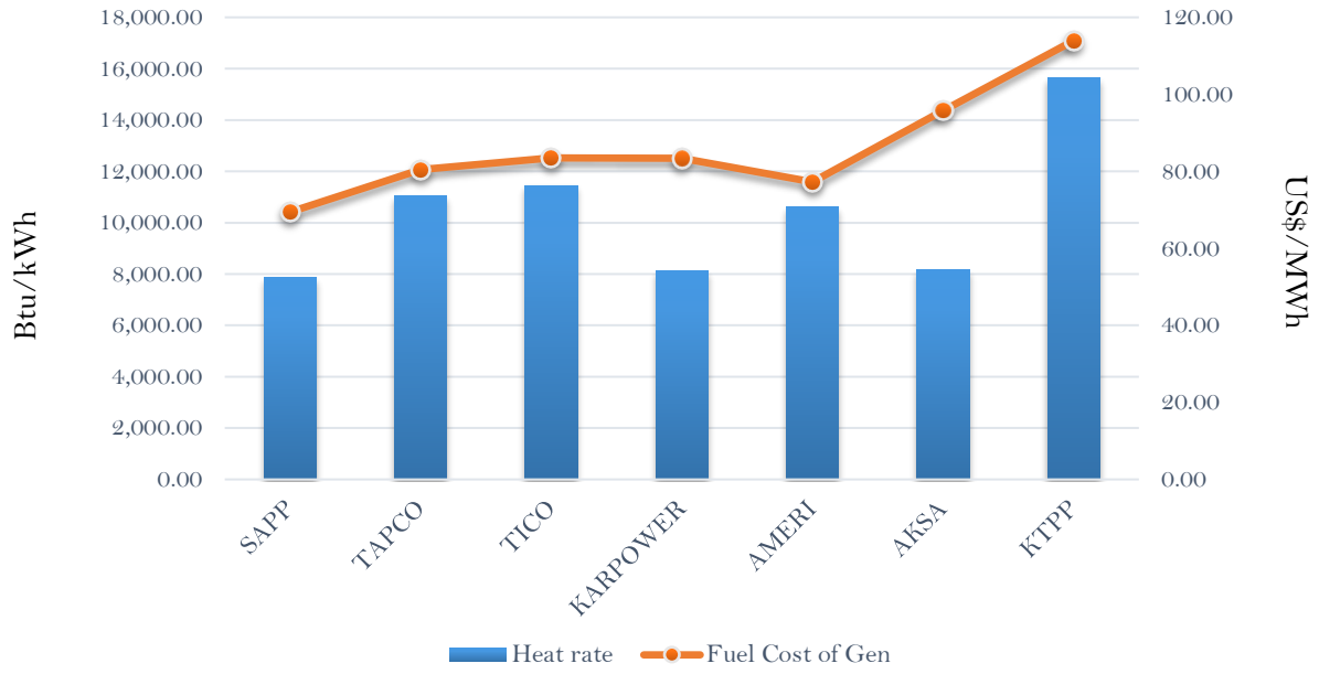
Efficiency and fuel cost of generation on the 13th January 2019
