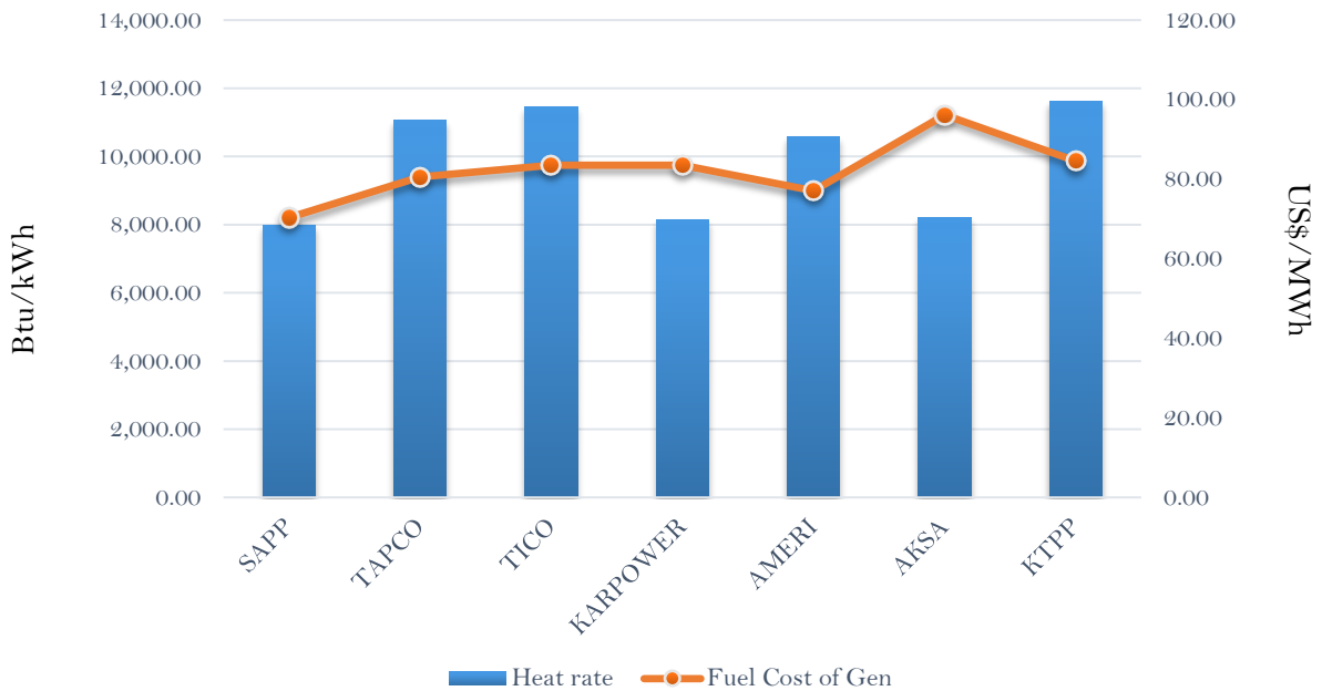
Efficiency and fuel cost of generation on the 11th January 2019
