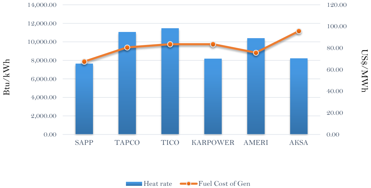
Efficiency and fuel cost of generation on the 16th January 2019
