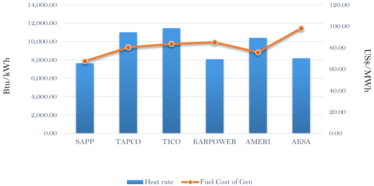
Efficiency and fuel cost of generation on the 20th January 2019
