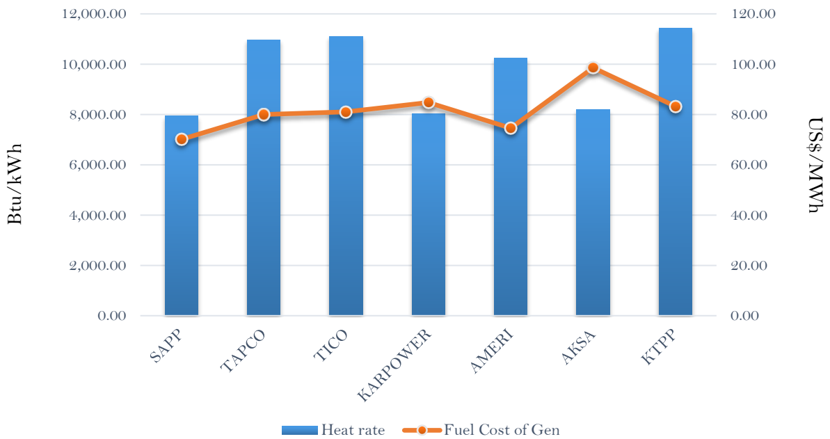
Efficiency and fuel cost of generation on the 20th January 2019
