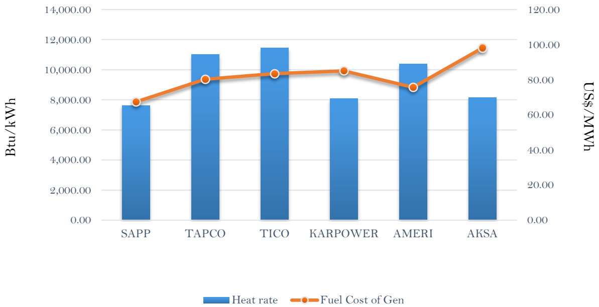
Efficiency and fuel cost of generation on the 18th January 2019
