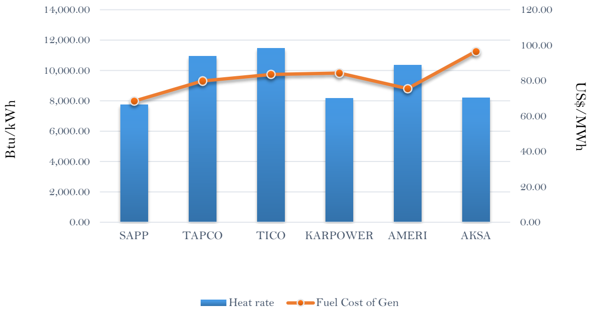
Efficiency and fuel cost of generation on the 16th January 2019
