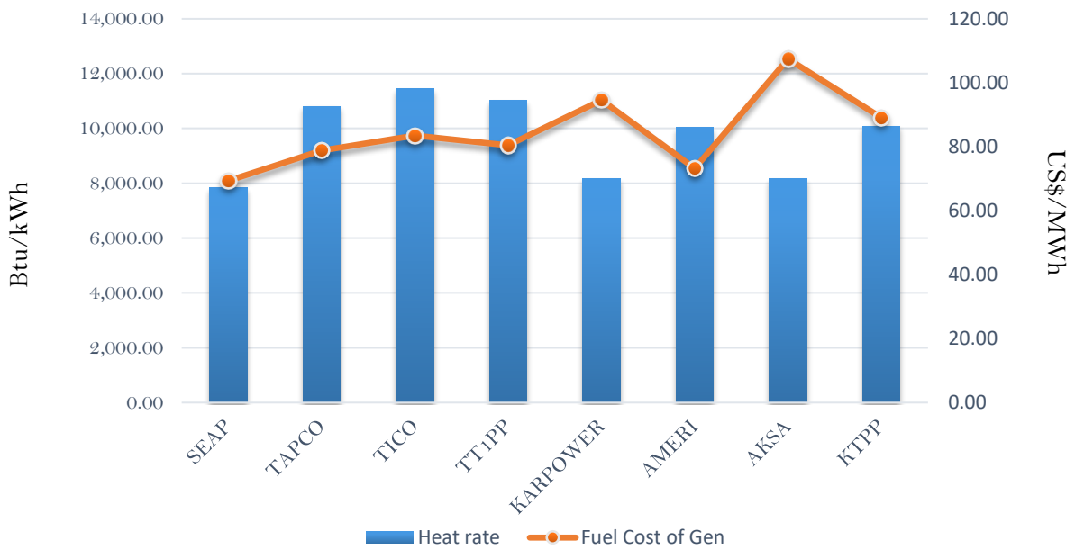
Efficiency and fuel cost of generation on the 11th November 2018
