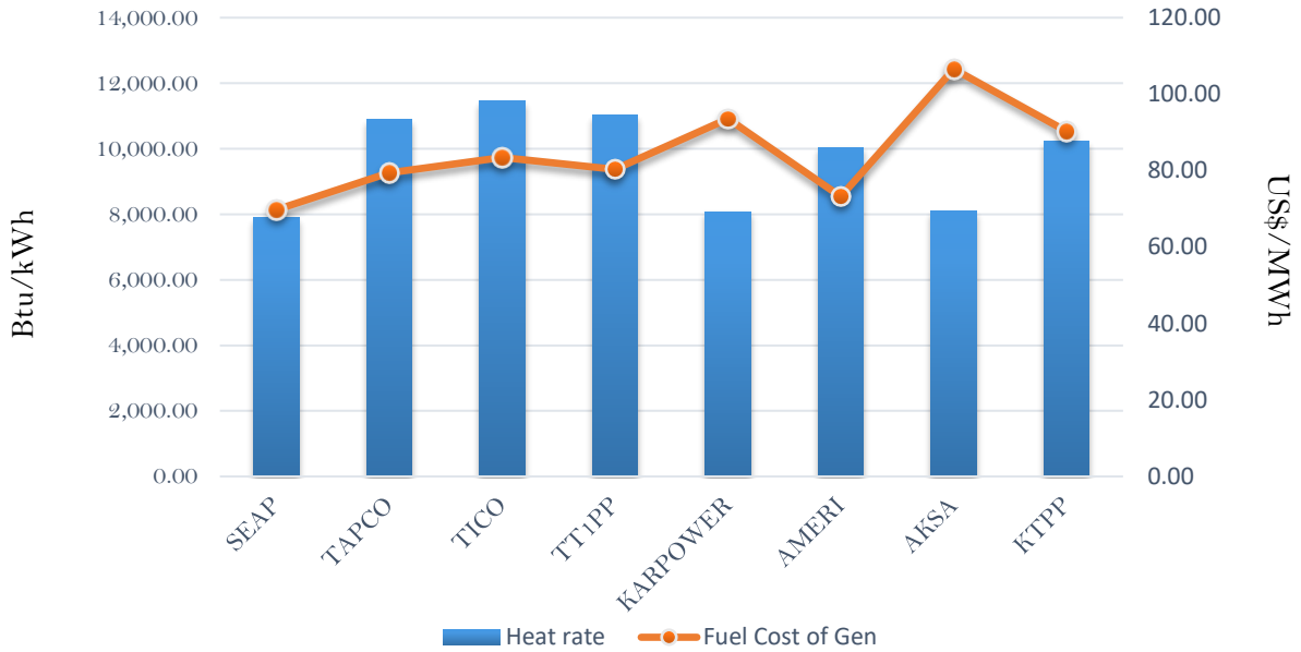
Efficiency and fuel cost of generation on the 10th November 2018
