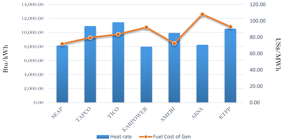
Efficiency and fuel cost of generation on the 9th November 2018
