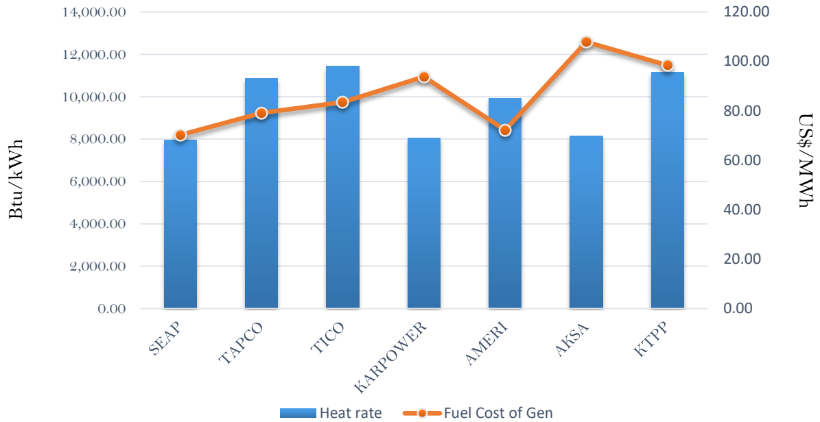
Efficiency and fuel cost of generation on the 8th November 2018
