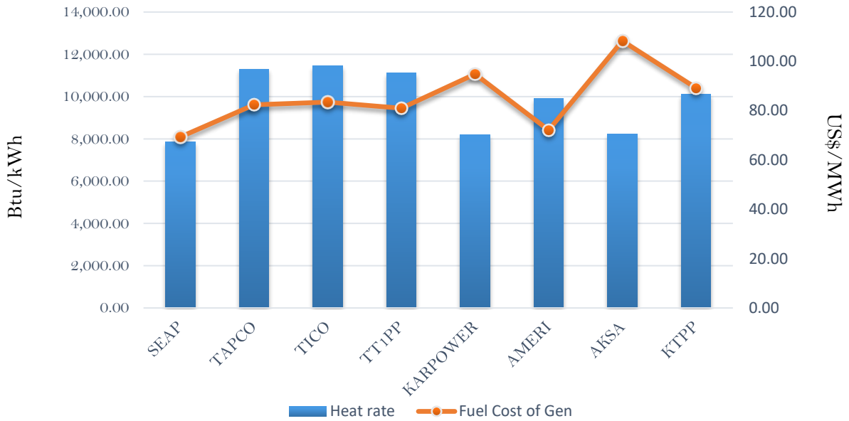
Efficiency and fuel cost of generation on the 12th November 2018
