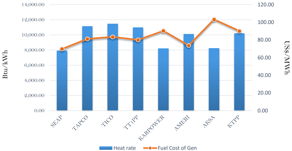
Efficiency and fuel cost of generation on the 13th November 2018
