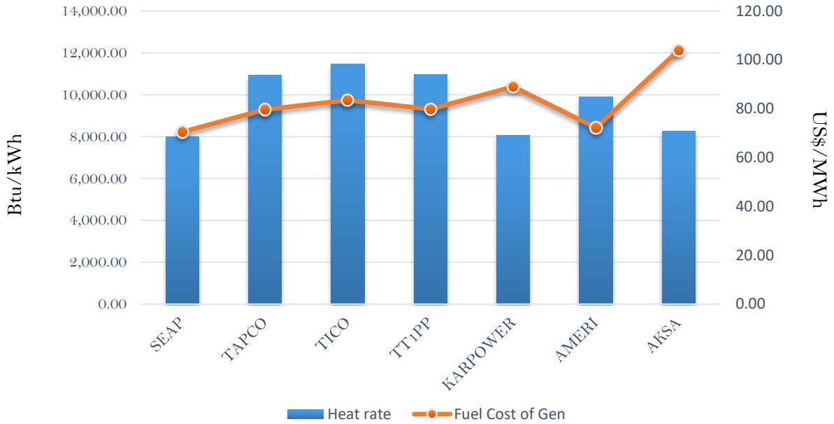
Efficiency and fuel cost of generation on the 16th November 2018
