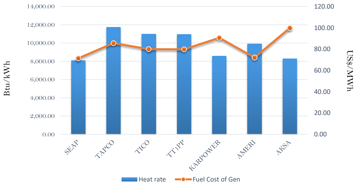
Efficiency and fuel cost of generation on the 20th November 2018
