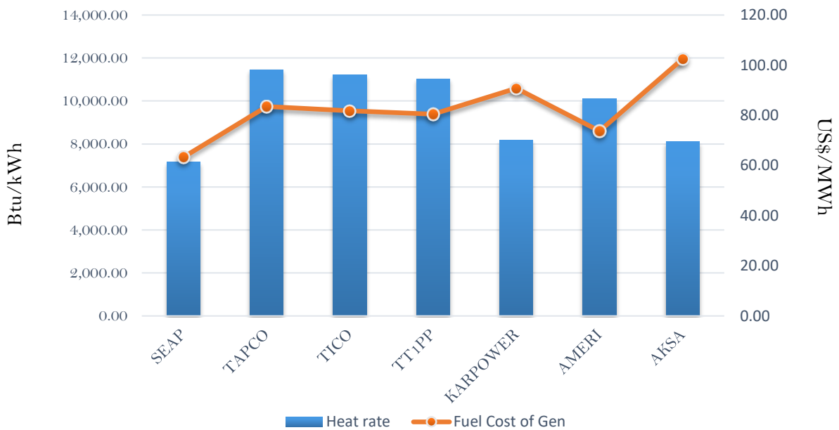
Efficiency and fuel cost of generation on the 16th November 2018
