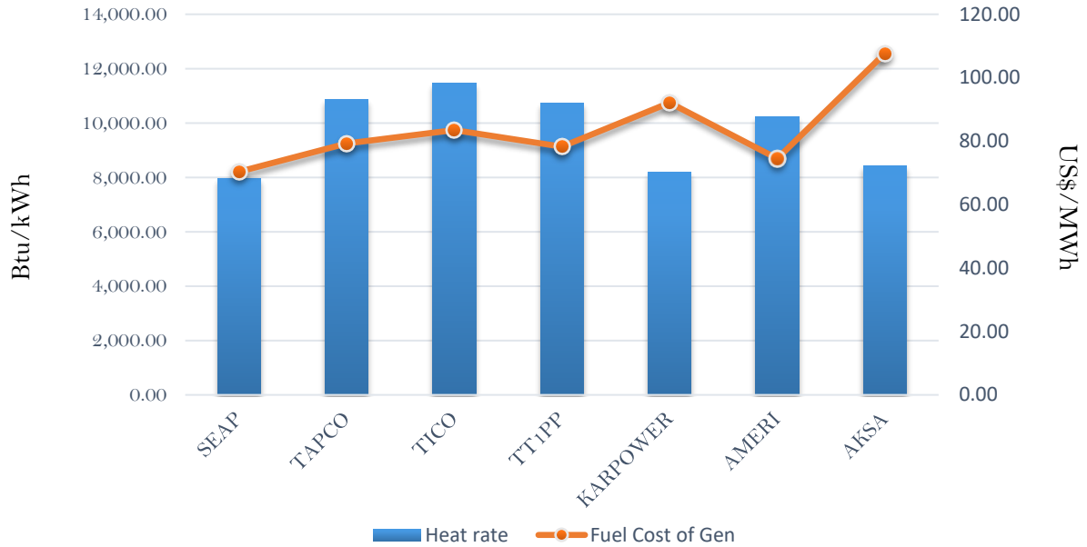
Efficiency and fuel cost of generation on the 19th November 2018
