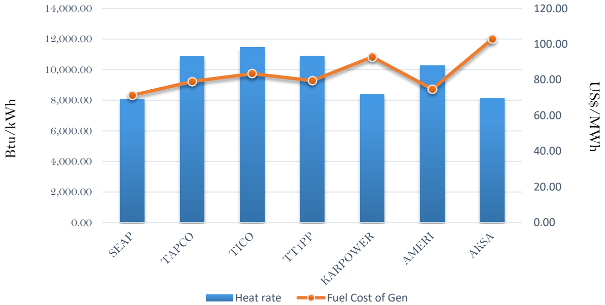
Efficiency and fuel cost of generation on the 17th November 2018
