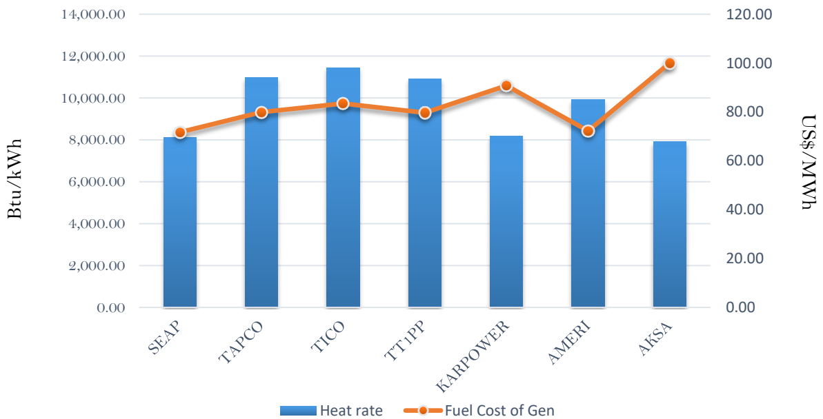
Efficiency and fuel cost of generation on the 18th November 2018
