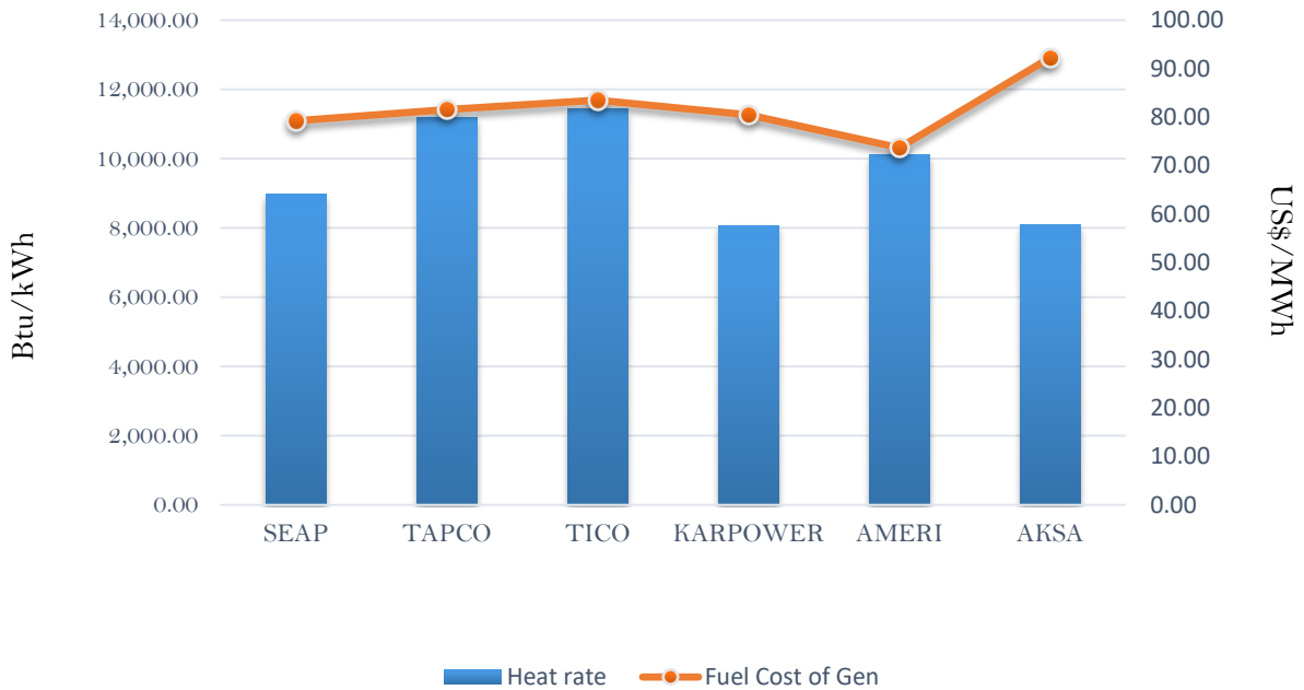
Efficiency and fuel cost of generation on the 29th November 2018
