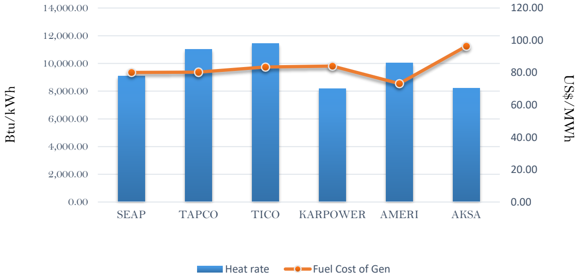
Efficiency and fuel cost of generation on the 26th November 2018
