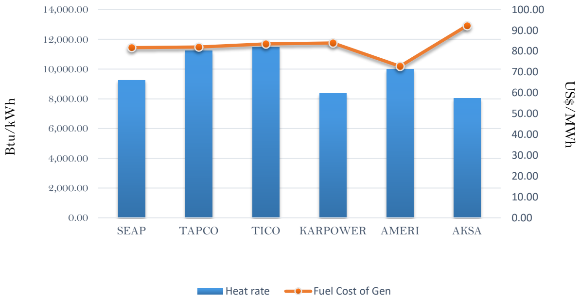
Efficiency and fuel cost of generation on the 25th November 2018
