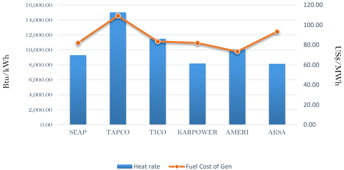
Efficiency and fuel cost of generation on the 24th November 2018
