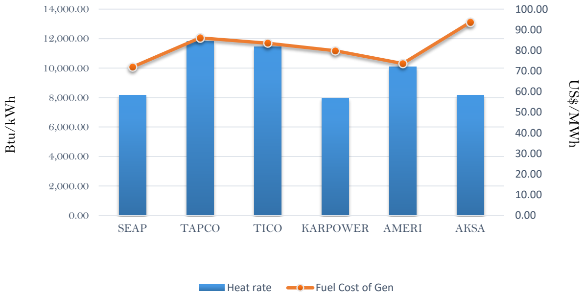
Efficiency and fuel cost of generation on the 23rd November 2018
