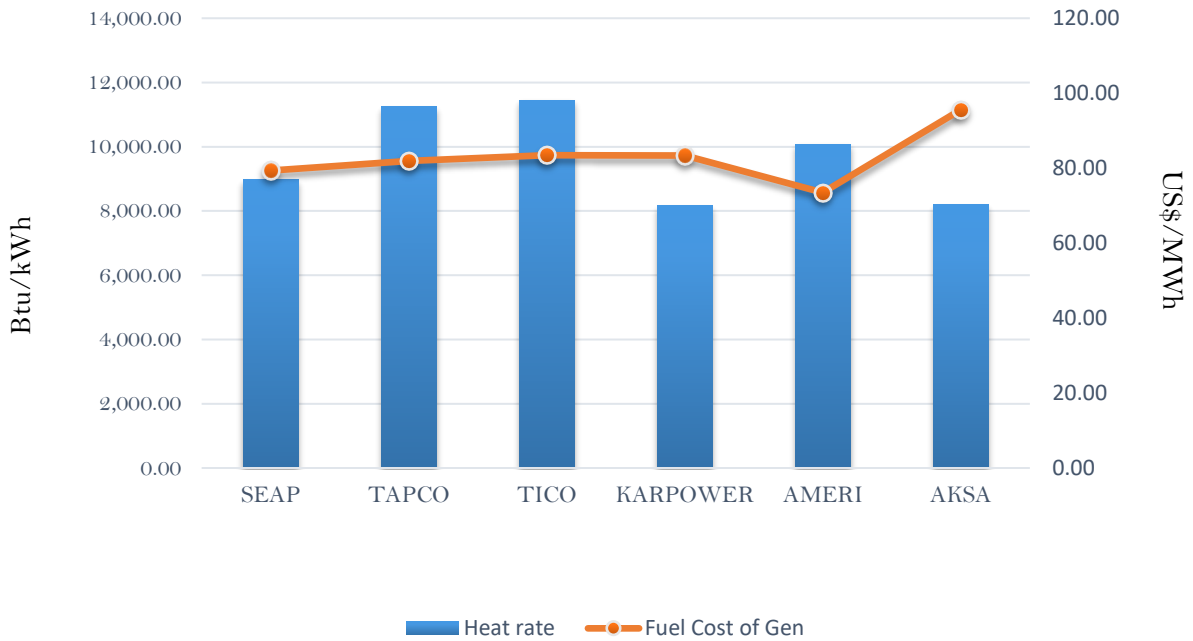
Efficiency and fuel cost of generation on the 27th November 2018
