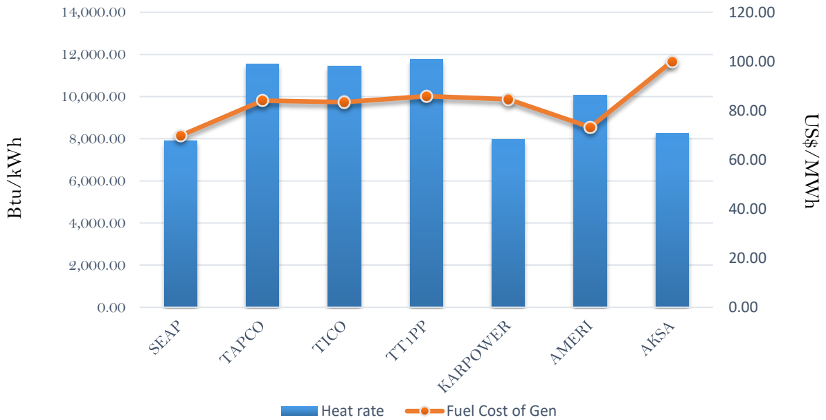
Efficiency and fuel cost of generation on the 22nd November 2018
