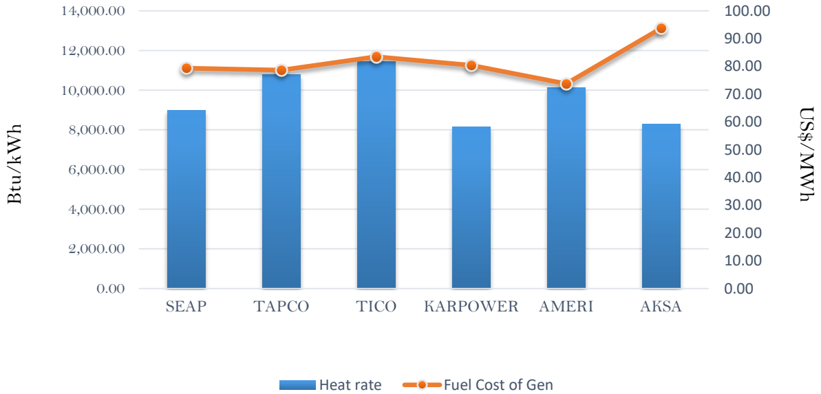
Efficiency and fuel cost of generation on the 28th November 2018
