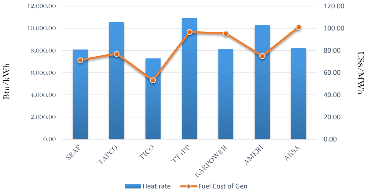
Efficiency and fuel cost of generation on 6th September 2018
