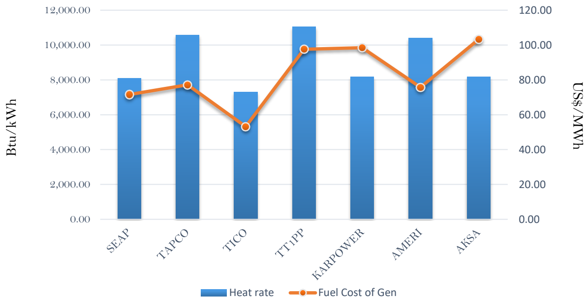
Efficiency and fuel cost of generation on 2nd September 2018
