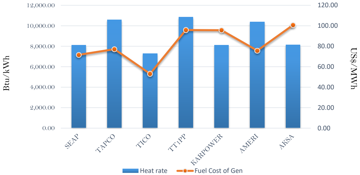
Efficiency and fuel cost of generation on 5th September 2018
