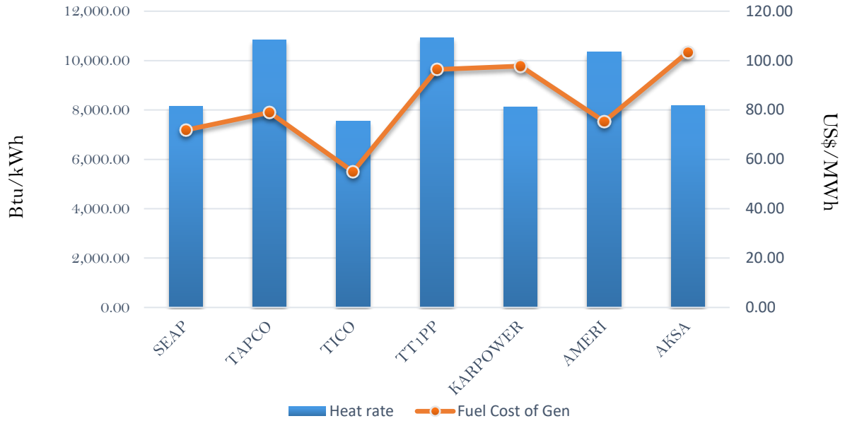
Efficiency and fuel cost of generation on 1st September 2018
