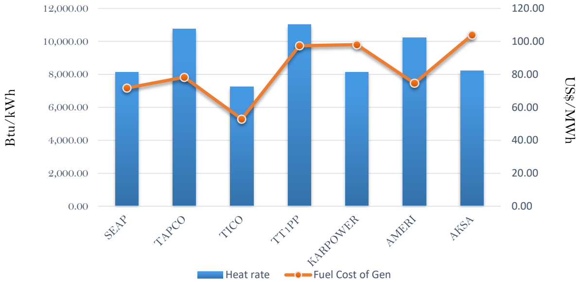
Efficiency and fuel cost of generation on 15th September 2018
