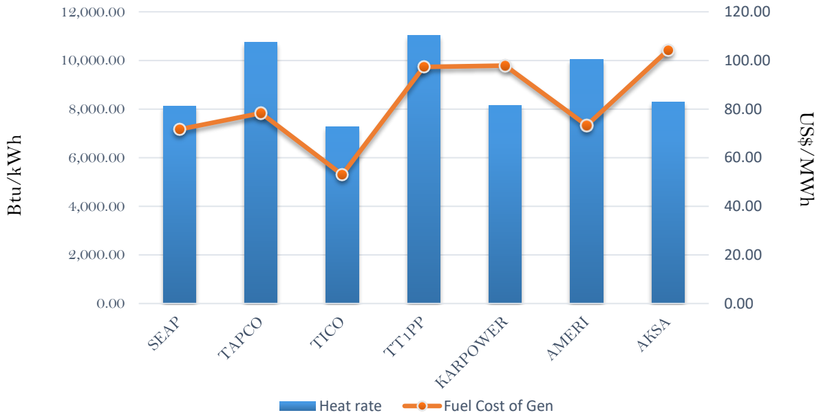
Efficiency and fuel cost of generation on 17th September 2018
