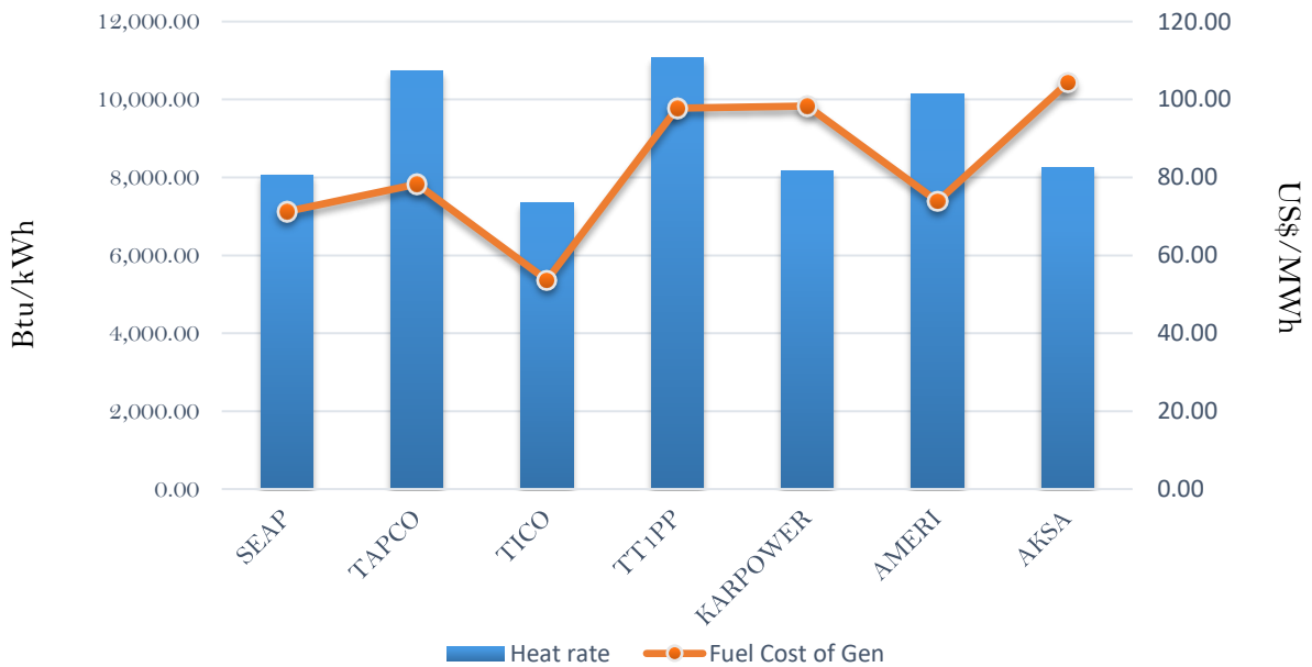
Efficiency and fuel cost of generation on 16th September 2018
