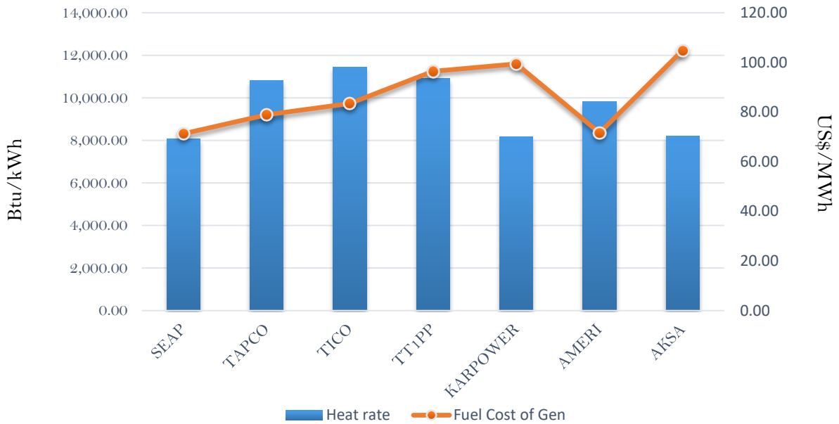
Efficiency and fuel cost of generation on 20th eptmber 2018
