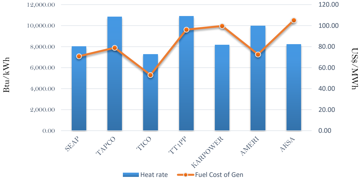
Efficiency and fuel cost of generation on 19th September 2018
