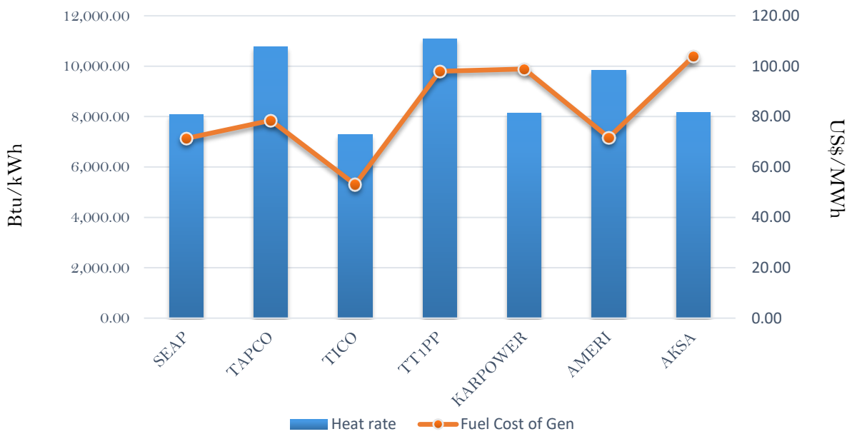
Efficiency and fuel cost of generation on 18th September 2018
