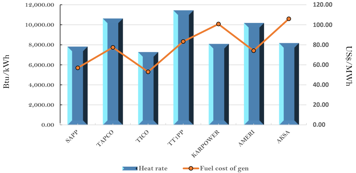
Efficiency and fuel cost of generation on the 18th April 2018
