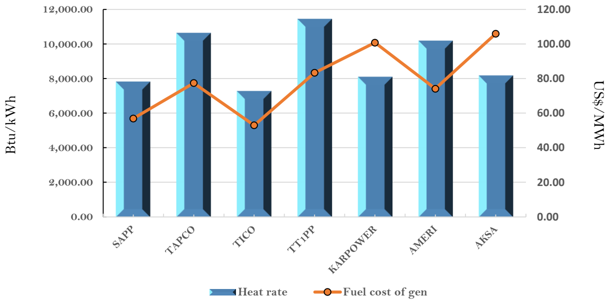
Efficiency and fuel cost of generation on the 20th April 2018
