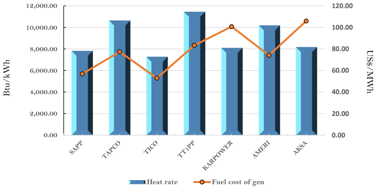
Efficiency and fuel cost of generation on the 16th April 2018
