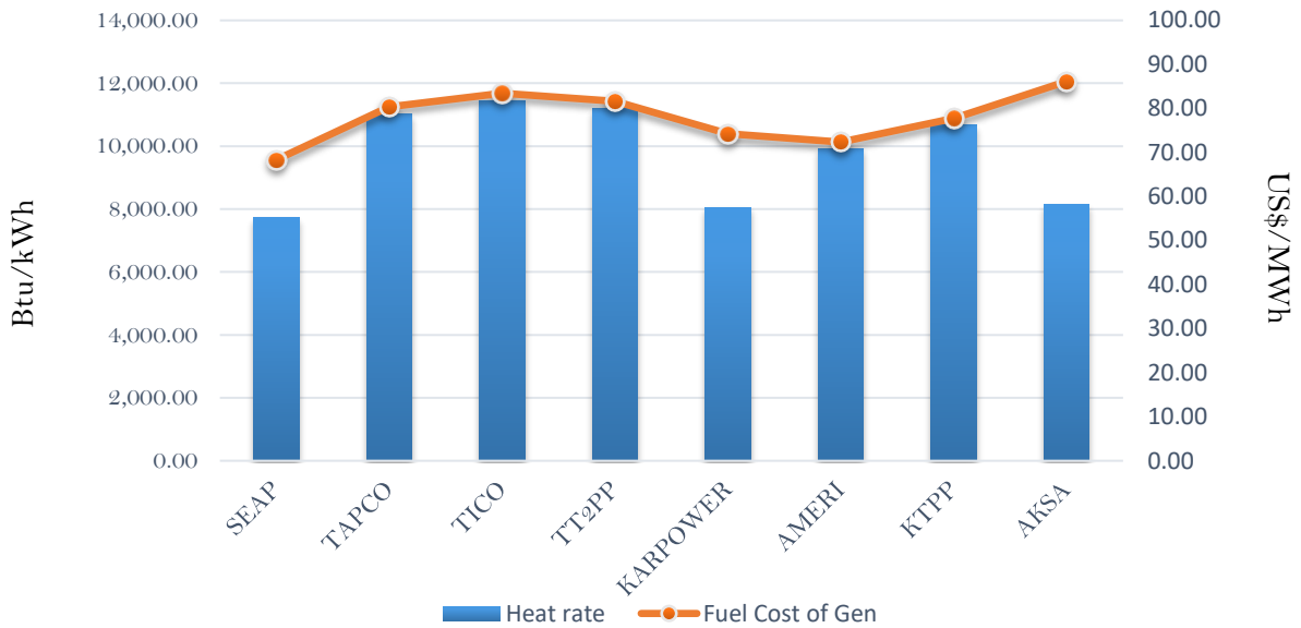
Efficiency and fuel cost of generation on the 26th December 2018
