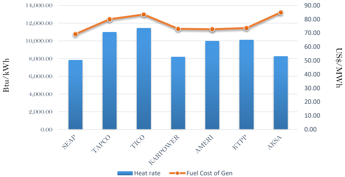
Efficiency and fuel cost of generation on the 29th December 2018
