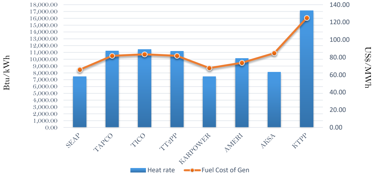
Efficiency and fuel cost of generation on the 22nd December 2018
