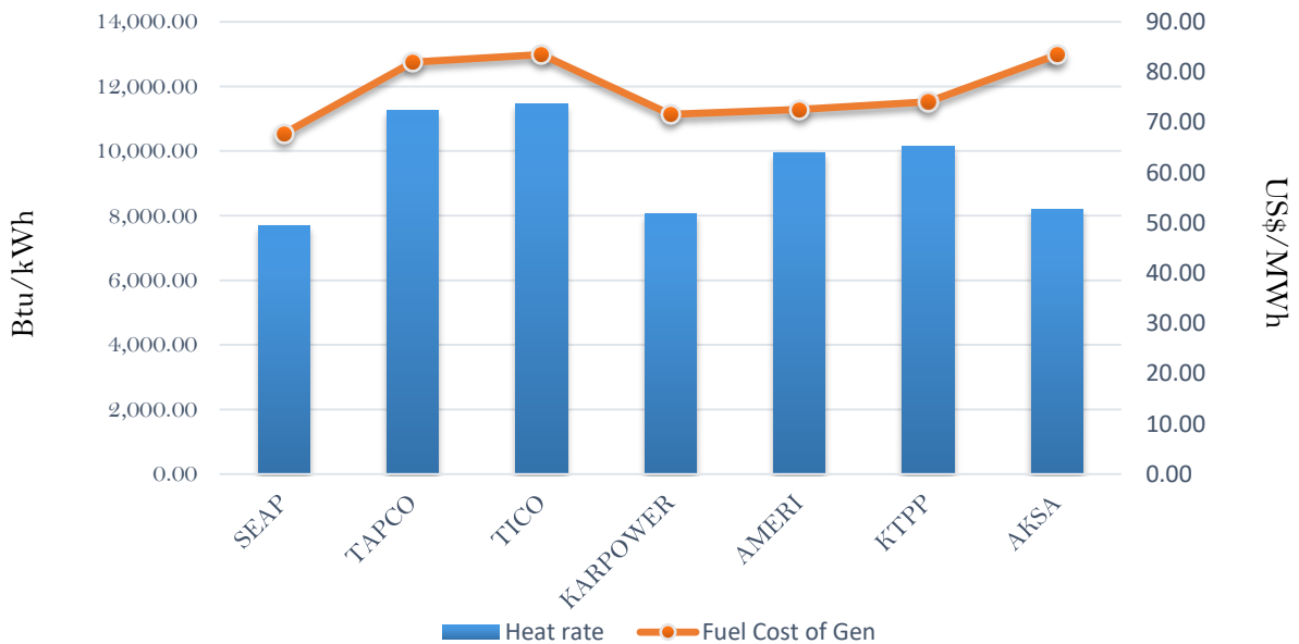
Efficiency and fuel cost of generation on the 27th December 2018
