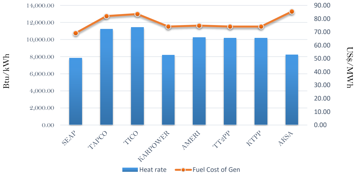
Efficiency and fuel cost of generation on the 31st December 2018
