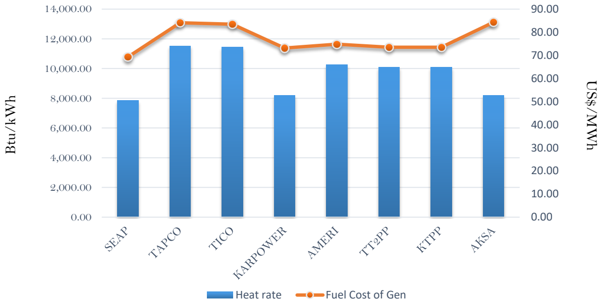
Efficiency and fuel cost of generation on the 30th December 2018
