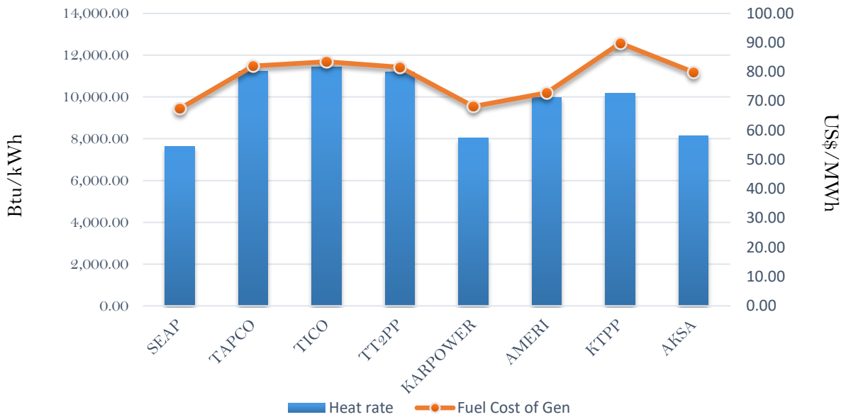
Efficiency and fuel cost of generation on the 24th December 2018
