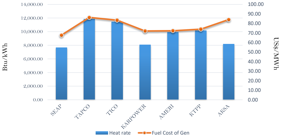
Efficiency and fuel cost of generation on the 28th December 2018
