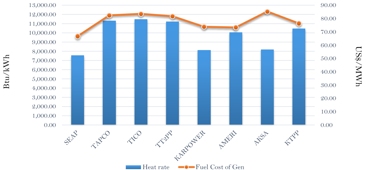
Efficiency and fuel cost of generation on the 23rd December 2018
