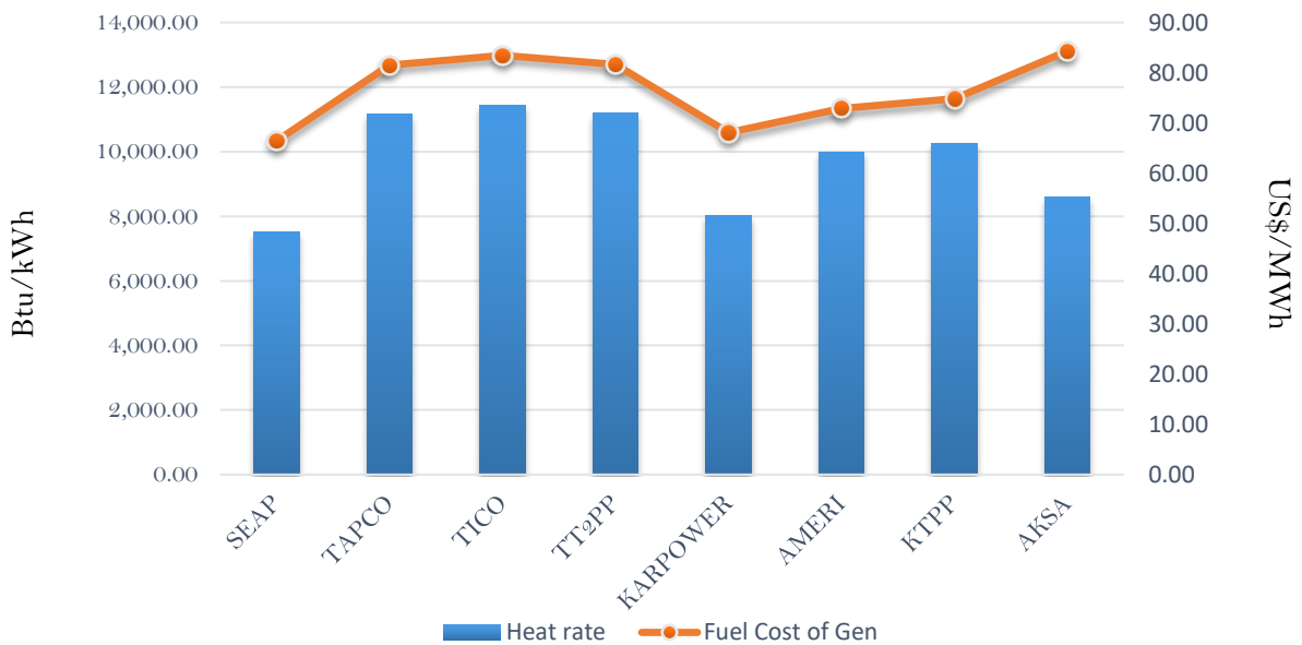
Efficiency and fuel cost of generation on the 25th December 2018
