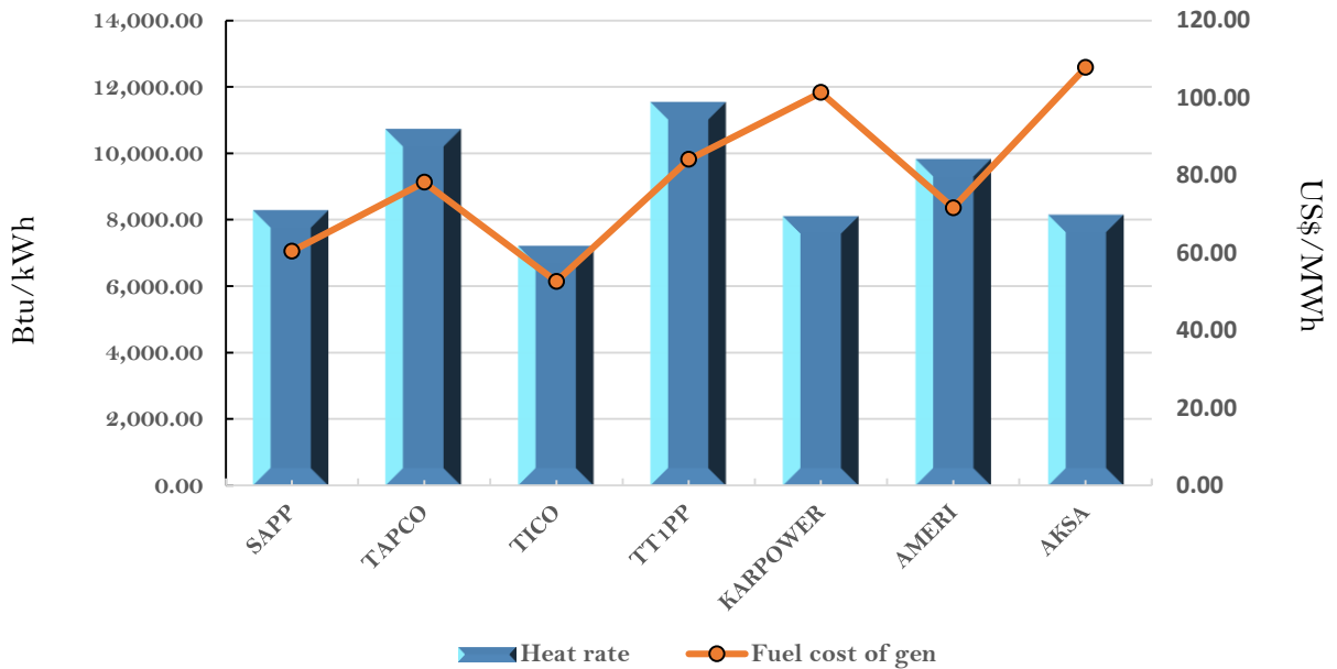
Efficiency and fuel cost of generation on the 27th April 2018
