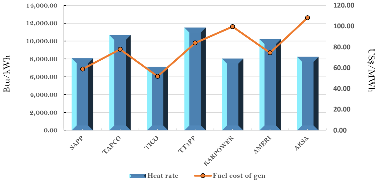
Efficiency and fuel cost of generation on the 23rd April 2018
