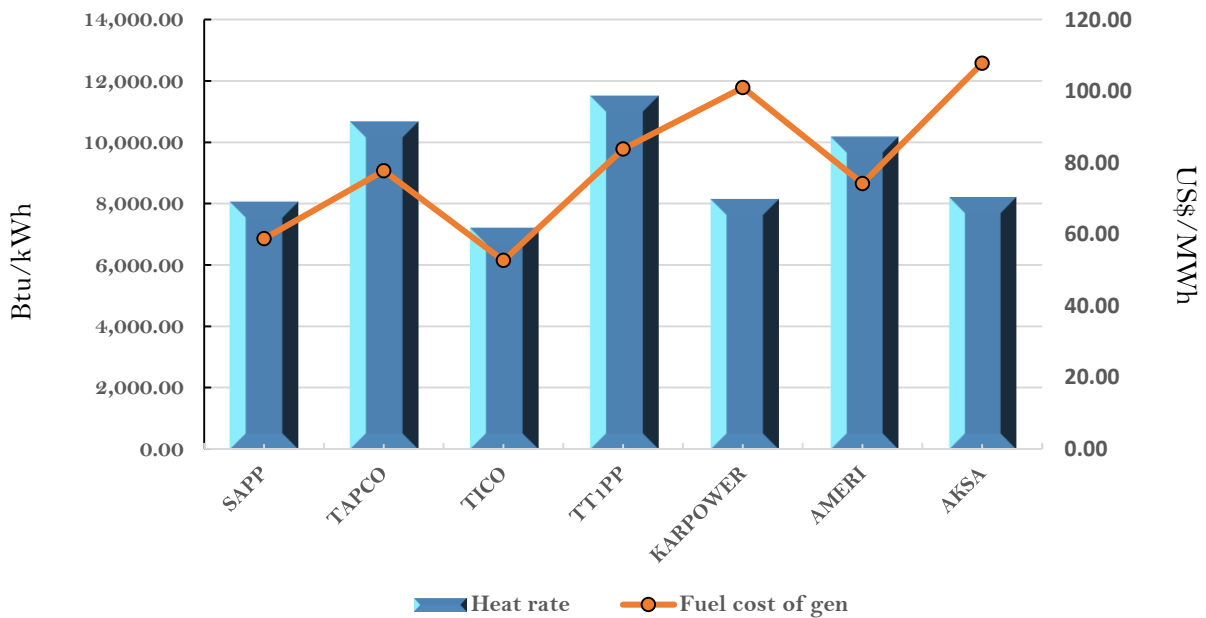
Efficiency and fuel cost of generation on the 23rd April 2018
