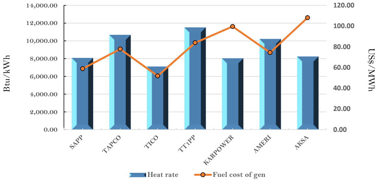
Efficiency and fuel cost of generation on the 22nd April 2018
