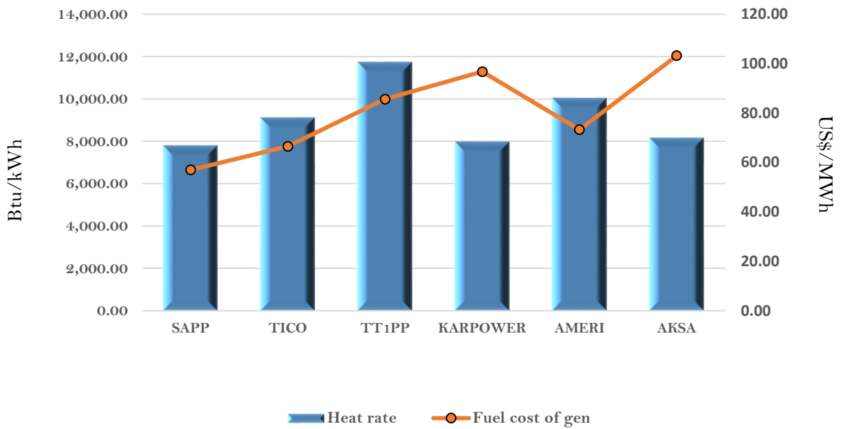
Efficiency and fuel cost of generation on the 9th April 2018
