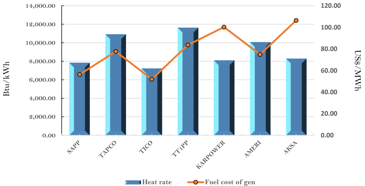
Efficiency and fuel cost of generation on the 13th April 2018
