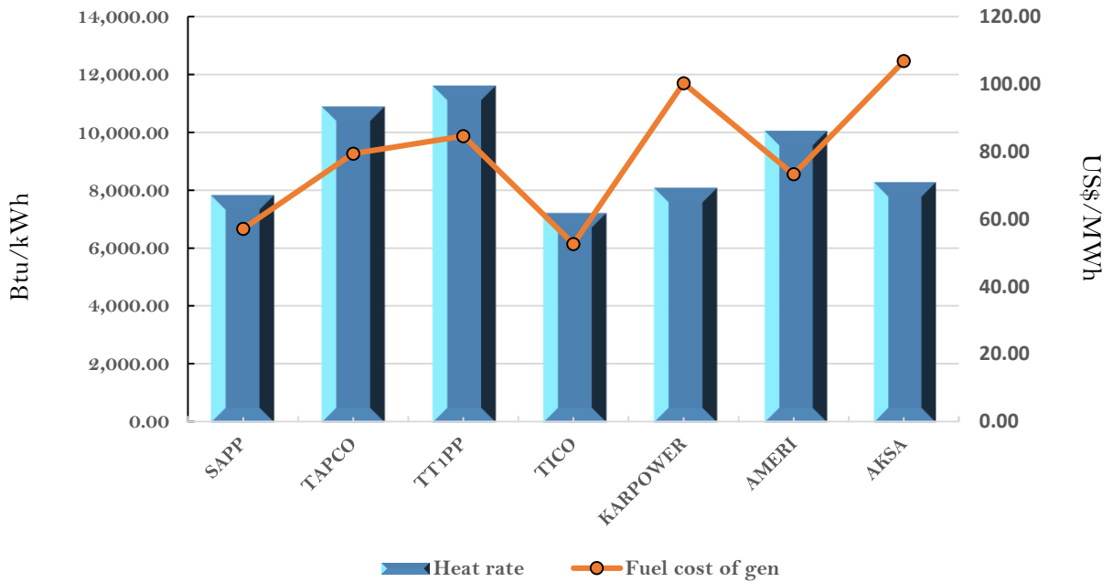
Efficiency and fuel cost of generation on the 11th April 2018
