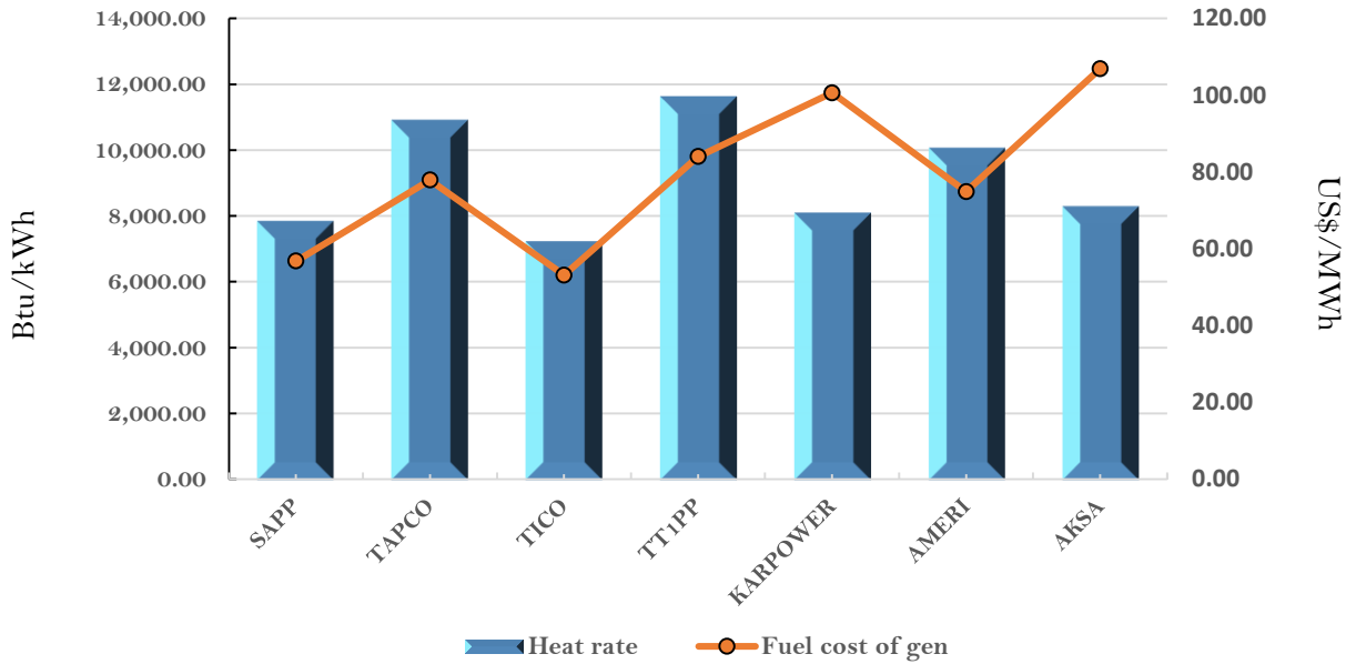
Efficiency and fuel cost of generation on the 13th April 2018
