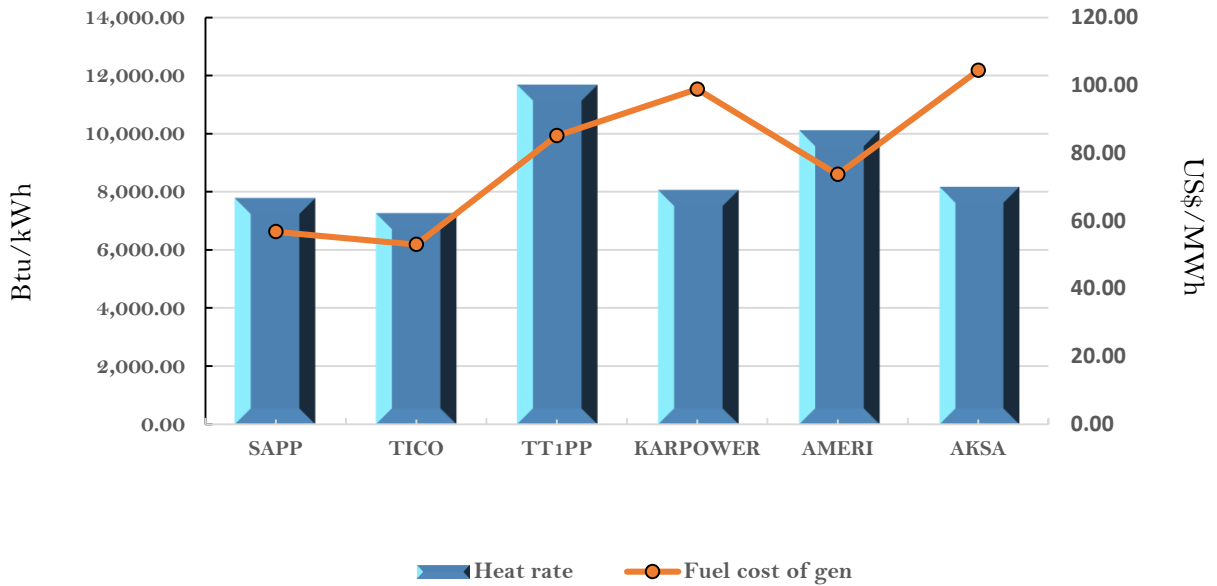
Efficiency and fuel cost of generation on the 11th April 2018
