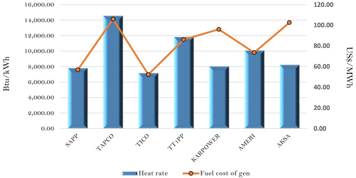
Efficiency and fuel cost of generation on the 9th April 2018
