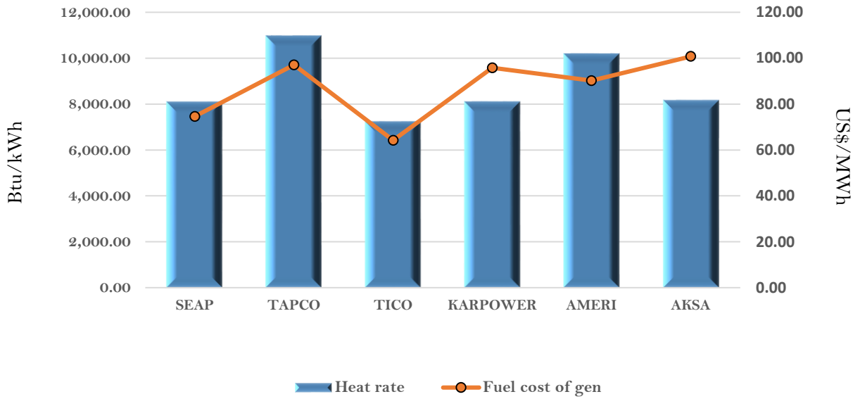
Efficiency and fuel cost of generation on the 12th March 2018
