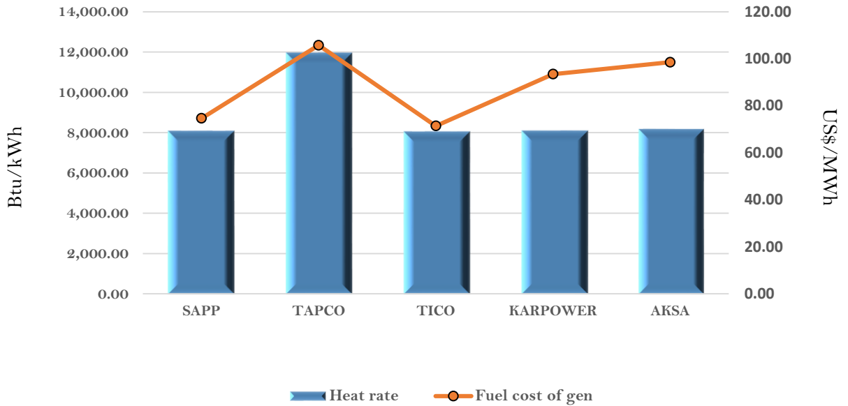
Efficiency and fuel cost of generation on the 8th March 2018
