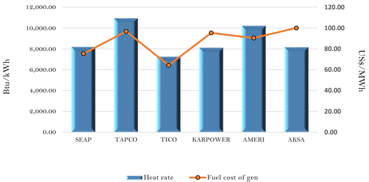
Efficiency and fuel cost of generation on the 13th March 2018
