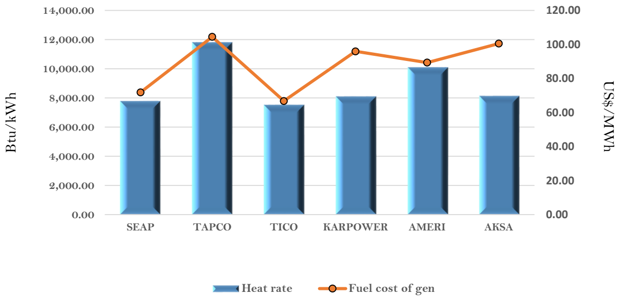
Efficiency and fuel cost of generation on the 9th March 2018
