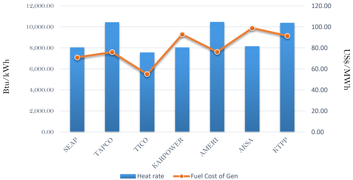
Efficiency and fuel cost of generation on the 20th August 2018
