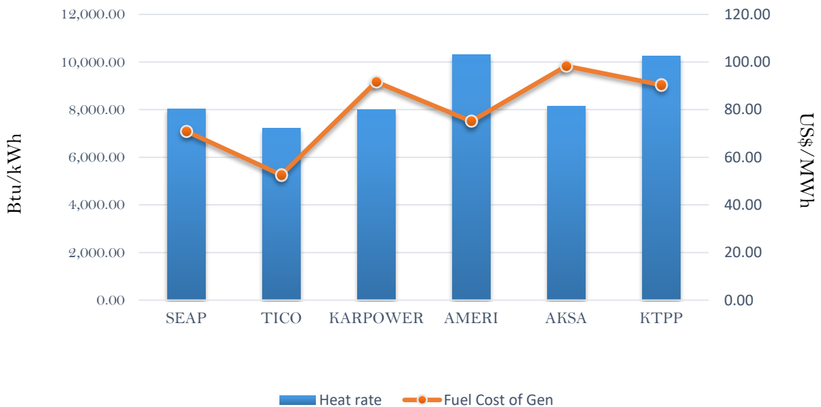
Efficiency and fuel cost of generation on the 18th August 2018
