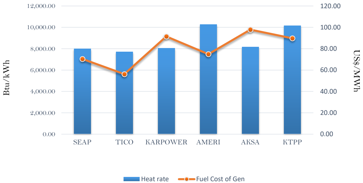
Efficiency and fuel cost of generation on the 16th August 2018
