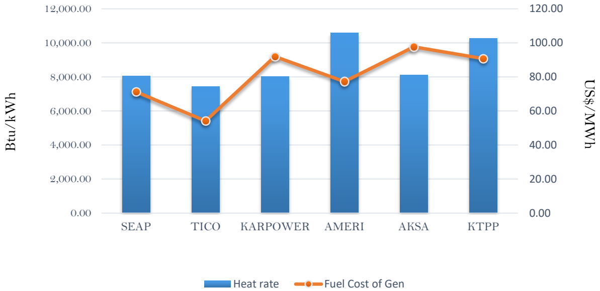
Efficiency and fuel cost of generation on the 19th August 2018
