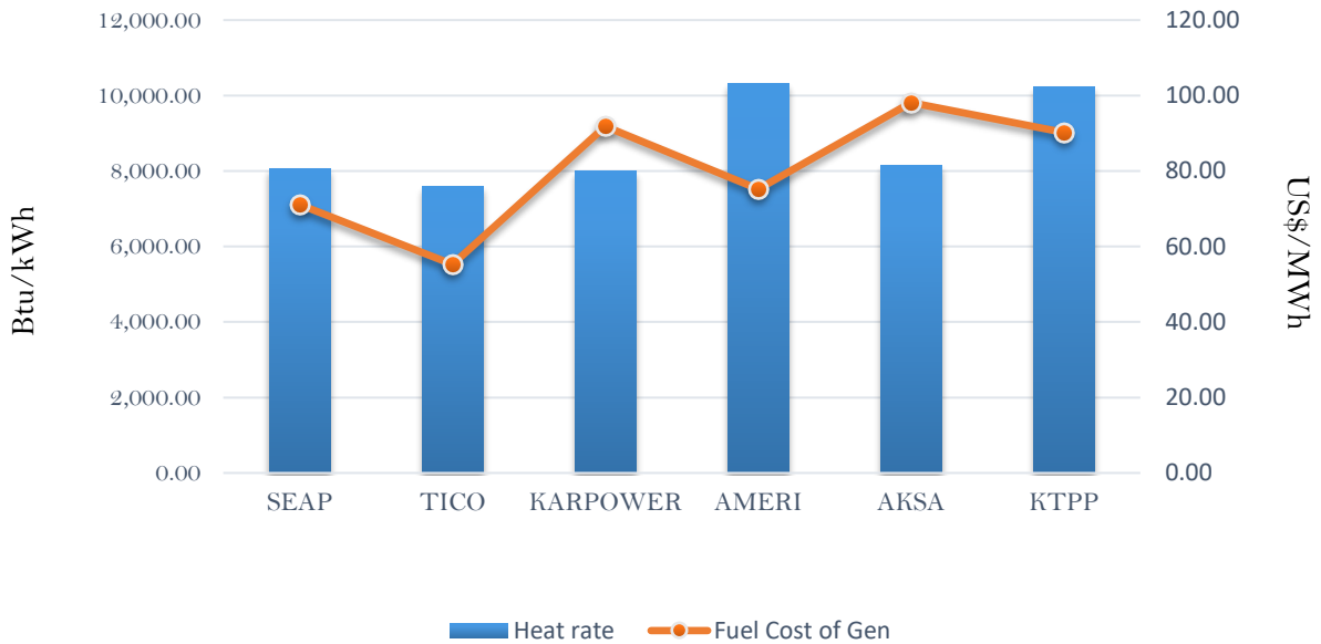
Efficiency and fuel cost of generation on the 17th August 2018
