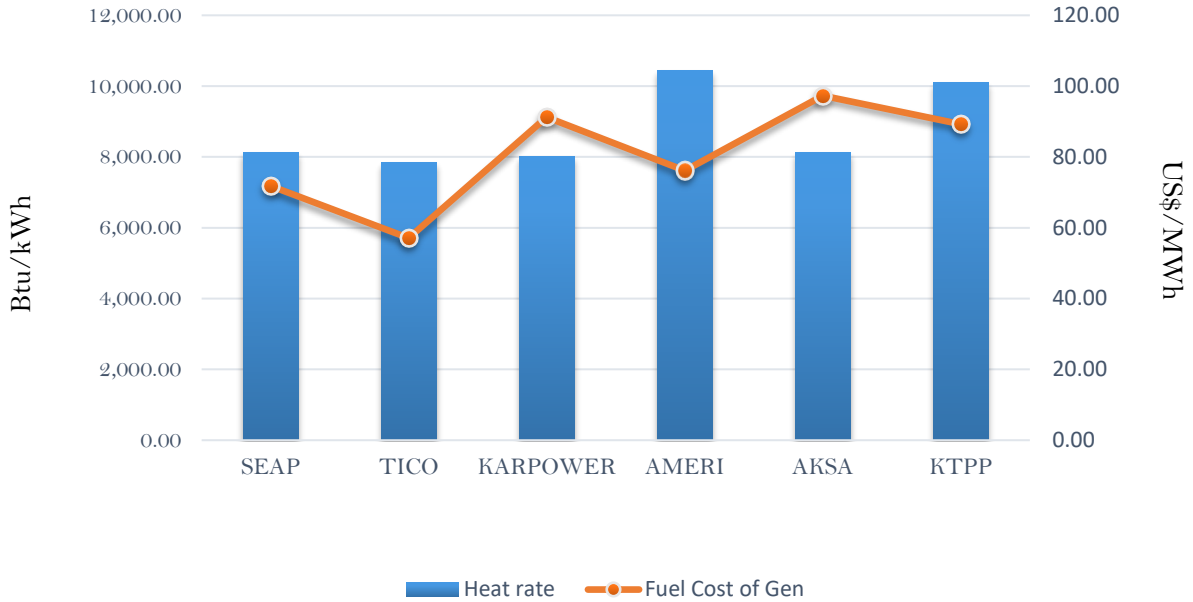
Efficiency and fuel cost of generation on the 15th August 2018
