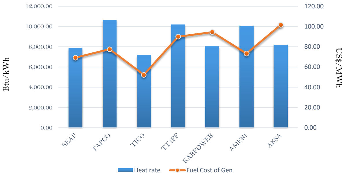
Efficiency and fuel cost of generation on the 11th July 2018
