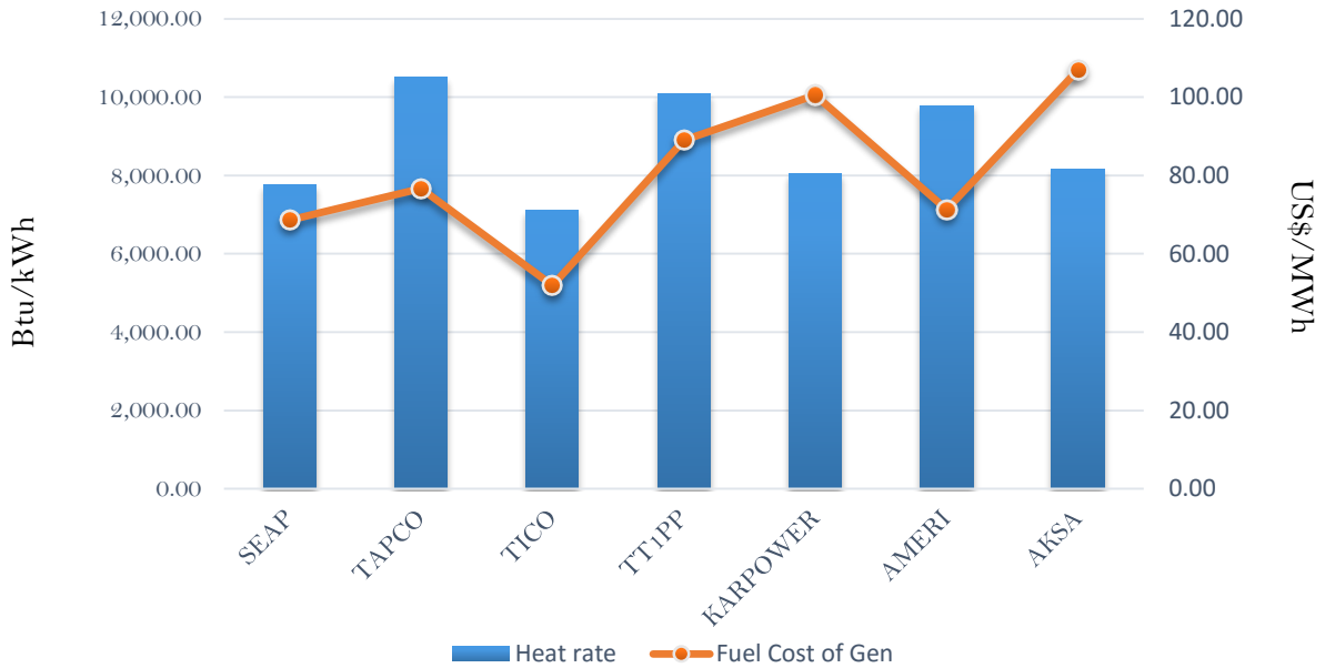
Efficiency and fuel cost of generation on the 10th July 2018
