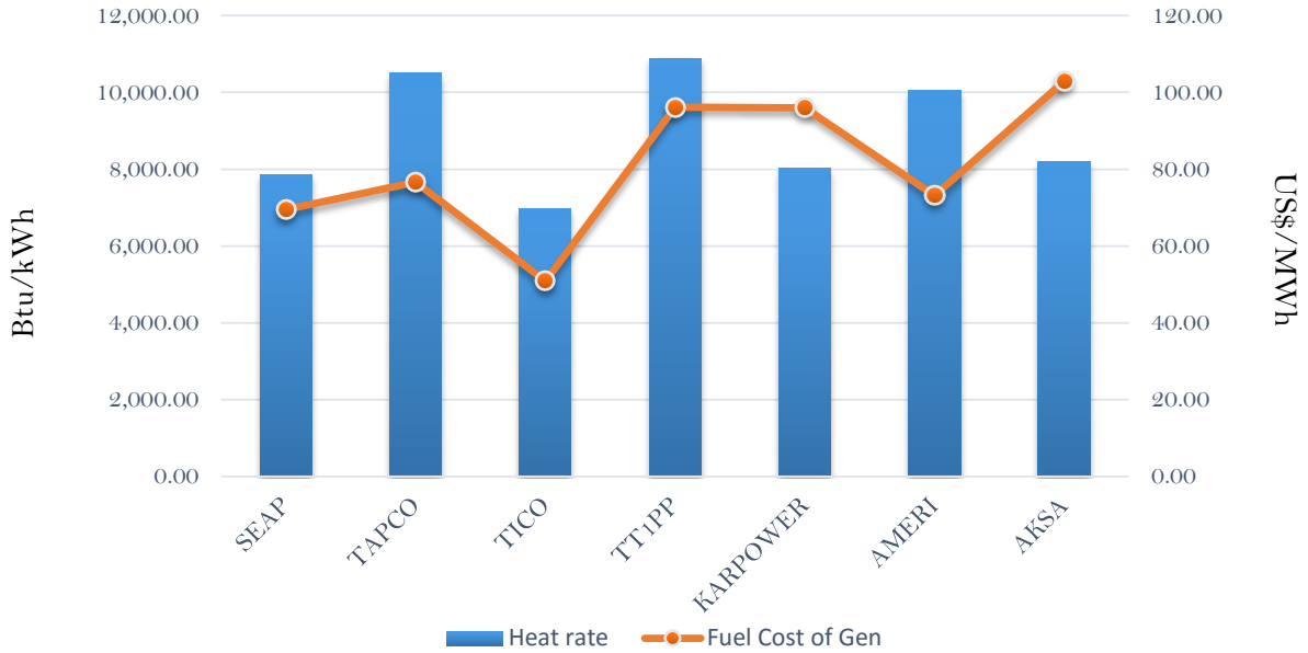
Efficiency and fuel cost of generation on the 12th July 2018
