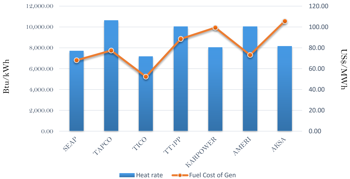
Efficiency and fuel cost of generation on the 9th July 2018
