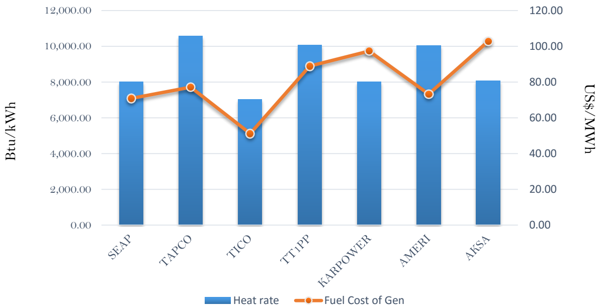
Efficiency and fuel cost of generation on the 13th July 2018
