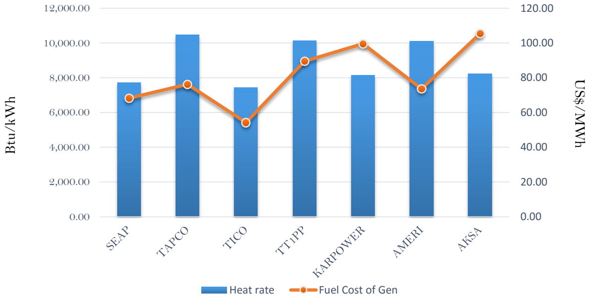
Efficiency and fuel cost of generation on the 8th July 2018
