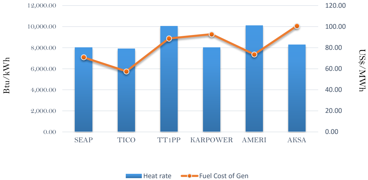
Efficiency and fuel cost of generation on the 17th July 2018
