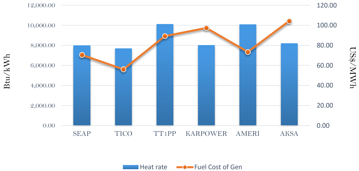
Efficiency and fuel cost of generation on the 15th July 2018
