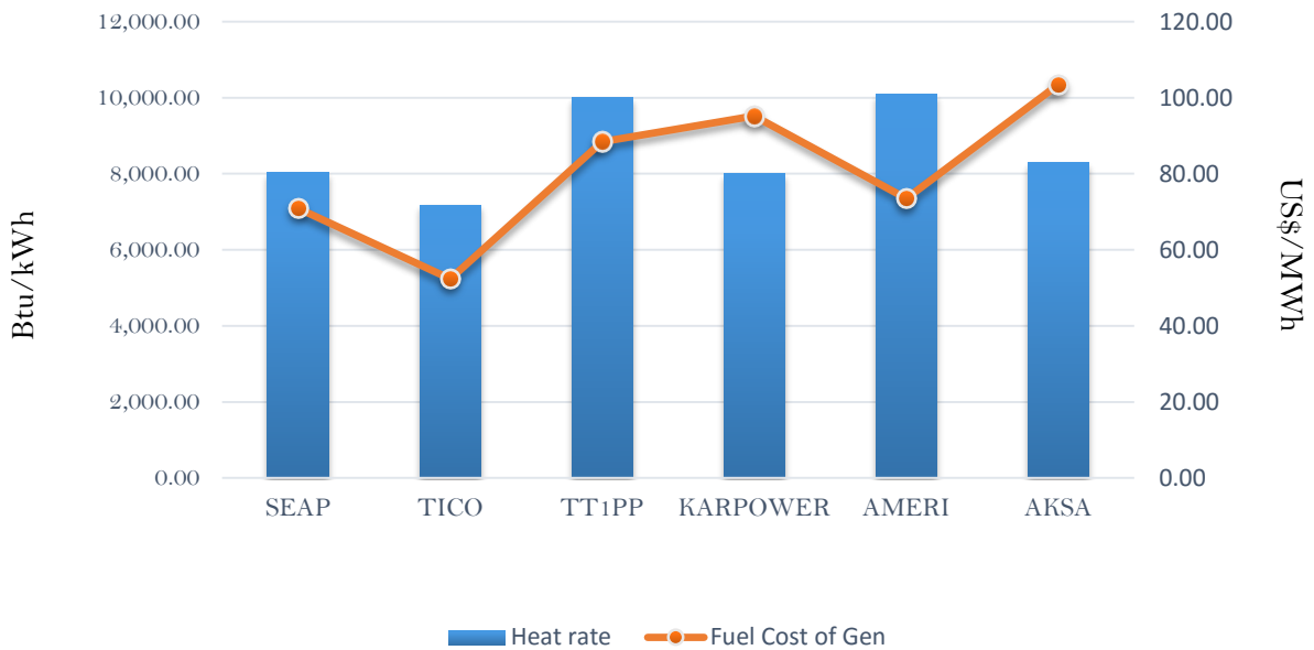
Efficiency and fuel cost of generation on the 20th July 2018
