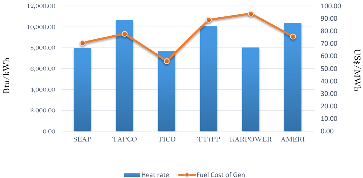
Efficiency and fuel cost of generation on the 18th July 2018
