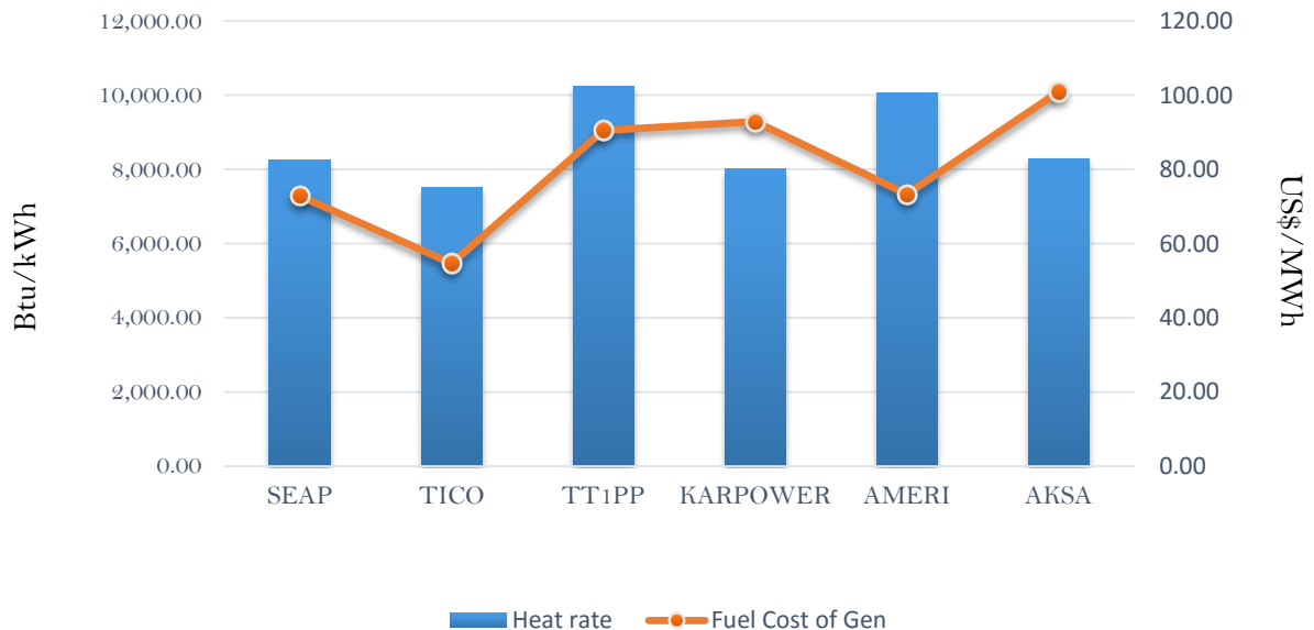
Efficiency and fuel cost of generation on the 16th July 2018
