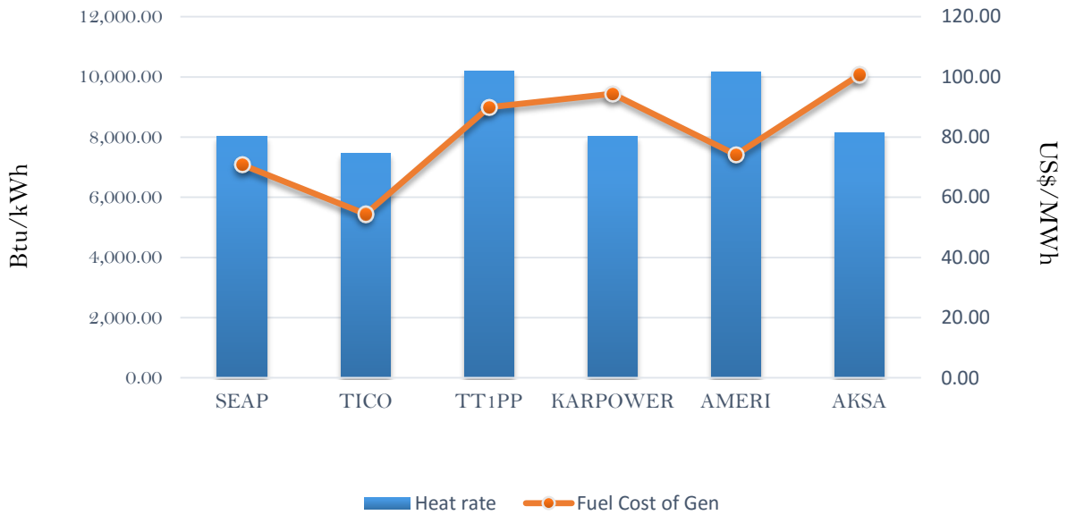
Efficiency and fuel cost of generation on the 19th July 2018
