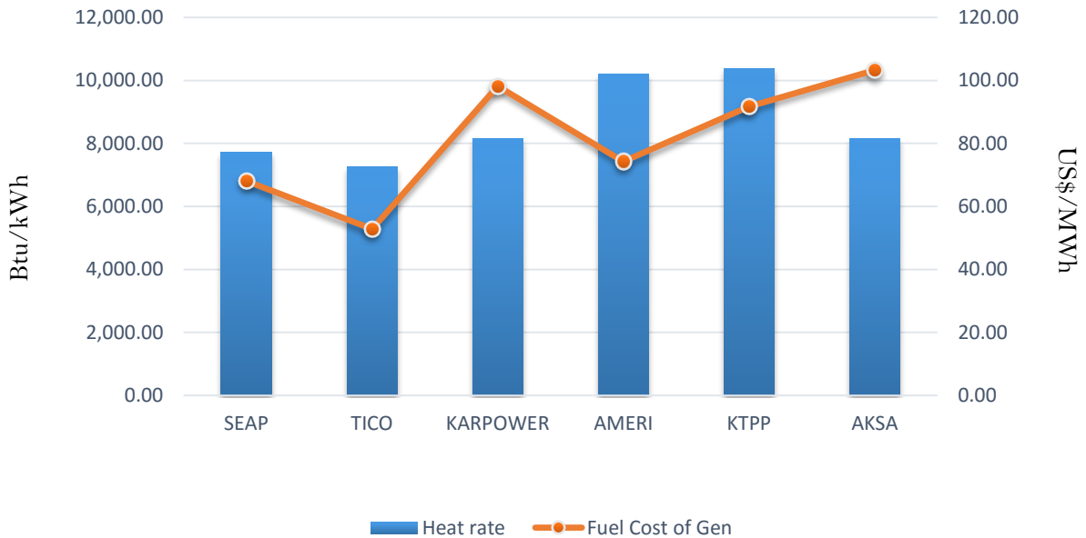
Efficiency and fuel cost of generation on the 2nd June 2018
