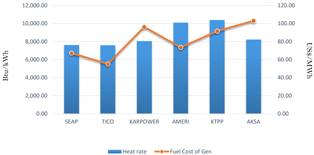
Efficiency and fuel cost of generation on the 4th June 2018
