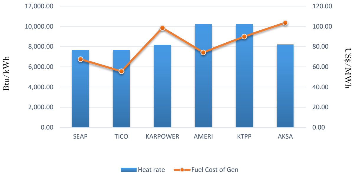
Efficiency and fuel cost of generation on the 5th June 2018
