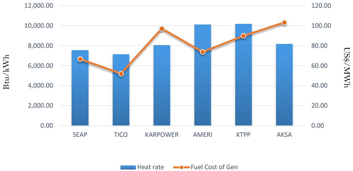
Efficiency and fuel cost of generation on the 1st June 2018
