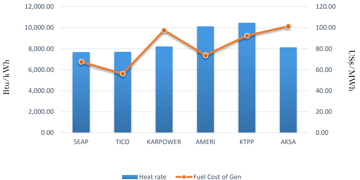
Efficiency and fuel cost of generation on the 6th June 2018
