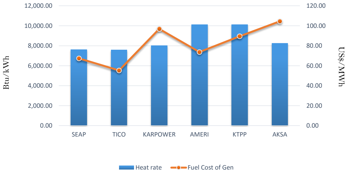
Efficiency and fuel cost of generation on the 3rd June 2018
