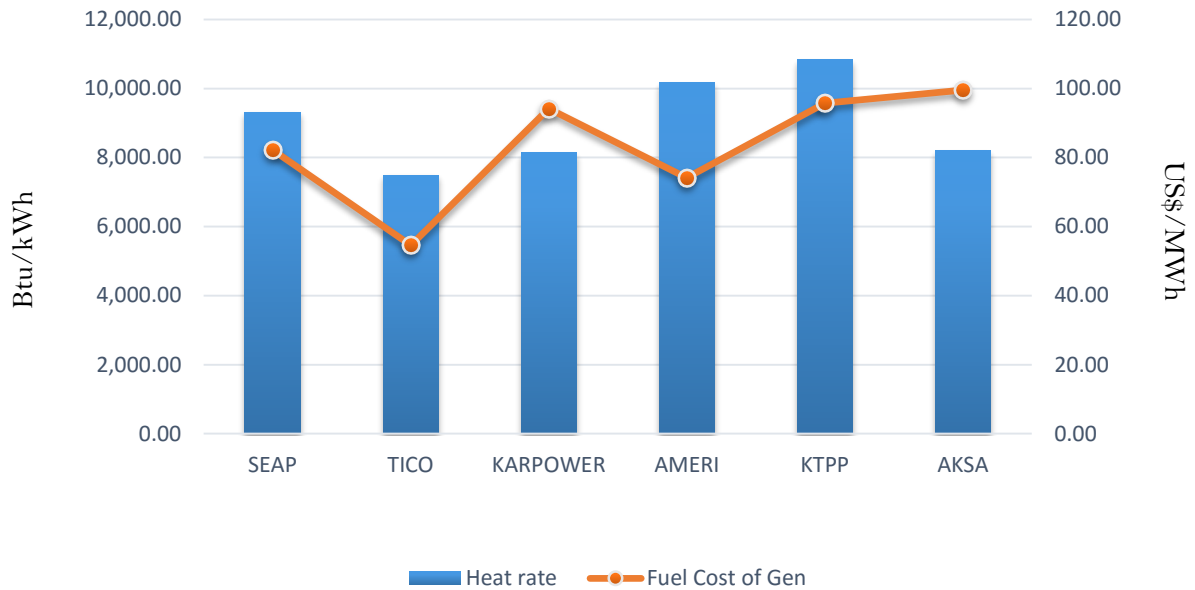
Efficiency and fuel cost of generation on the 15th June 2018
