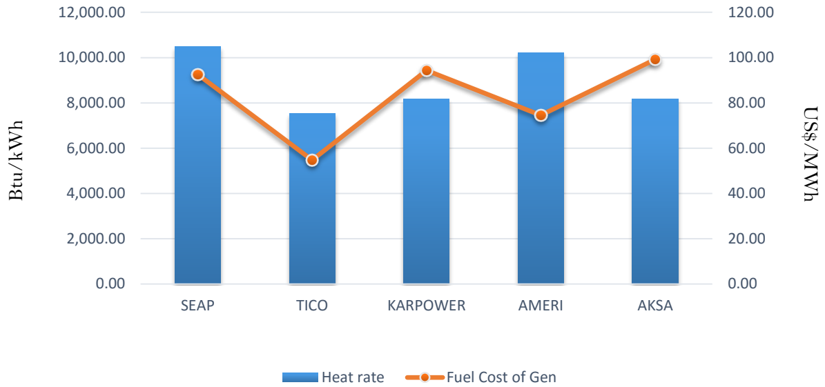
Efficiency and fuel cost of generation on the 17th June 2018
