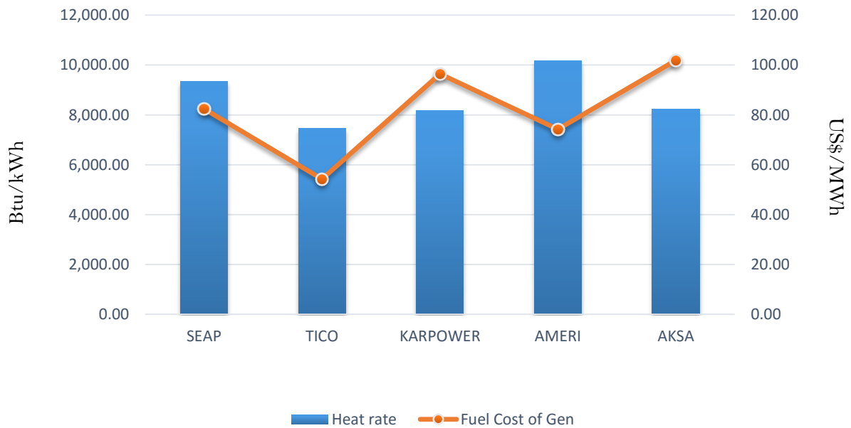
Efficiency and fuel cost of generation on the 18th June 2018
