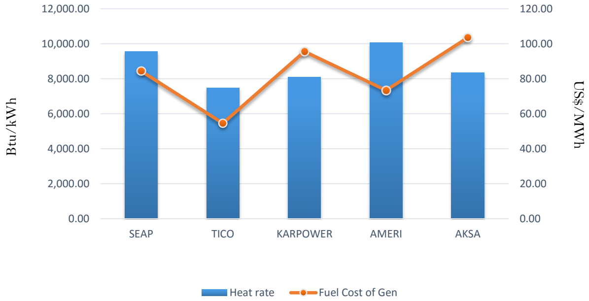
Efficiency and fuel cost of generation on the 19th June 2018
