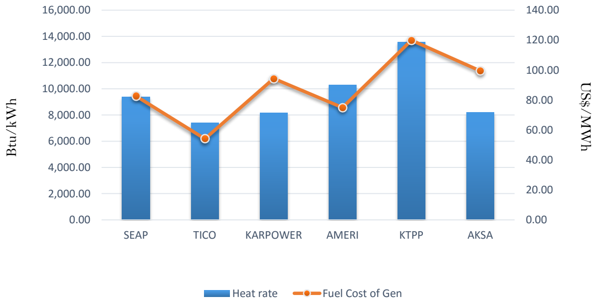
Efficiency and fuel cost of generation on the 16th June 2018
