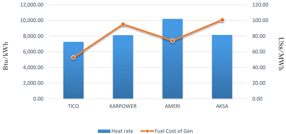
Efficiency and fuel cost of generation on the 20th June 2018
