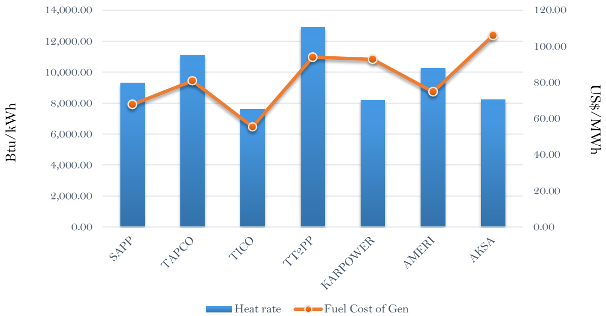
Efficiency and fuel cost of generation on the 4th March 2019
