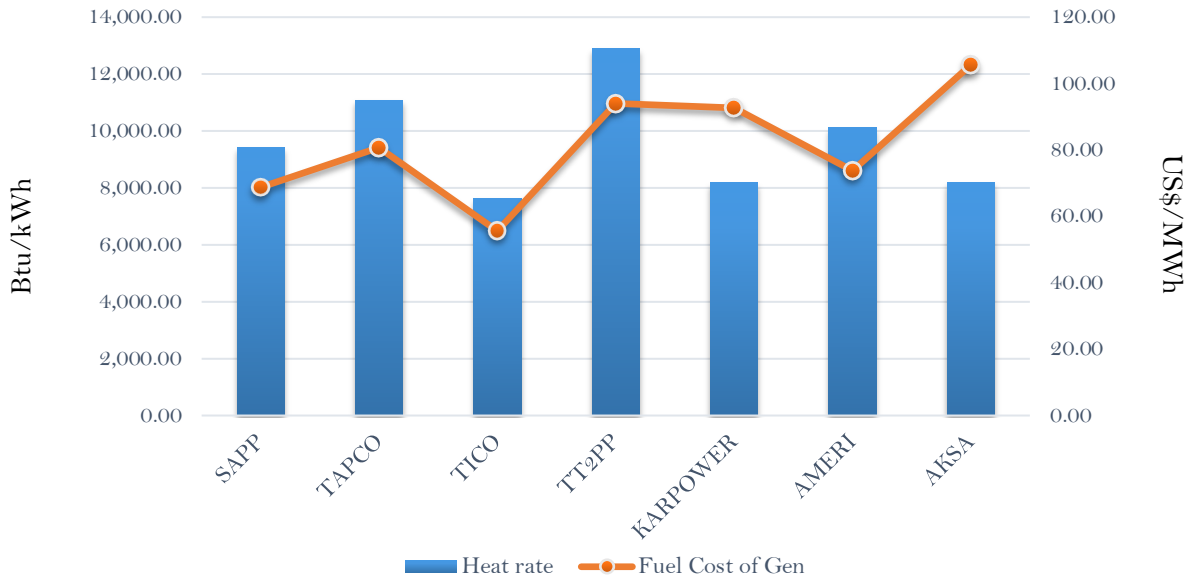
Efficiency and fuel cost of generation on the 5th March 2019
