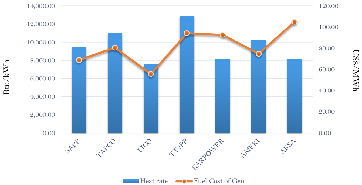
Efficiency and fuel cost of generation on the 6th March 2019
