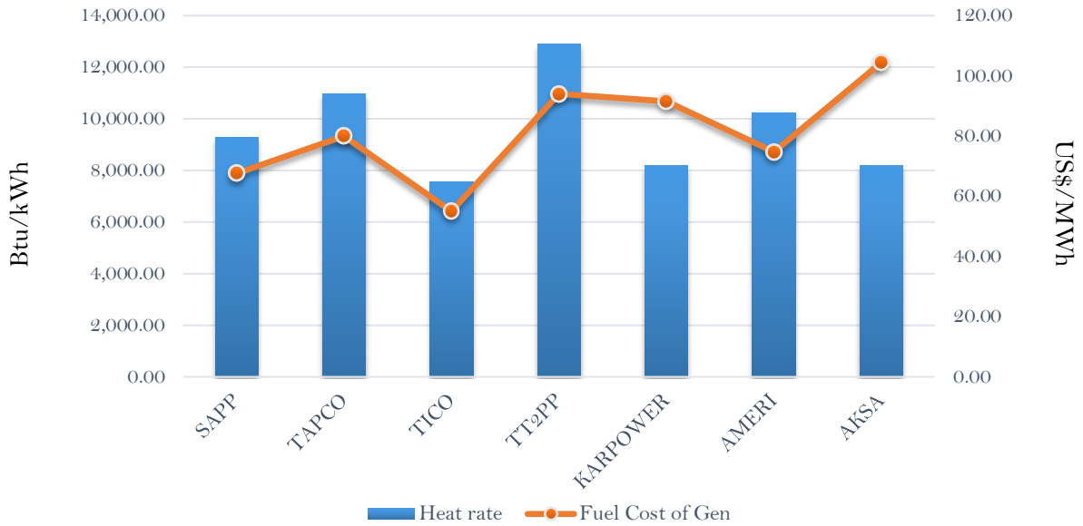
Efficiency and fuel cost of generation on the 1st March 2019
