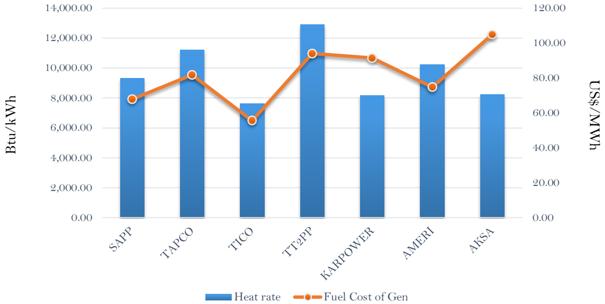
Efficiency and fuel cost of generation on the 4th March 2019
