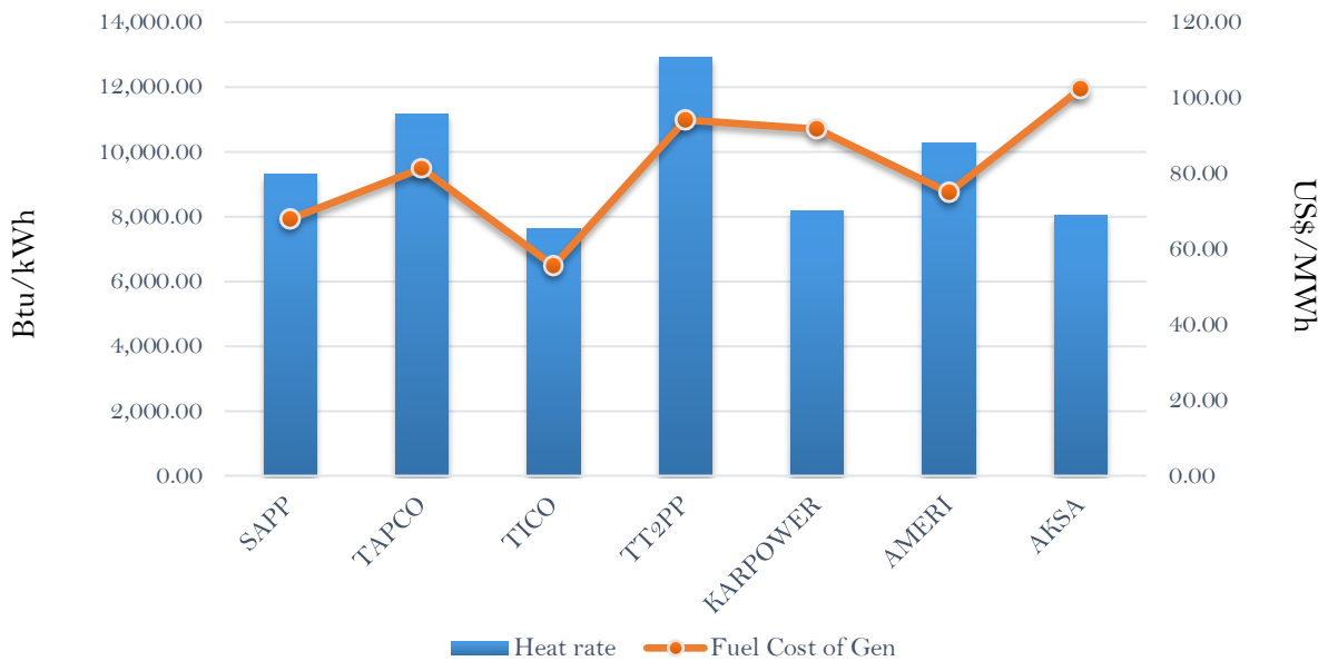
Efficiency and fuel cost of generation on the 2nd March 2019
