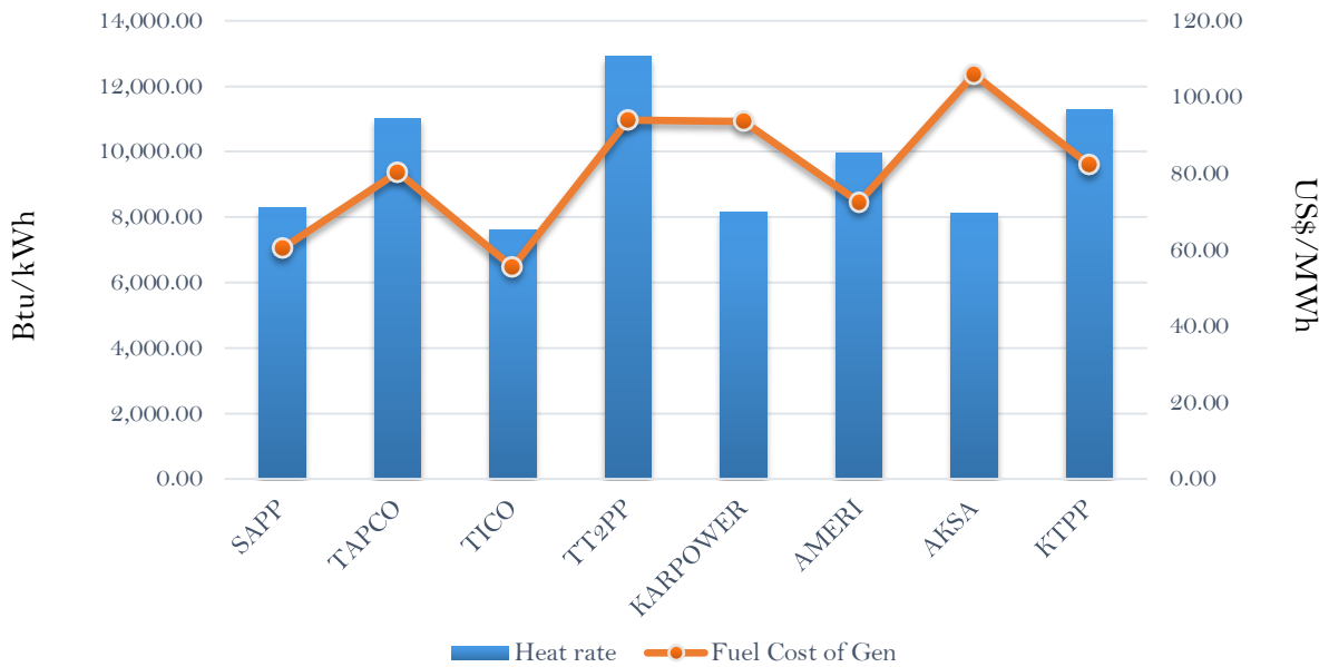
Efficiency and fuel cost of generation on the 13th March 2019
