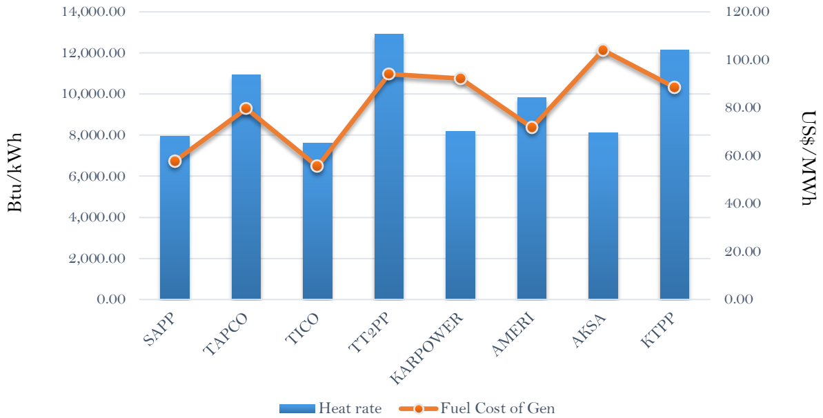
Efficiency and fuel cost of generation on the 11th March 2019
