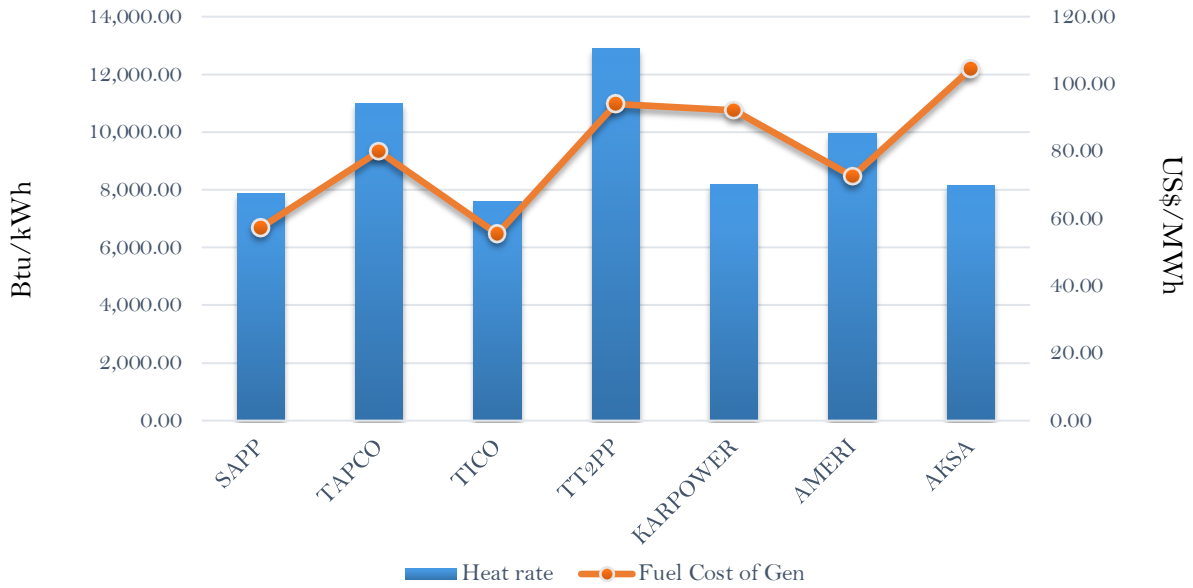
Efficiency and fuel cost of generation on the 9th March 2019
