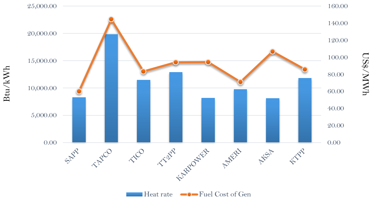
Efficiency and fuel cost of generation on the 13th March 2019
