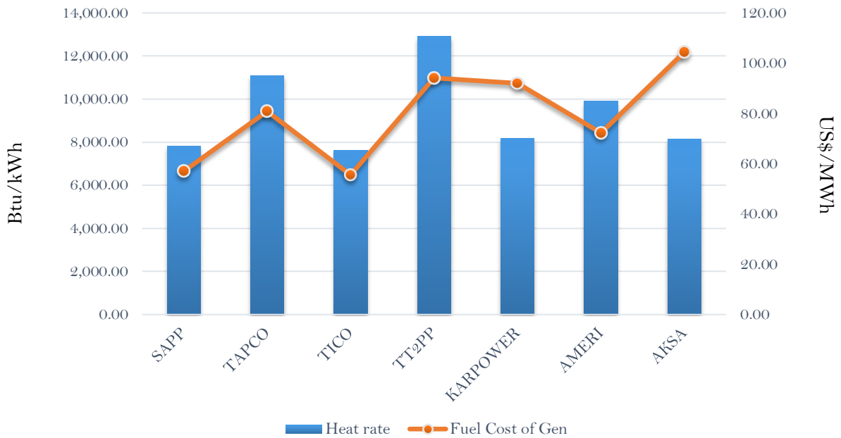
Efficiency and fuel cost of generation on the 9th March 2019
