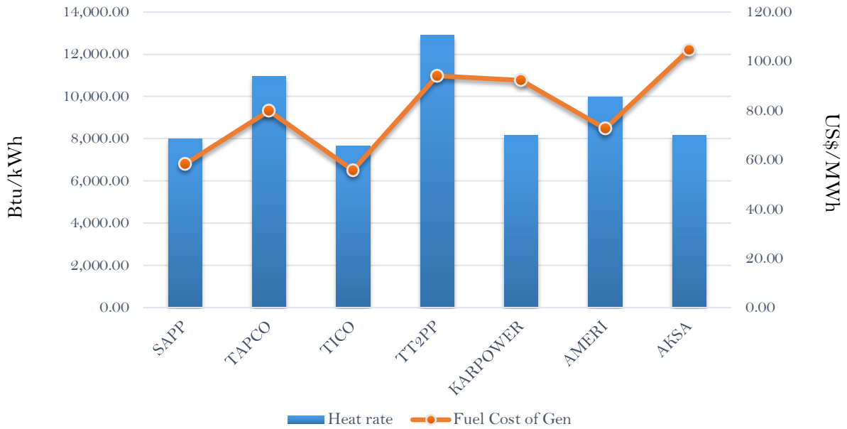
Efficiency and fuel cost of generation on the 25th March 2019
