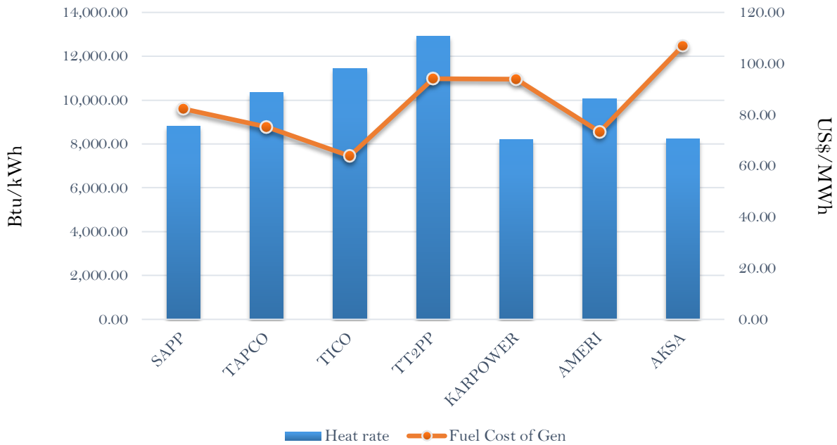
Efficiency and fuel cost of generation on the 29th March 2019
