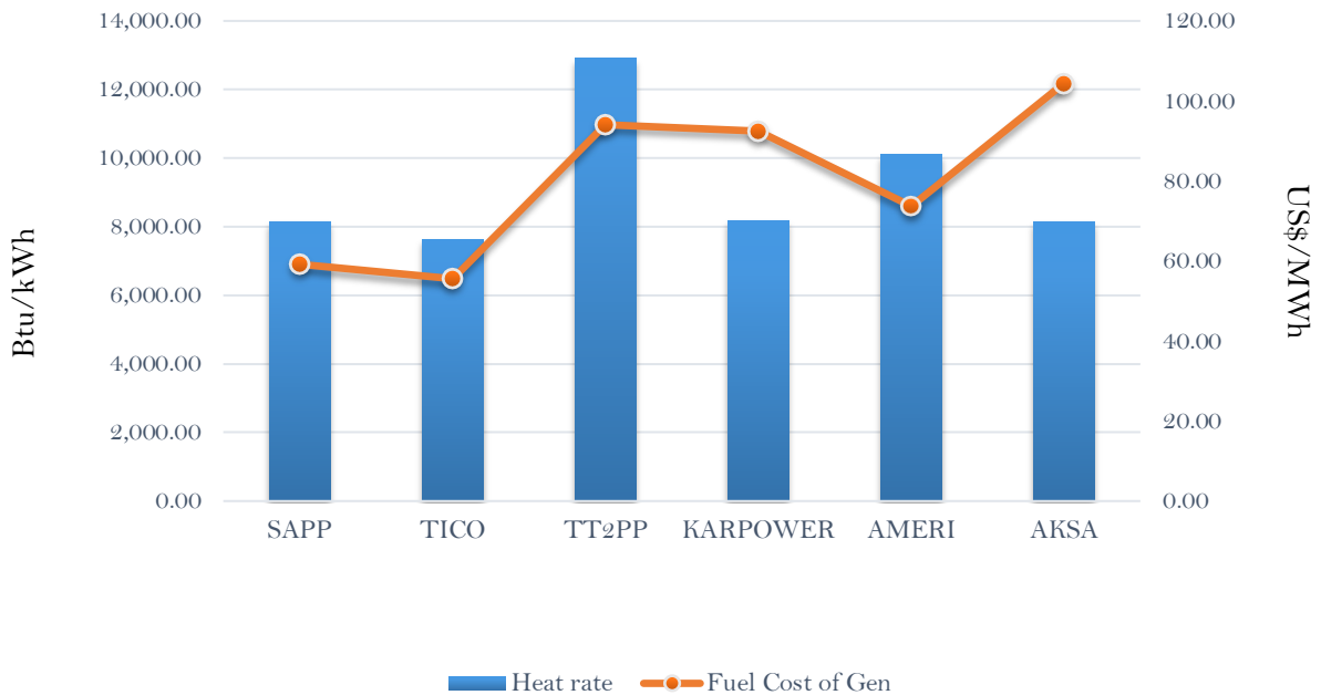
Efficiency and fuel cost of generation on the 25th March 2019
