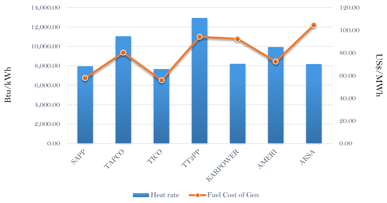
Efficiency and fuel cost of generation on the 23rd March 2019
