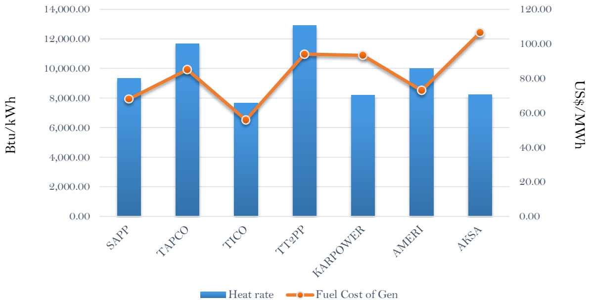
Efficiency and fuel cost of generation on the 27th March 2019
