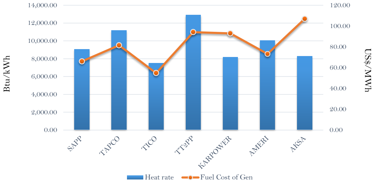
Efficiency and fuel cost of generation on the 28th March 2019
