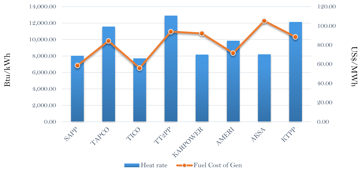
Efficiency and fuel cost of generation on the 23rd March 2019
