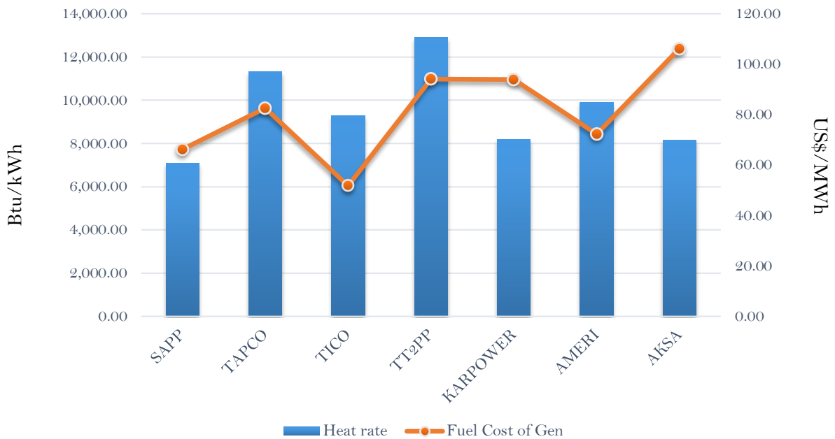
Efficiency and fuel cost of generation on the 30th March 2019
