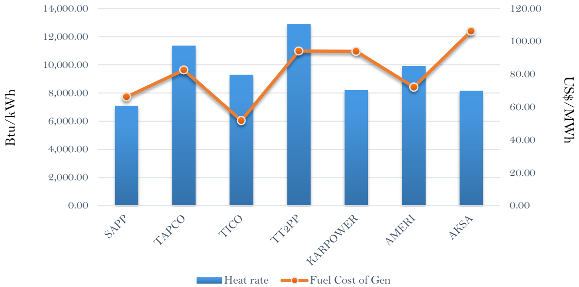
Efficiency and fuel cost of generation on the 30th March 2019
