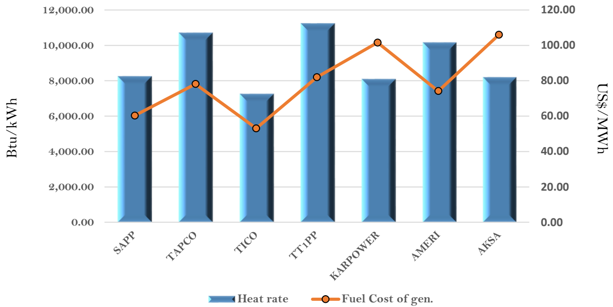
Efficiency and fuel cost of generation on the 19th May 2018
