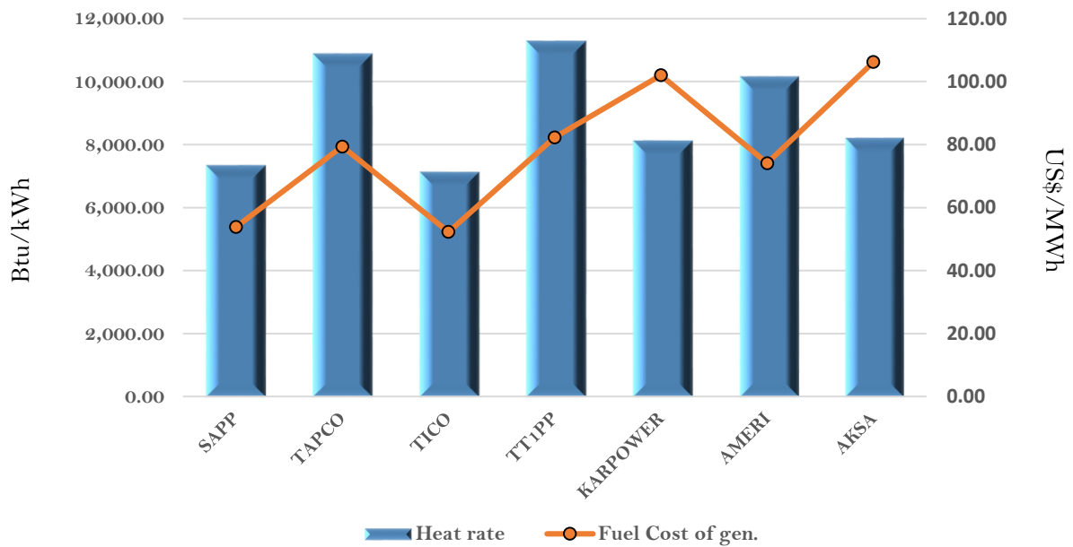
Efficiency and fuel cost of generation on the 20th May 2018
