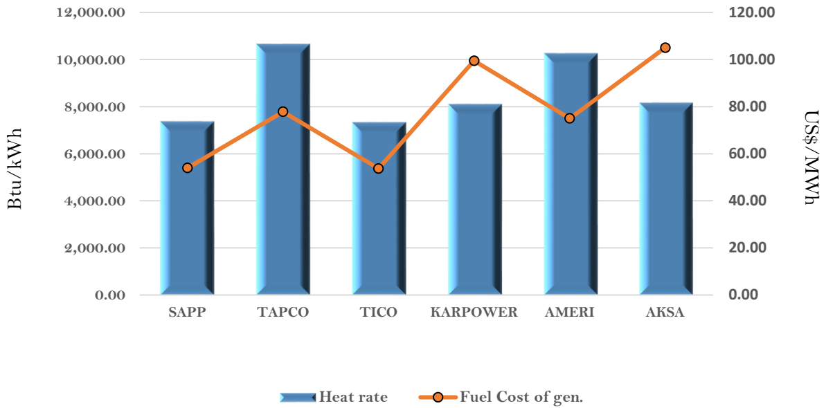
Efficiency and fuel cost of generation on the 25th May 2018
