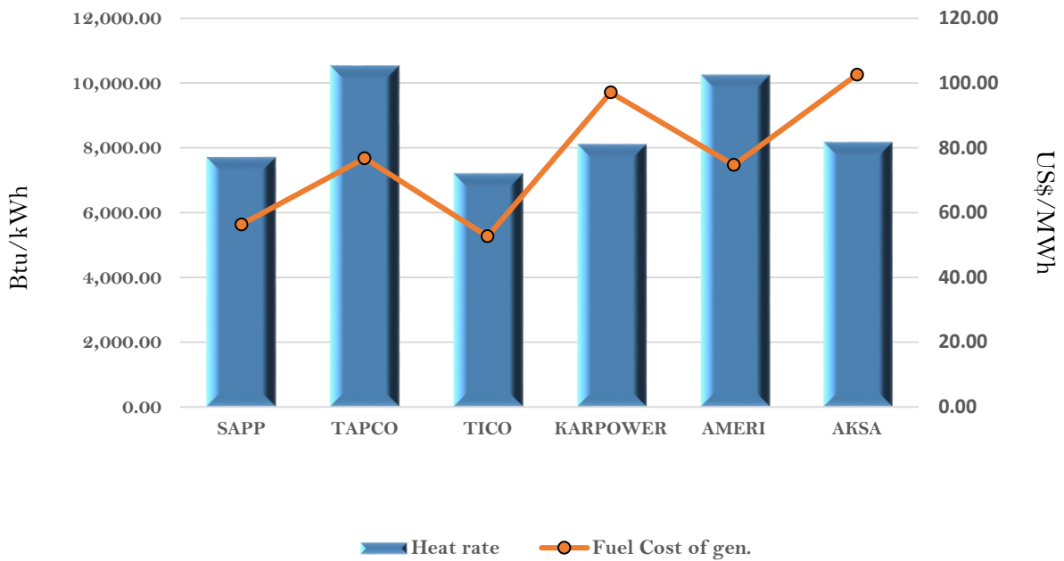
Efficiency and fuel cost of generation on the 25th May 2018
