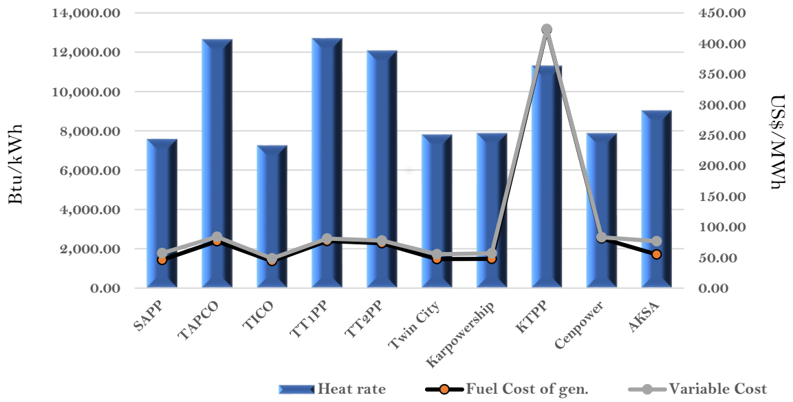
Efficiency and fuel cost of generation on the 21st April 2022
