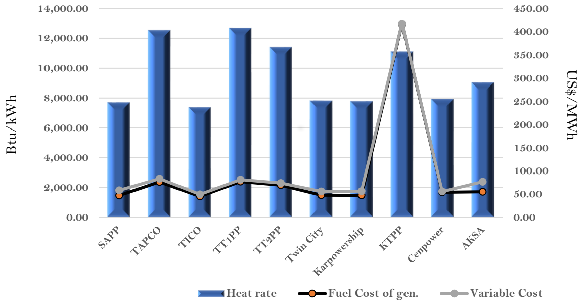
Efficiency and fuel cost of generation on the 21st April 2022
