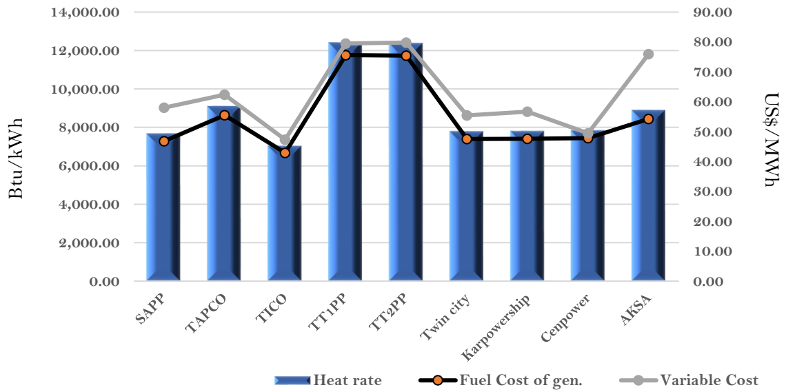
Efficiency and fuel cost of generation on the 30th April 2022
