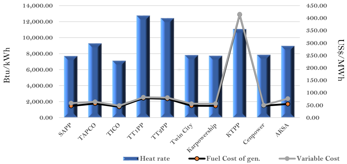
Efficiency and fuel cost of generation on the 28th April 2022
