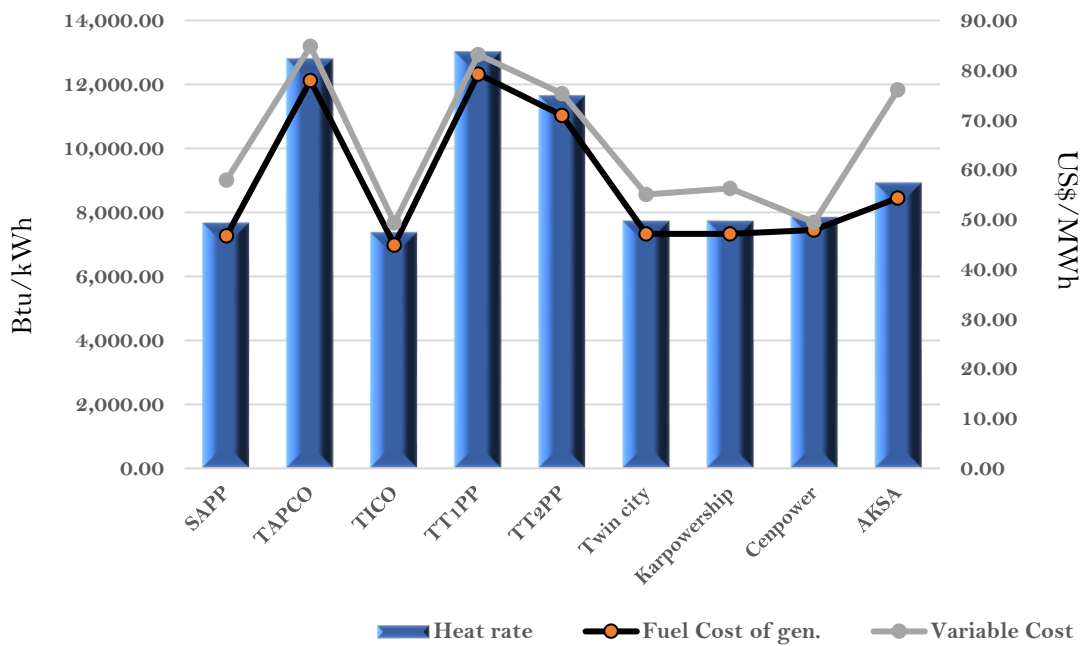
Efficiency and fuel cost of generation on the 28th April 2022
