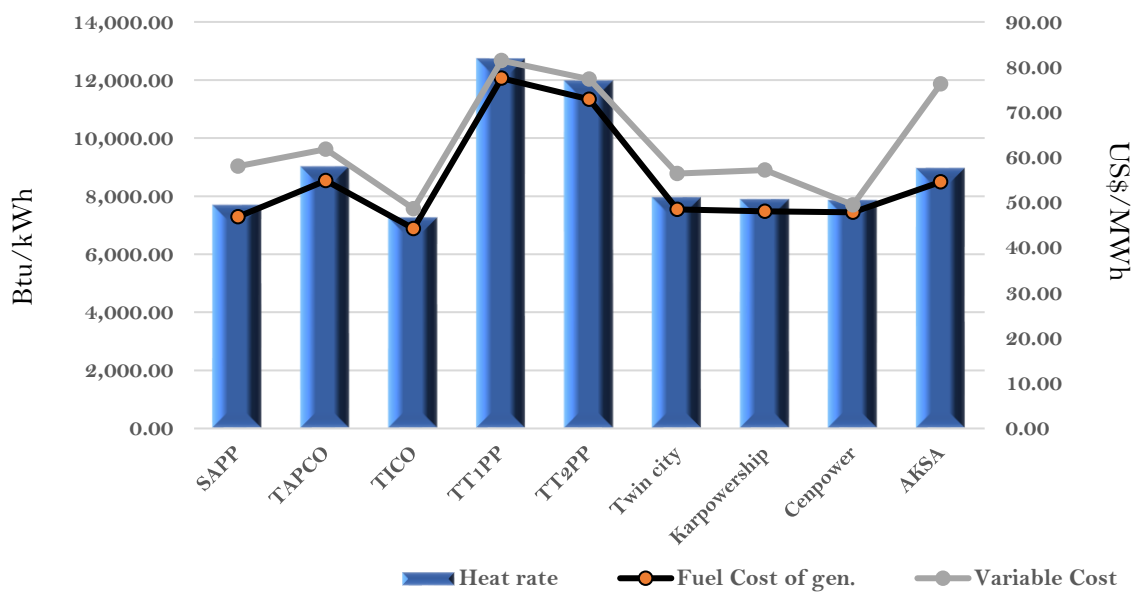
Efficiency and fuel cost of generation on the 30th April 2022
