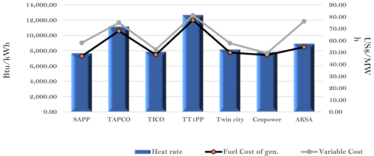
Efficiency and fuel cost of generation on the 31st August 2022
