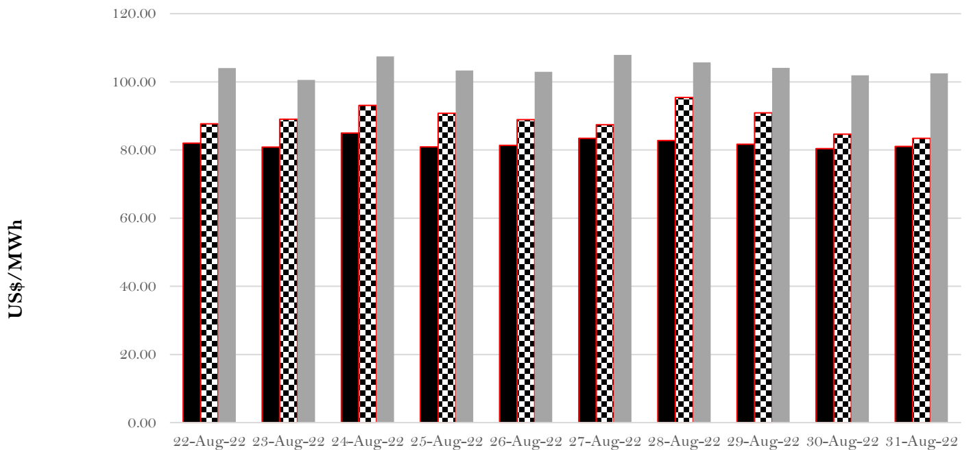
System Marginal Cost Vs Average Market Prices for Week 4 of August 2022
