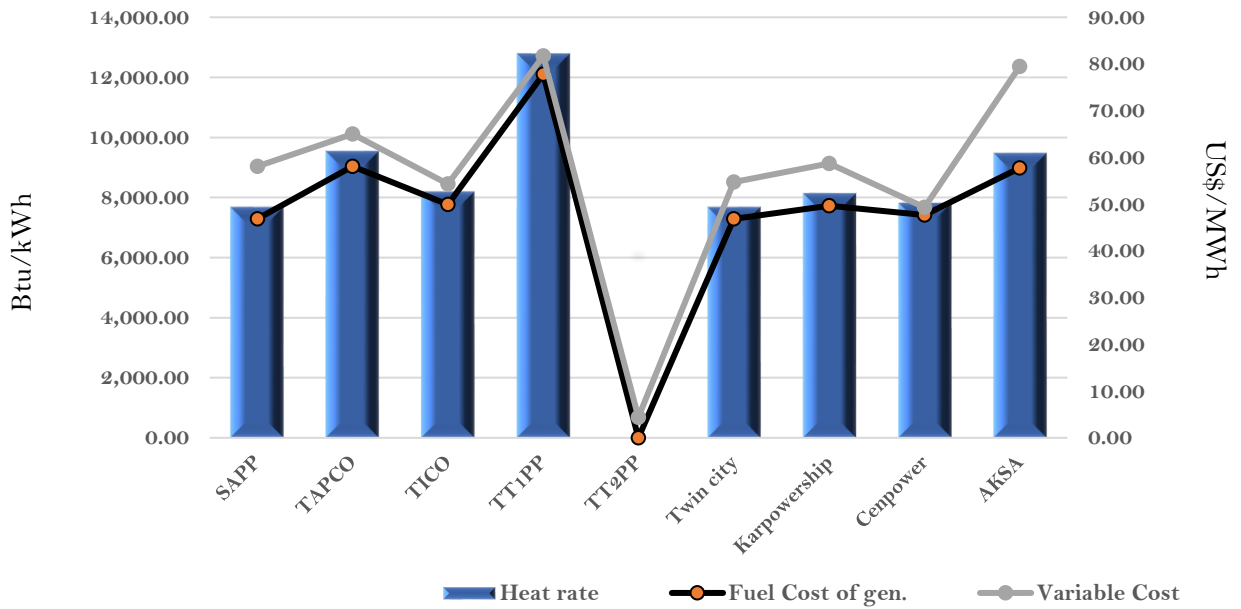
Efficiency and fuel cost of generation on the 29th August 2022
