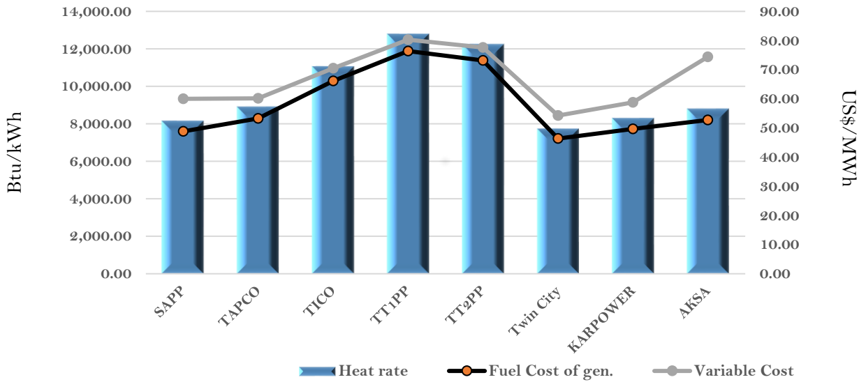
Efficiency and fuel cost of generation on the 6th December 2022
