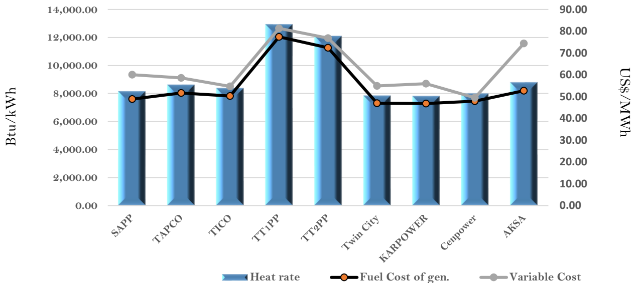
Efficiency and fuel cost of generation on the 3rd December 2022
