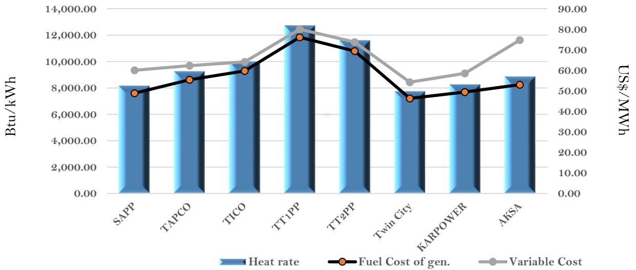
Efficiency and fuel cost of generation on the 7th December 2022
