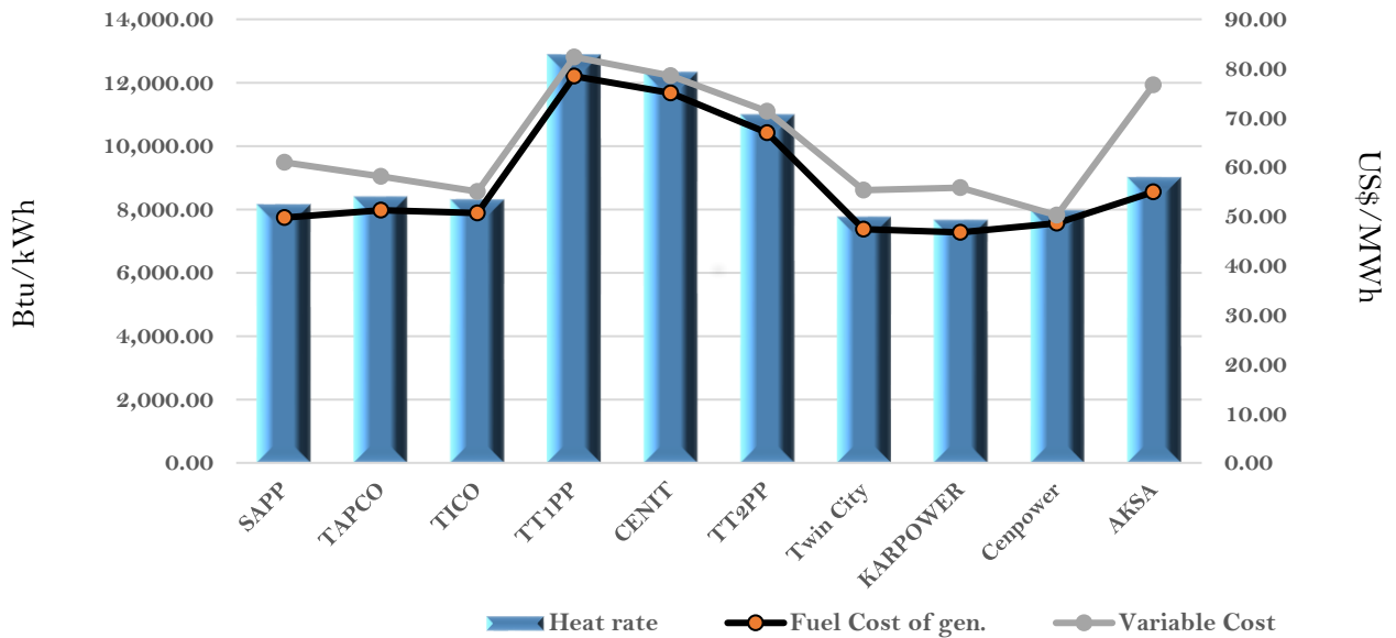
Efficiency and fuel cost of generation on the 2nd December 2022
