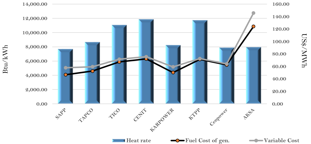
Efficiency and fuel cost of generation on the 30th January 2022
