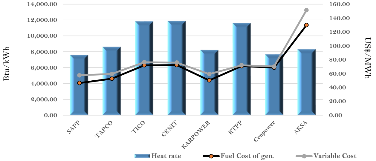
Efficiency and fuel cost of generation on the 29th January 2022
