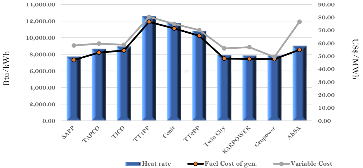
Efficiency and fuel cost of generation on the 6th June 2022
