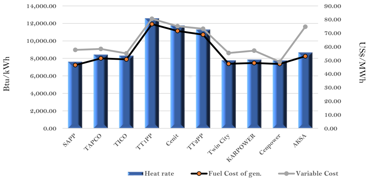
Efficiency and fuel cost of generation on the 7th June 2022
