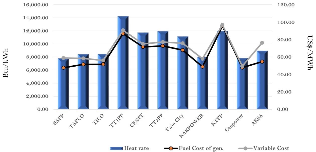
Efficiency and fuel cost of generation on the 4th June 2022
