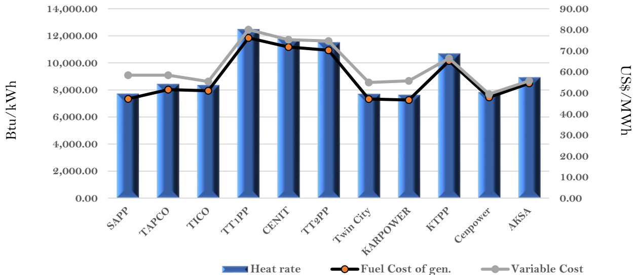
Efficiency and fuel cost of generation on the 5th June 2022
