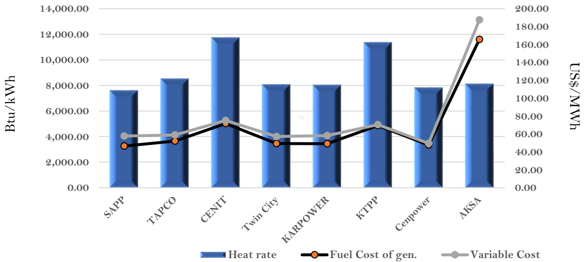
Efficiency and fuel cost of generation on the 4th March 2022
