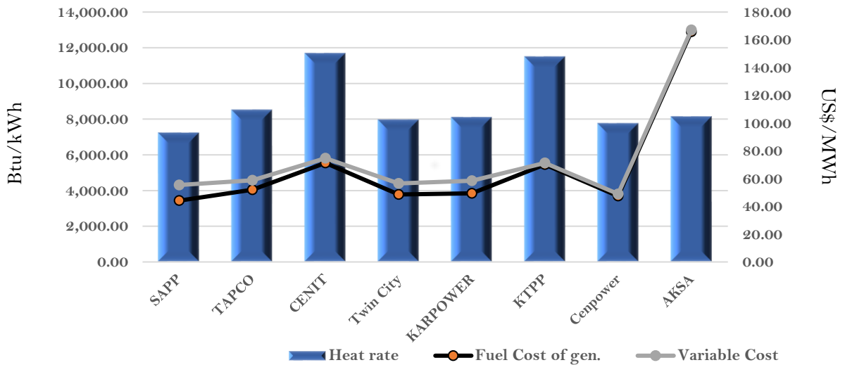
Efficiency and fuel cost of generation on the 5th March 2022
