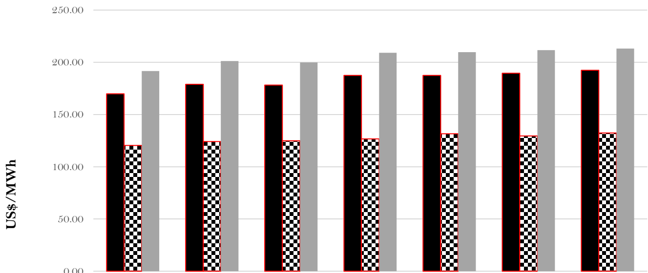
System Marginal Cost Vs Average Market Prices for Week 1 of March 2022
