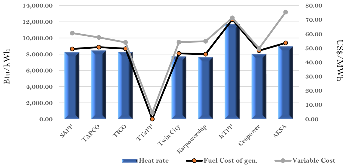
Efficiency and fuel cost of generation on the 21st November 2022
