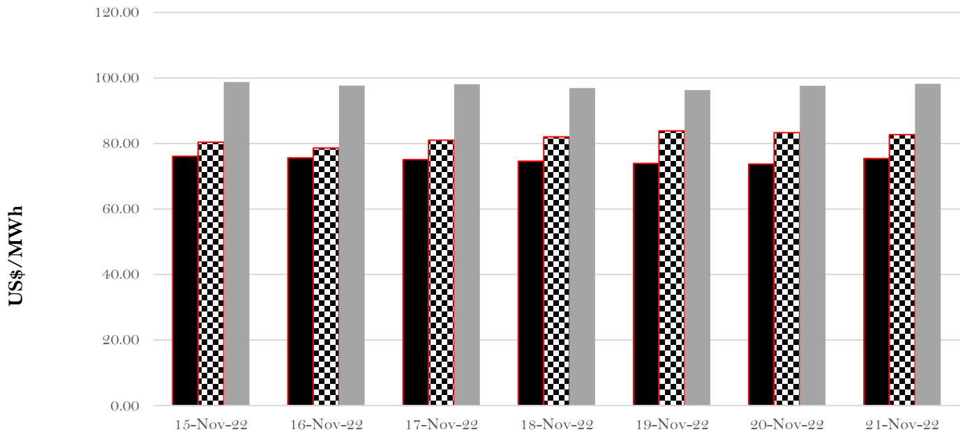
System Marginal Cost Vs Average Market Prices for Week 3 of November 2022
