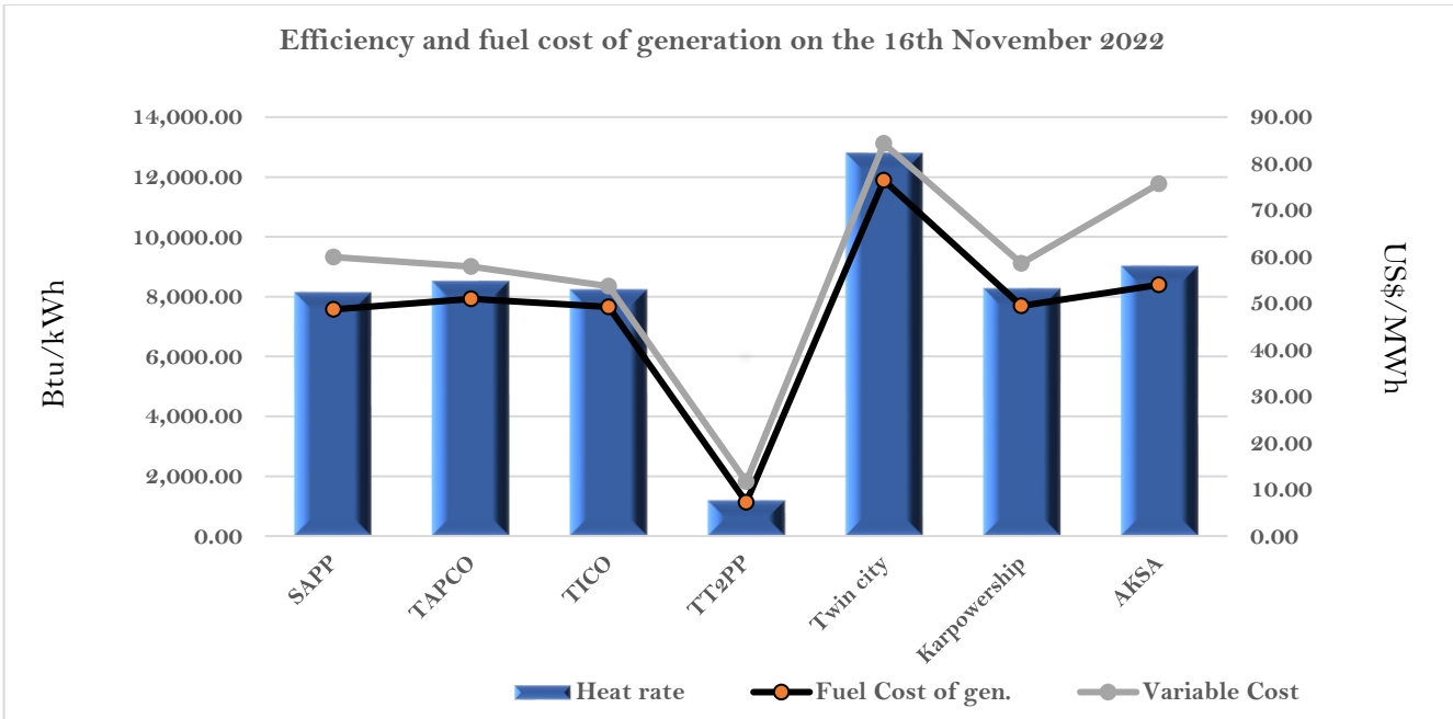
Efficiency and fuel cost of generation on the 17th November 2022
