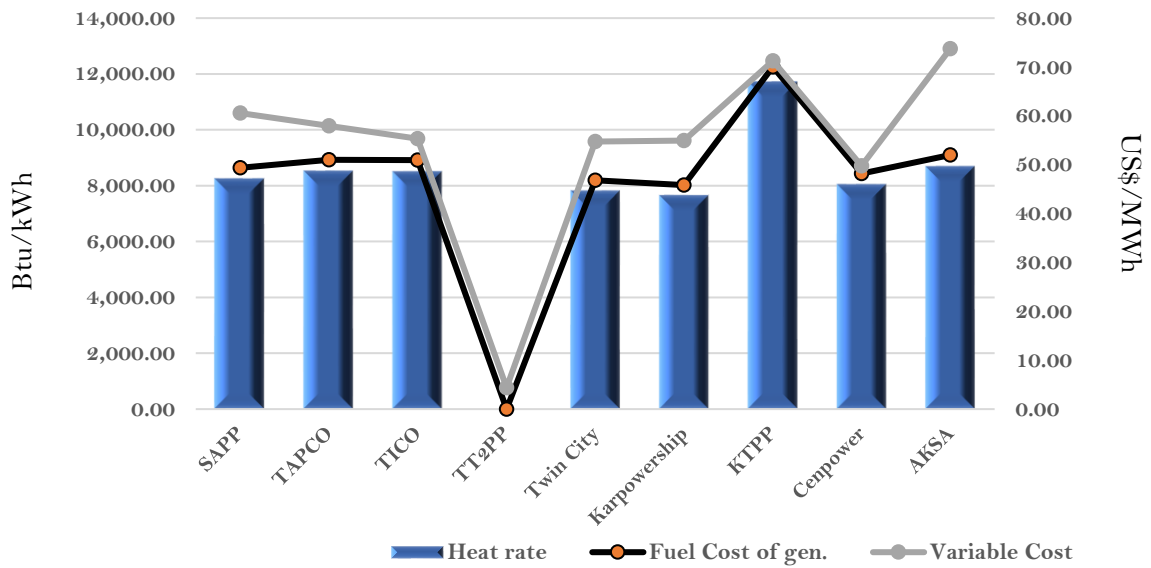
Efficiency and fuel cost of generation on the 21st November 2022
