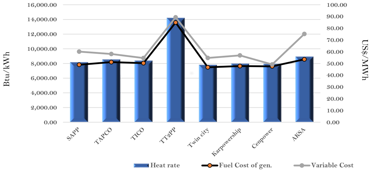
Efficiency and fuel cost of generation on the 29th November 2022
