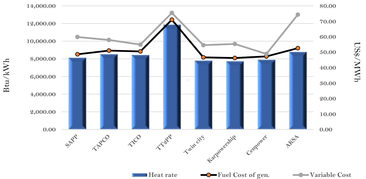
Efficiency and fuel cost of generation on the 30th November 2022
