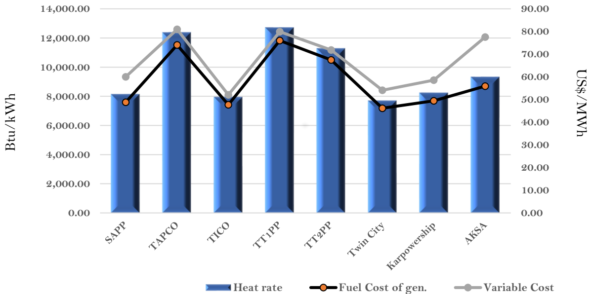
Efficiency and fuel cost of generation on the 19th October 2022
