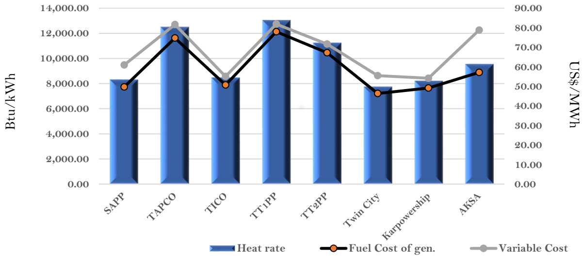
Efficiency and fuel cost of generation on the 18th October 2022
