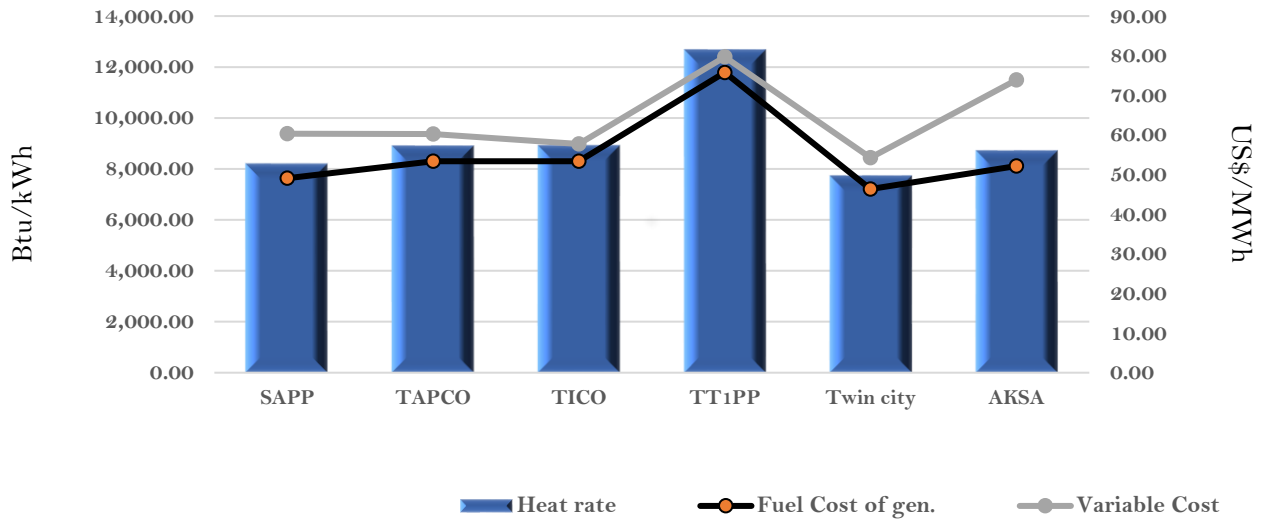
Efficiency and fuel cost of generation on the 31st October 2022
