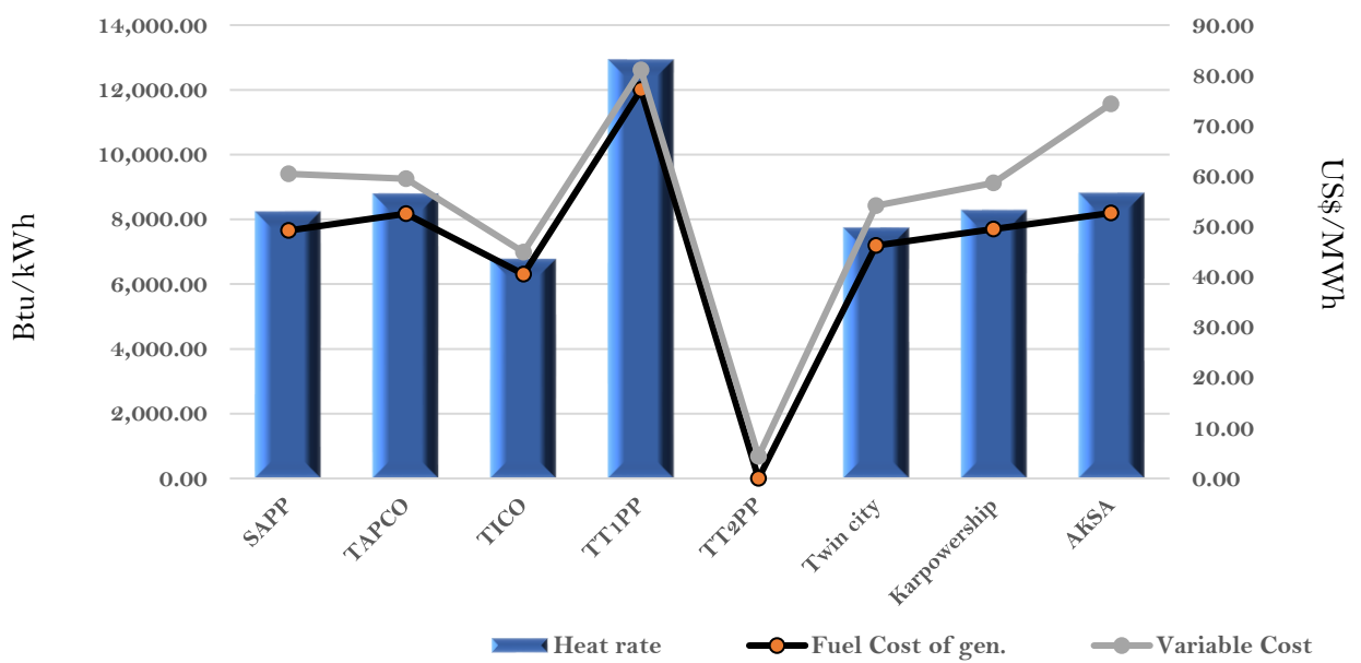
Efficiency and fuel cost of generation on the 30th October 2022
