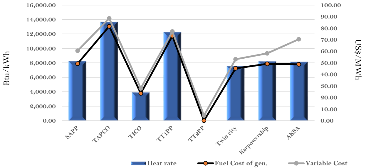
Efficiency and fuel cost of generation on the 29th October 2022
