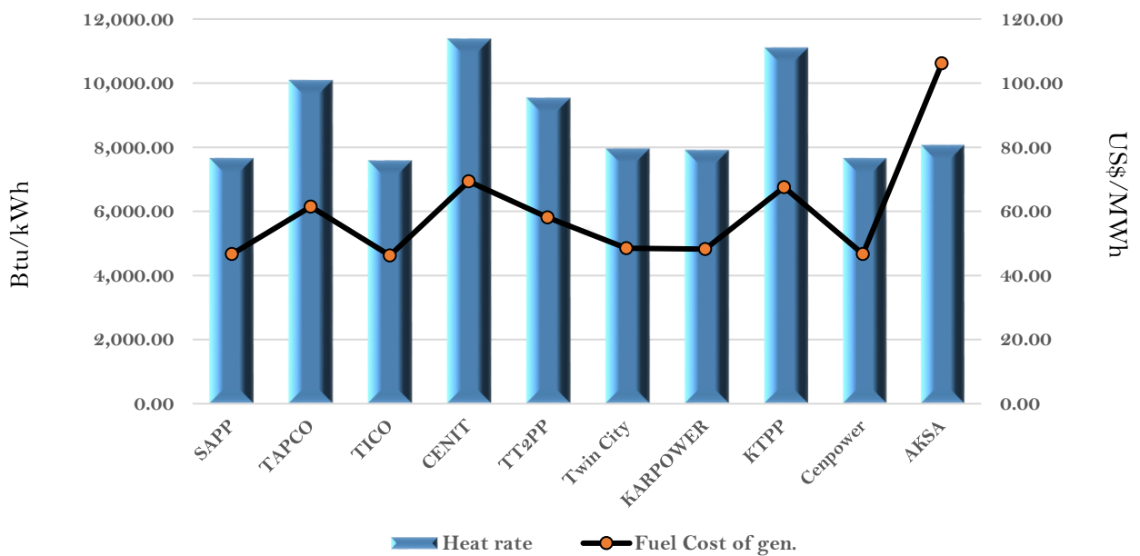
Efficiency and fuel cost of generation on the 7th April 2021
