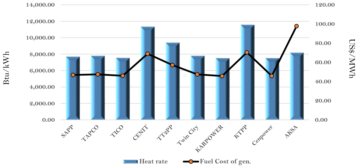
Efficiency and fuel cost of generation on the 6th April 2021
