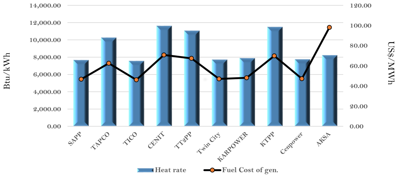
Efficiency and fuel cost of generation on the 9th April 2021
