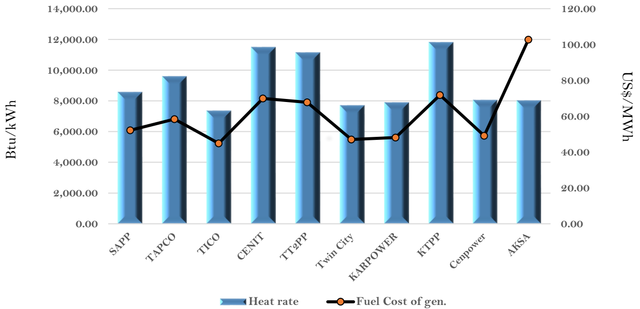
Efficiency and fuel cost of generation on the 10th April 2021
