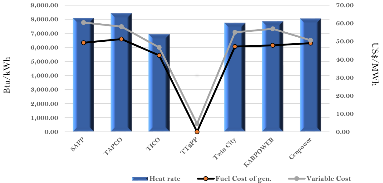
Efficiency and fuel cost of generation on the 7th January 2023
