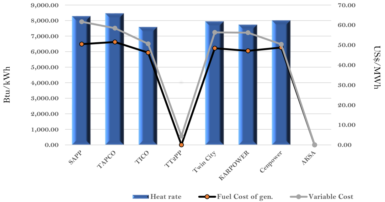
Efficiency and fuel cost of generation on the 7th January 2023
