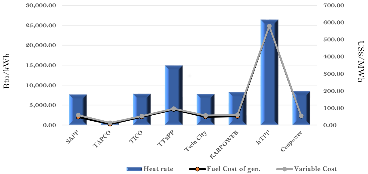
Efficiency and fuel cost of generation on the 14th January 2023
