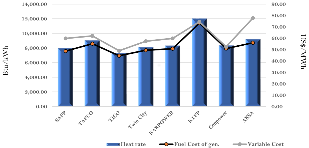
Efficiency and fuel cost of generation on the 7th May 2023
