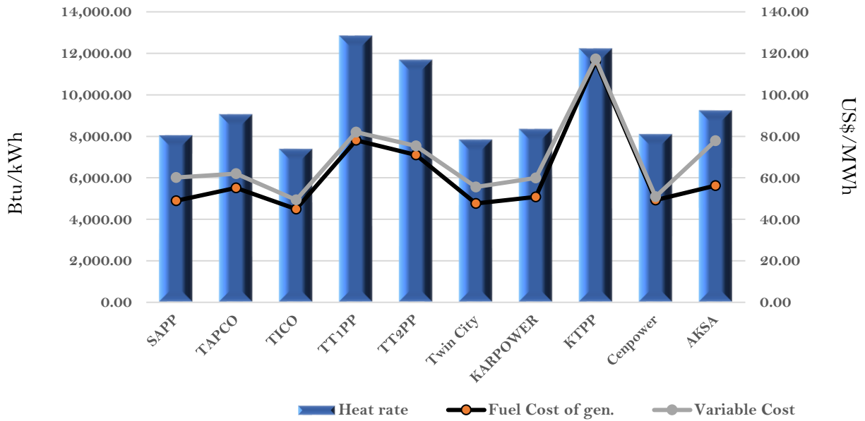
Efficiency and fuel cost of generation on the 6th May 2023
