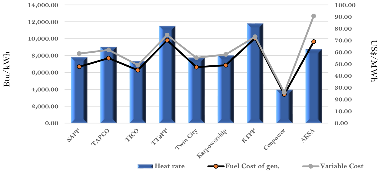
Efficiency and fuel cost of generation on the 25th May 2023
