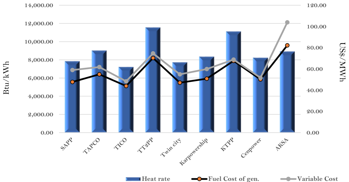
Efficiency and fuel cost of generation on the 28th May 2023
