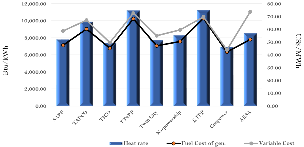
Efficiency and fuel cost of generation on the 27th May 2023
