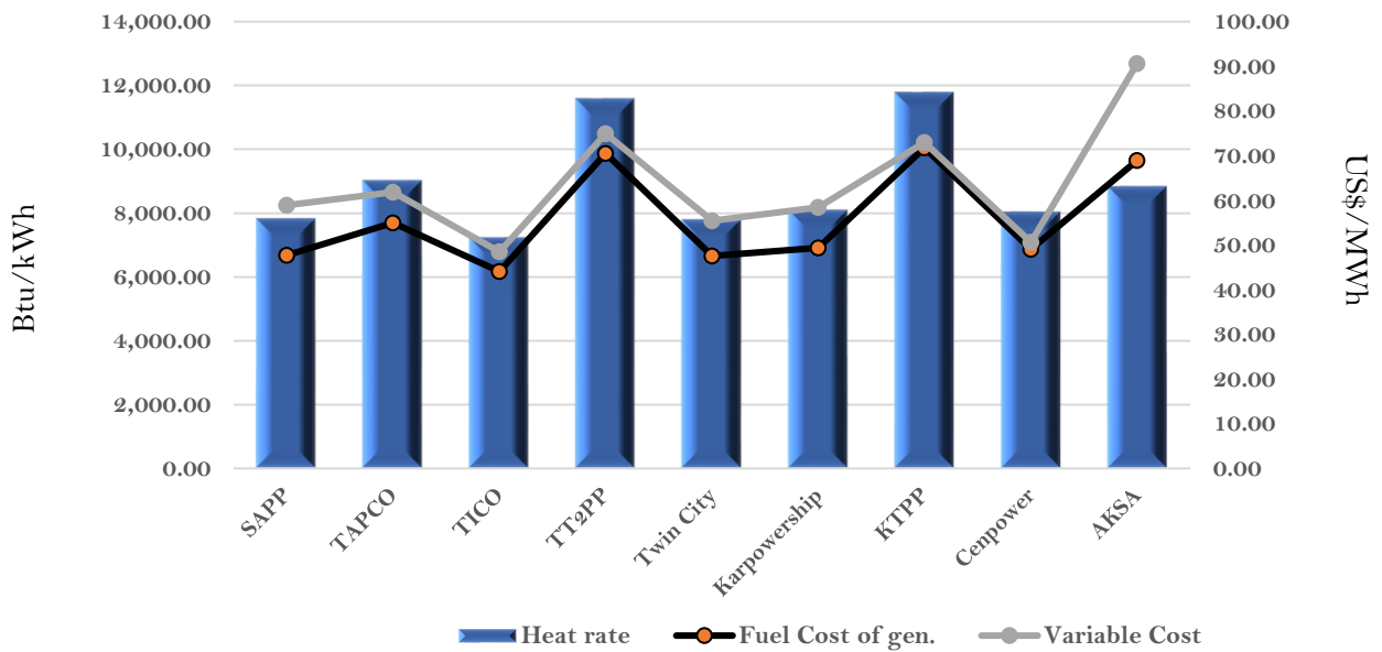
Efficiency and fuel cost of generation on the 24th May 2023
