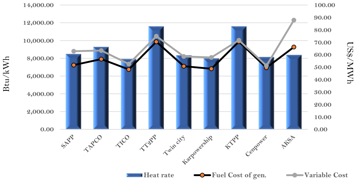
Efficiency and fuel cost of generation on the 30th May 2023
