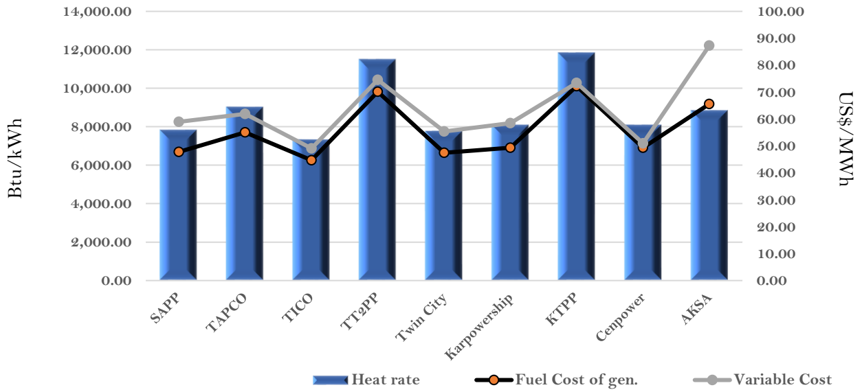
Efficiency and fuel cost of generation on the 23rd May 2023
