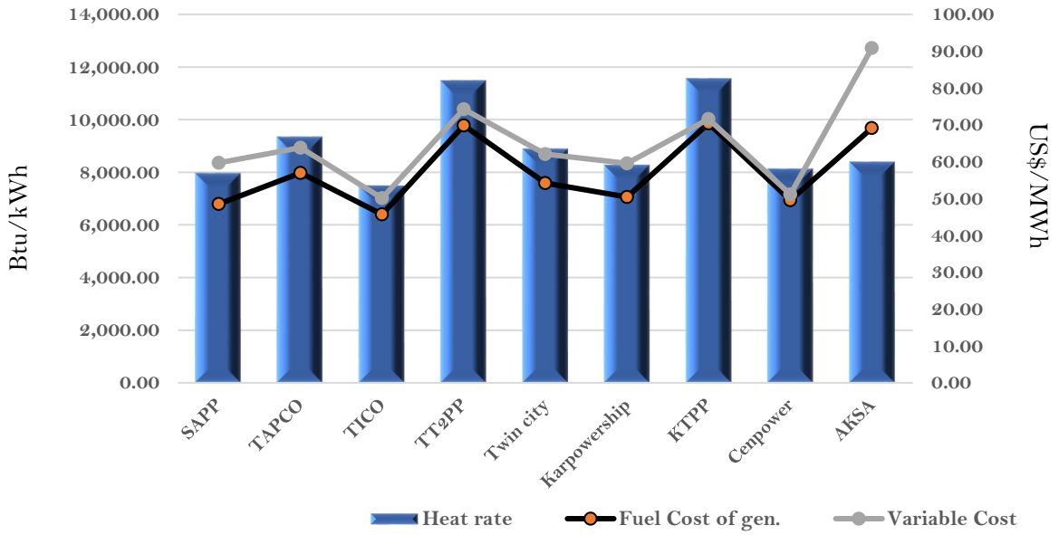
Efficiency and fuel cost of generation on the 29th May 2023
