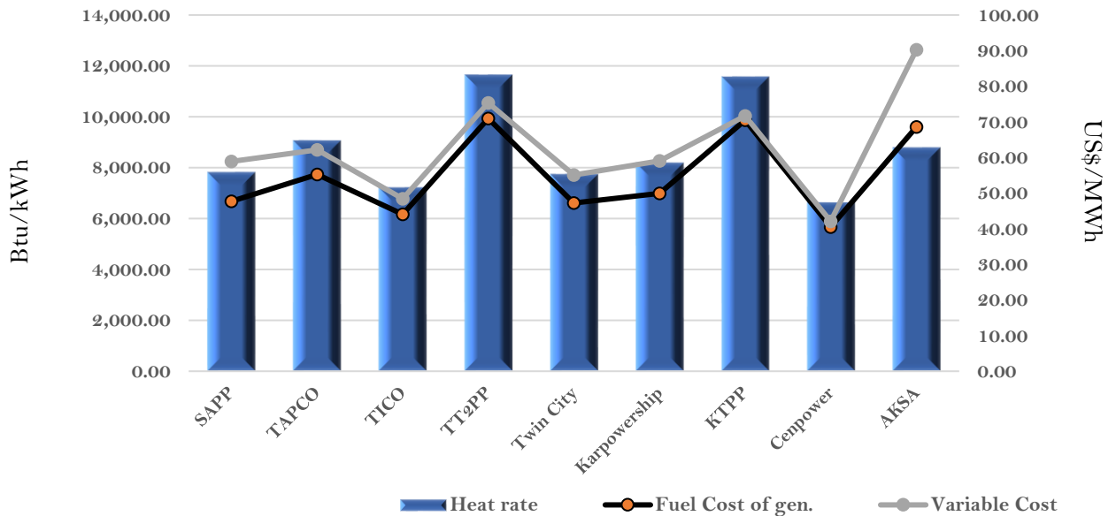
Efficiency and fuel cost of generation on the 26th May 2023
