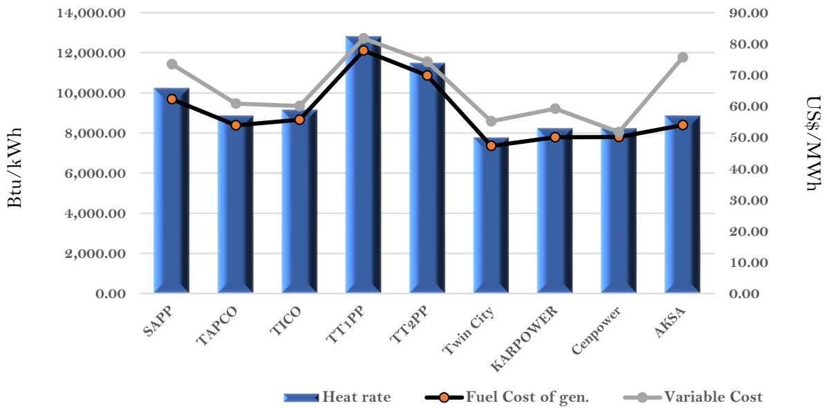
Efficiency and fuel cost of generation on the 11th June 2023
