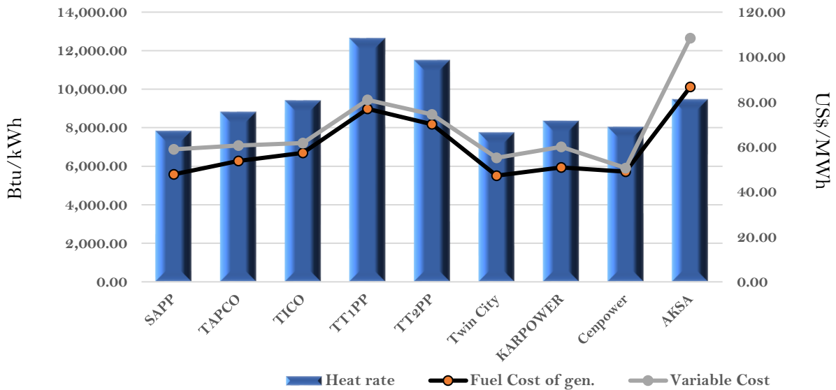
Efficiency and fuel cost of generation on the 12th June 2023
