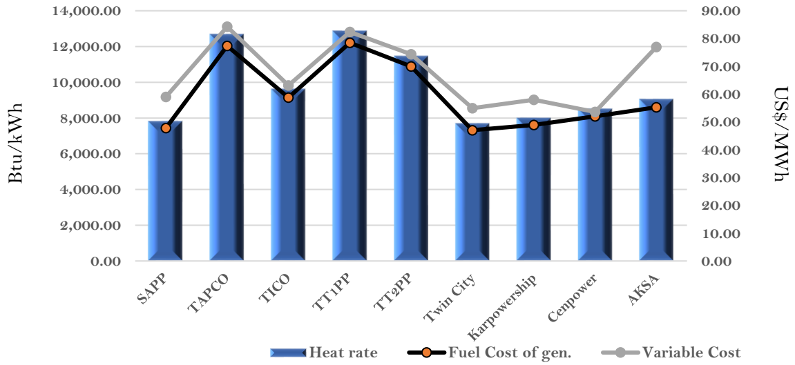
Efficiency and fuel cost of generation on the 20th June 2023
