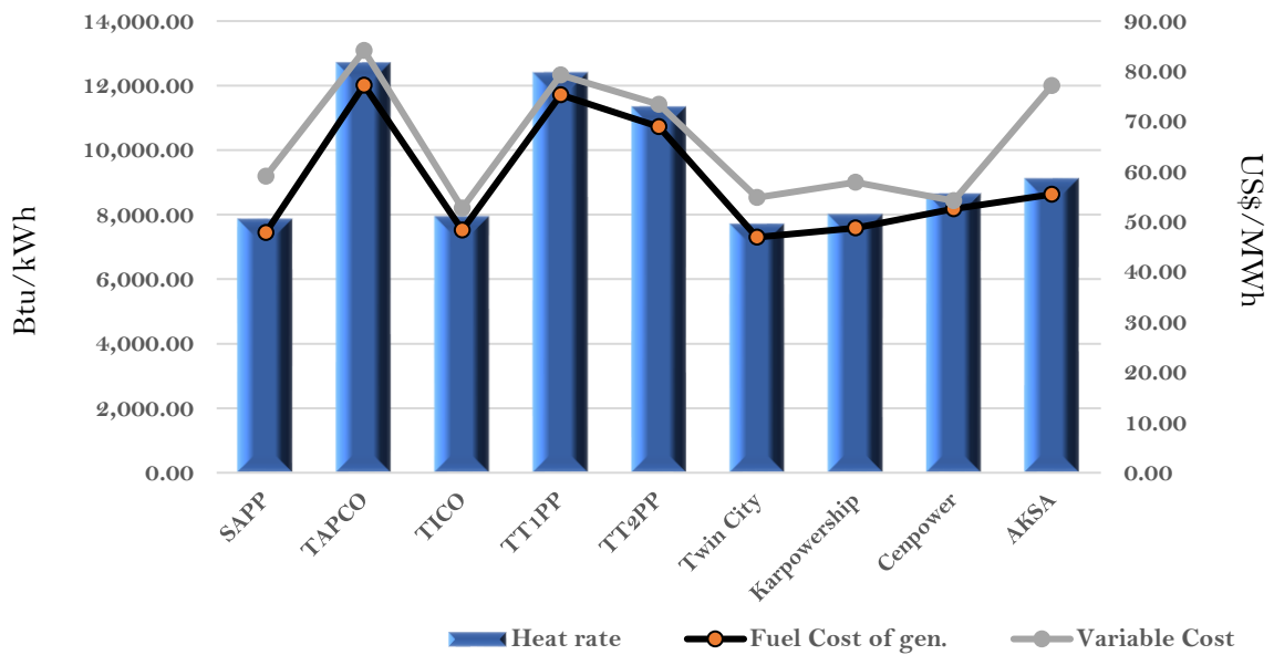
Efficiency and fuel cost of generation on the 21st June 2022
