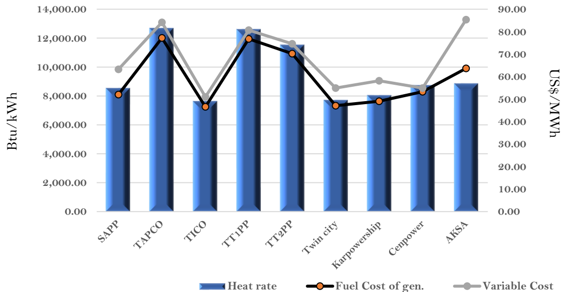
Efficiency and fuel cost of generation on the 30th June 2023
