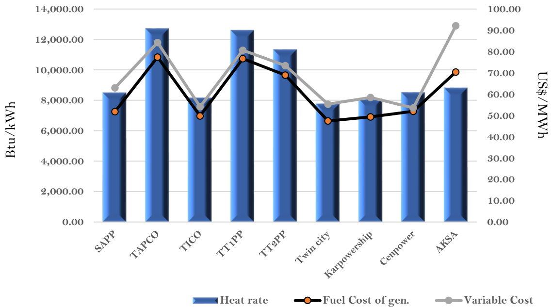
Efficiency and fuel cost of generation on the 29th June 2023
