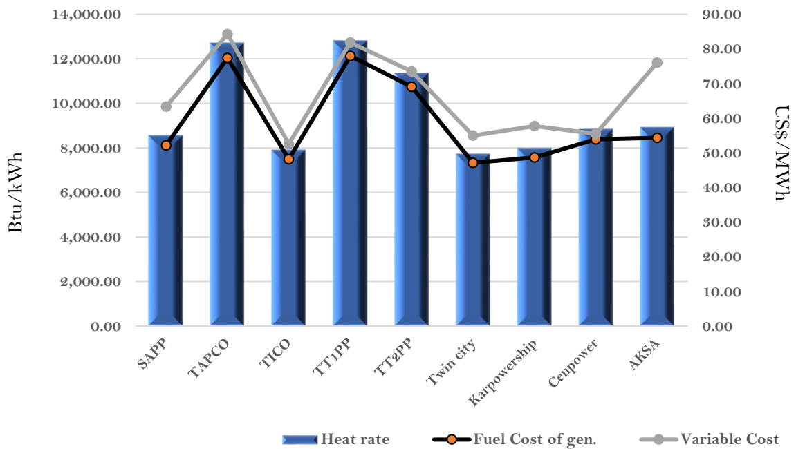
Efficiency and fuel cost of generation on the 28th June 2023
