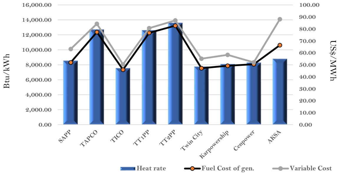
Efficiency and fuel cost of generation on the 27th June 2023
