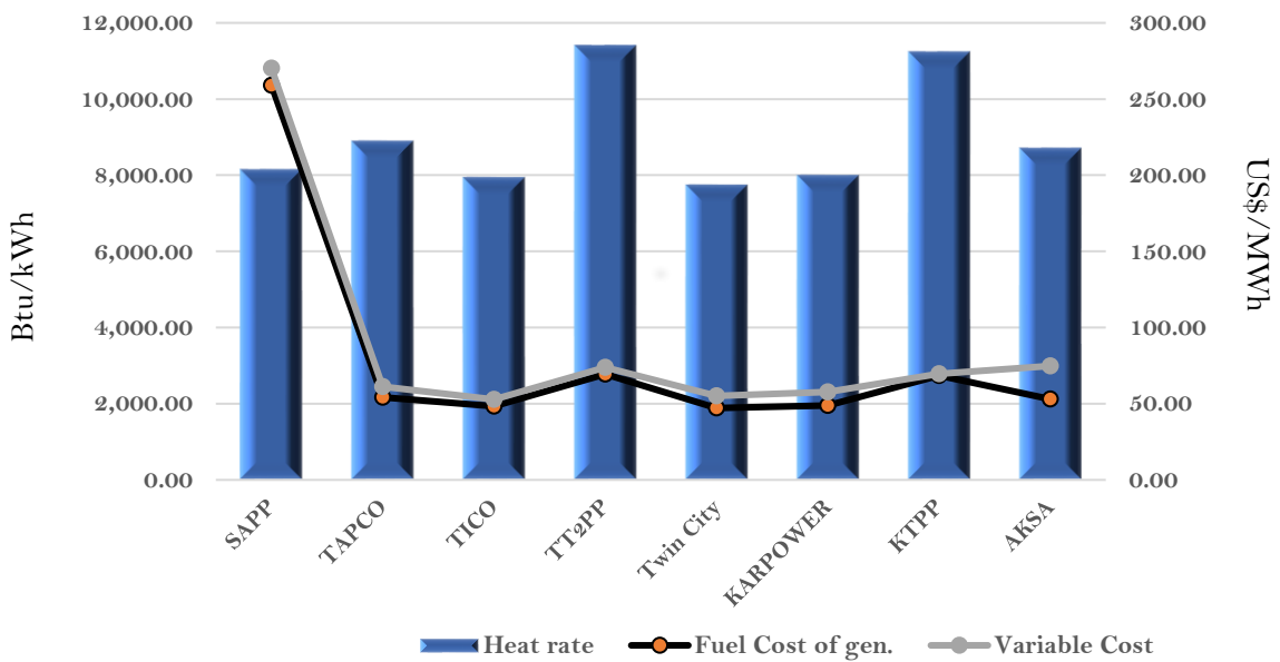
Efficiency and fuel cost of generation on the 14th July 2023
