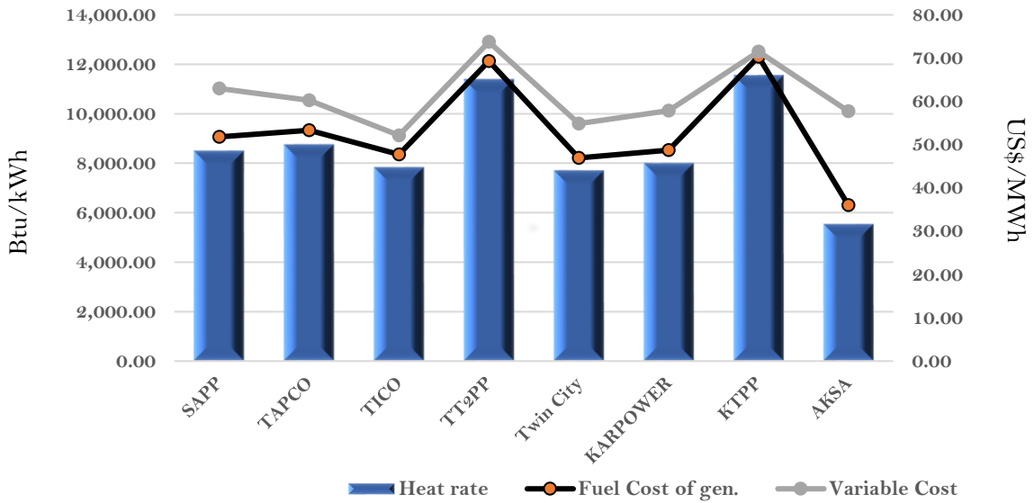
Efficiency and fuel cost of generation on the 13th July 2023
