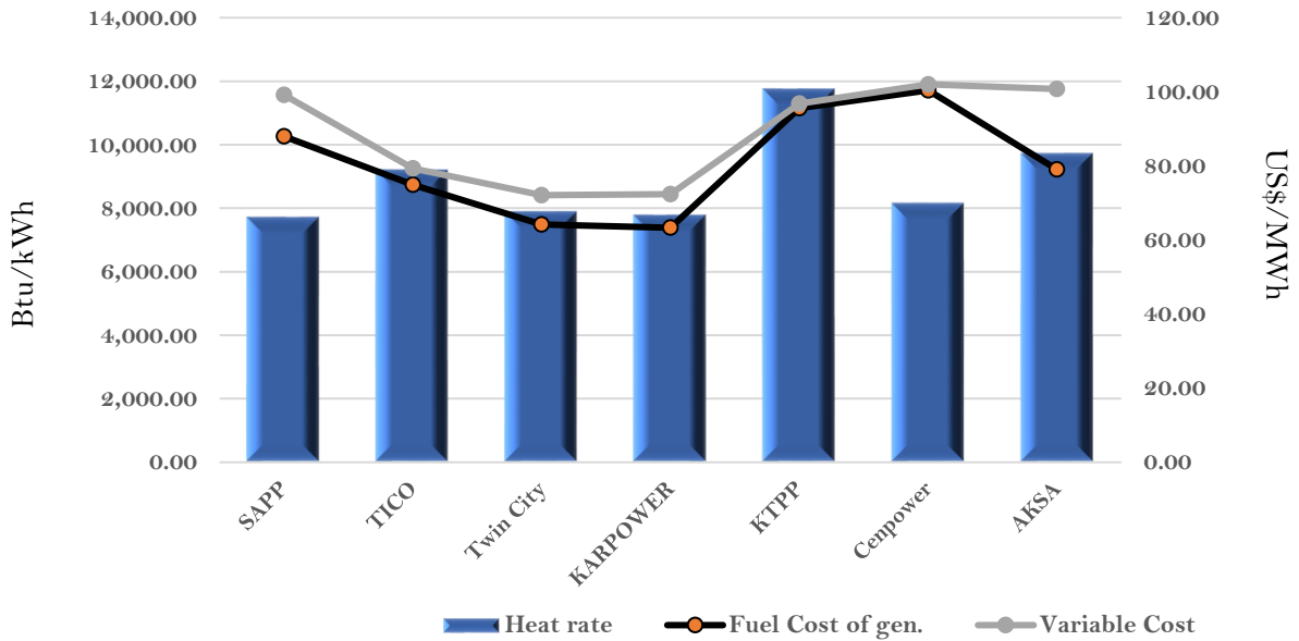
Efficiency and fuel cost of generation on the 12th September 2023
