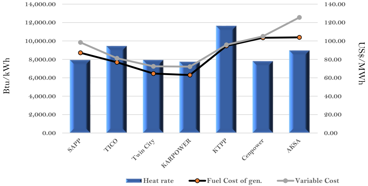
Efficiency and fuel cost of generation on the 11th September 2023
