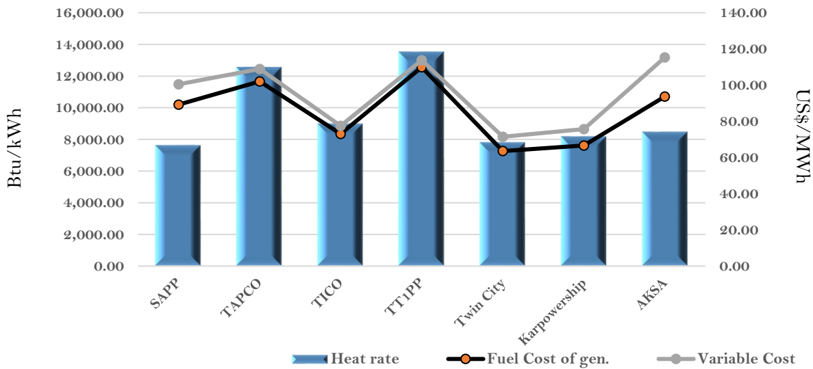
Efficiency and fuel cost of generation on the 28th September 2023
