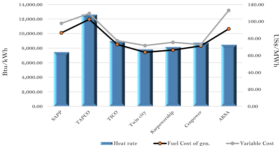
Efficiency and fuel cost of generation on the 28th September 2023
