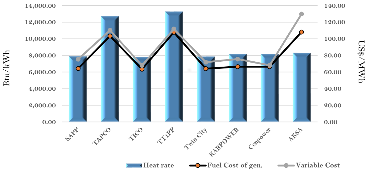
Efficiency and fuel cost of generation on the 4th October 2023
