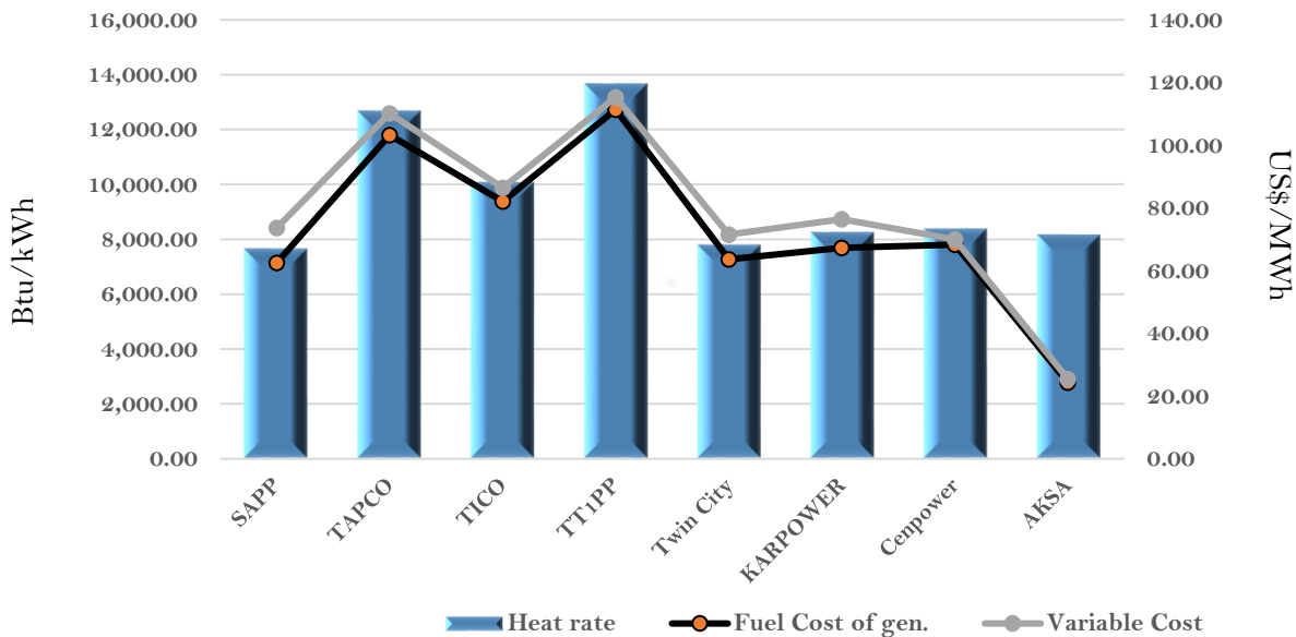
Efficiency and fuel cost of generation on the 5th October 2023
